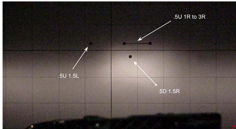
FIGURE 11 - TEST POINTS FOR THE 9007 REFERENCE REFLECTOR
