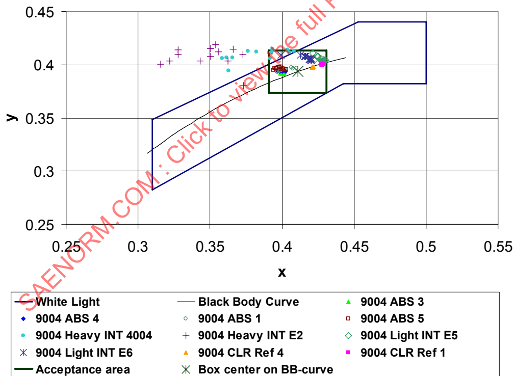
FIGURE 13A - DETAIL OF CIE 1931 CHROMATICITY DIAGRAM SHOWING CHROMATICITY DISTRIBUTIONS FROM THE BULB COLOR SEPARATION TEST FOR THE 9004 BULBS TESTED
