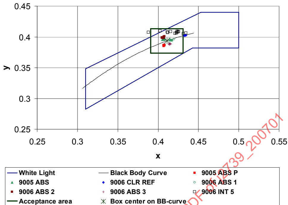
FIGURE 13B - DETAIL OF CIE 1931 CHROMATICITY DIAGRAM SHOWING CHROMATICITY DISTRIBUTIONS FROM THE BULB COLOR SEPARATION TEST FOR THE 9005 AND 9006 BULBS TESTED; THE ACCEPTANCE AREA SHOWN IS FOR THE EVALUATION OF BULB "9006 INT 5"
