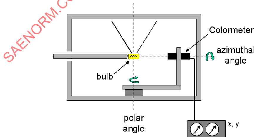
FIGURE 17 - PRINCIPLE OF THE COLOR SEPARATION TEST; THE SPATIAL CHROMATICITY DISTRIBUTION WITHIN A WELL-DEFINED ANGULAR REGION AROUND THE BULB IS DETERMINED WITH A ROTATING AND TILTING COLORIMETER
