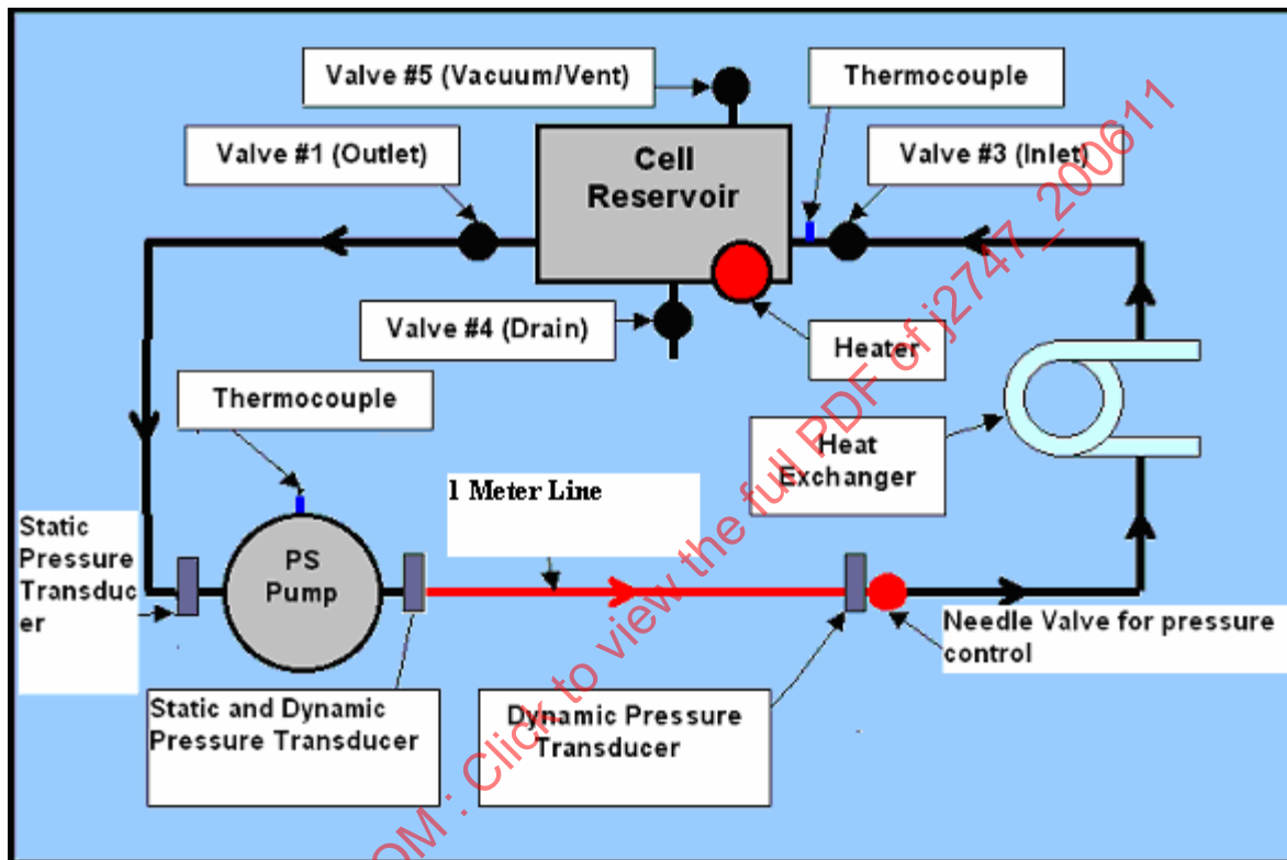
FIGURE 4 - HYDRAULIC CIRCUIT SETUP
