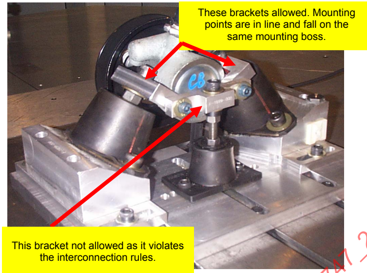
FIGURE 2 - PUMP MOUNTING AND ISOLATOR LOCATION
