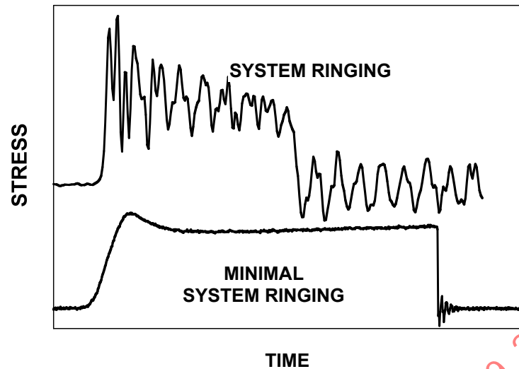
FIGURE A2 - TEST RUNS WITH AND WITHOUT SYSTEM RINGING
