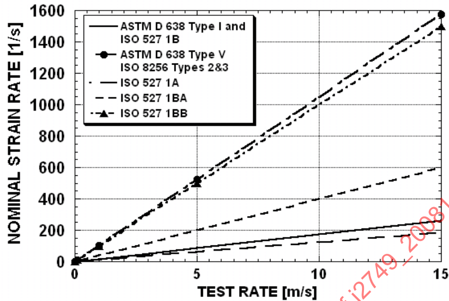
FIGURE A1 - RELATIONSHIP BETWEEN TEST RATE AND NOMINAL PLASTIC STRAIN RATE FOR DIFFERENT SPECIMEN CONFIGURATIONS
