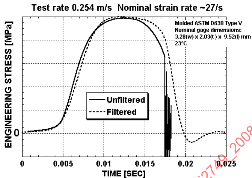
FIGURE A5 - EFFECTS OF A SLOW MEASUREMENT FREQUENCY RESPONSE WITH A LOW PASS FILTER ON THE RECORDED STRESS SIGNAL
