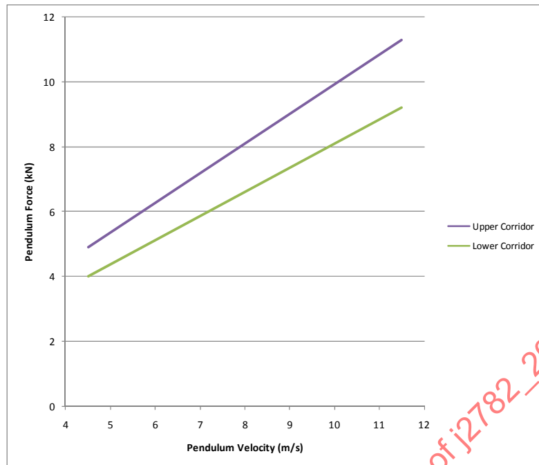
FIGURE 13 - FORCE VERSUS VELOCITY LATERAL PELVIS CORRIDOR
