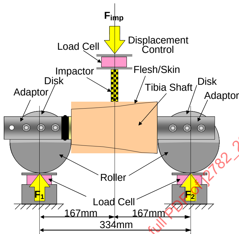
FIGURE 21 - LEG EXAMPLE TEST SET-UP
