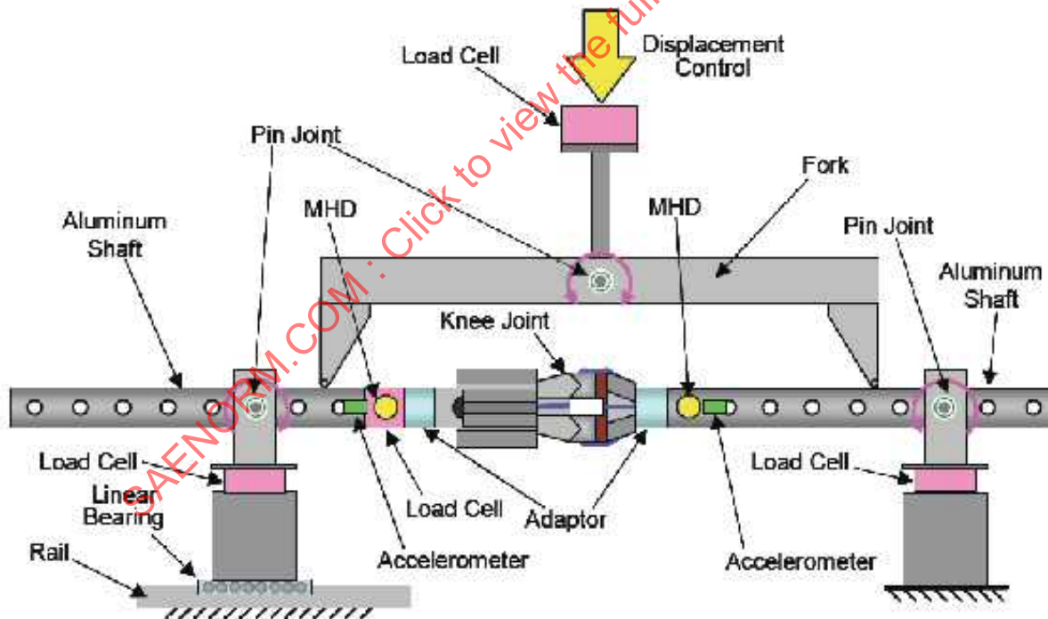
FIGURE 19 - KNEE EXAMPLE TEST SET-UP
