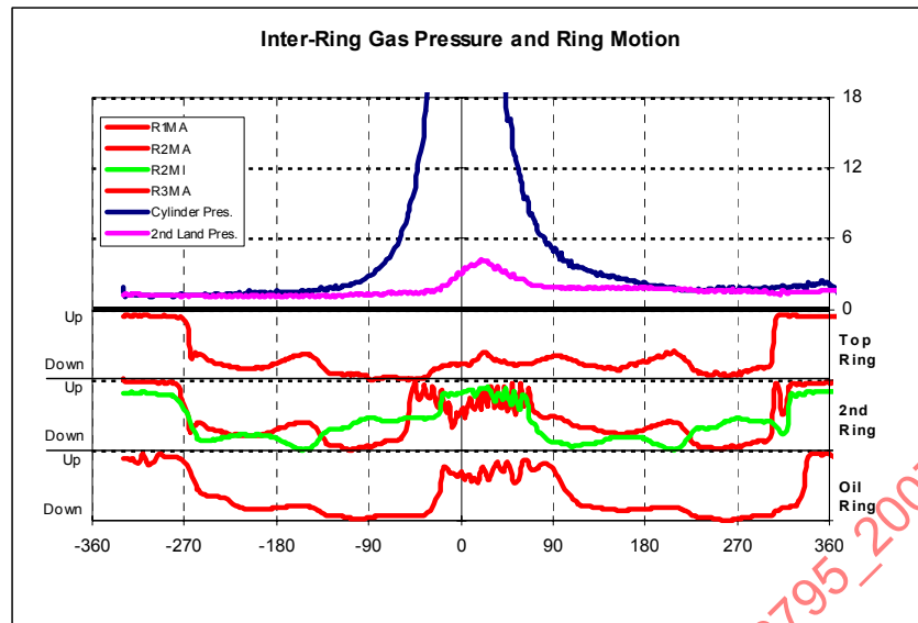
FIGURE 9 - EXAMPLE OF INTER-RING GAS PRESSURE AND RING MOTION
