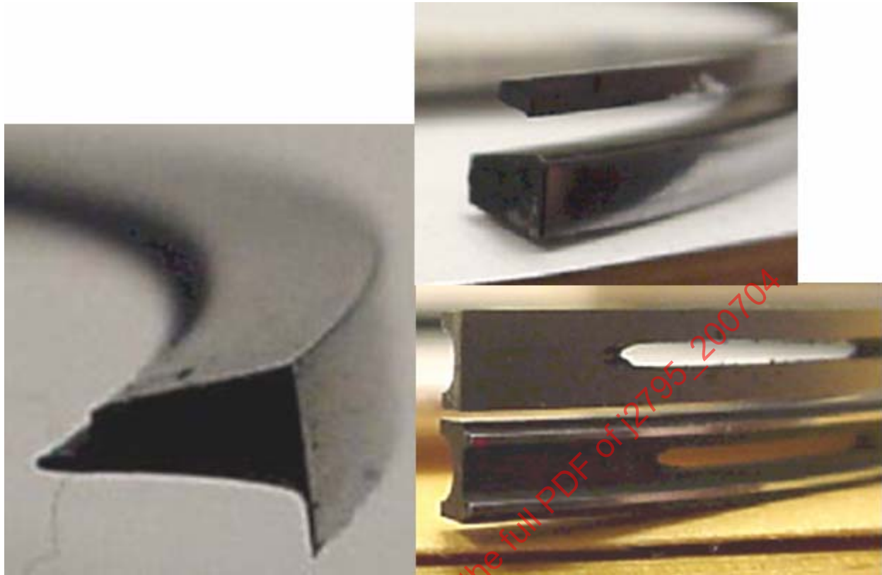
FIGURE 7 - EXAMPLES OF EXCESSIVELY WORN RINGS
