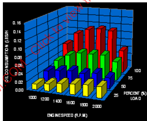
FIGURE 10 - EXAMPLE OF OIL CONSUMPTION MAPPING
