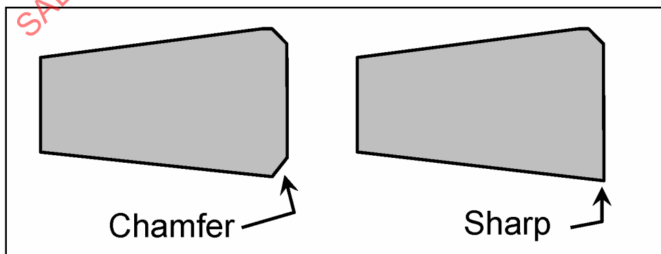
FIGURE 24 - SCHEMATICS OF BOTTOM SIDE OD CHAMFERS
