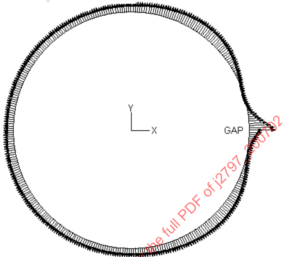
FIGURE 19 - EXAMPLE OF CALCULATED RING PRESSURE PATTERN
