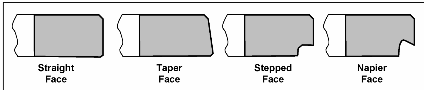
FIGURE 22 - SECOND RING FACE PROFILES
