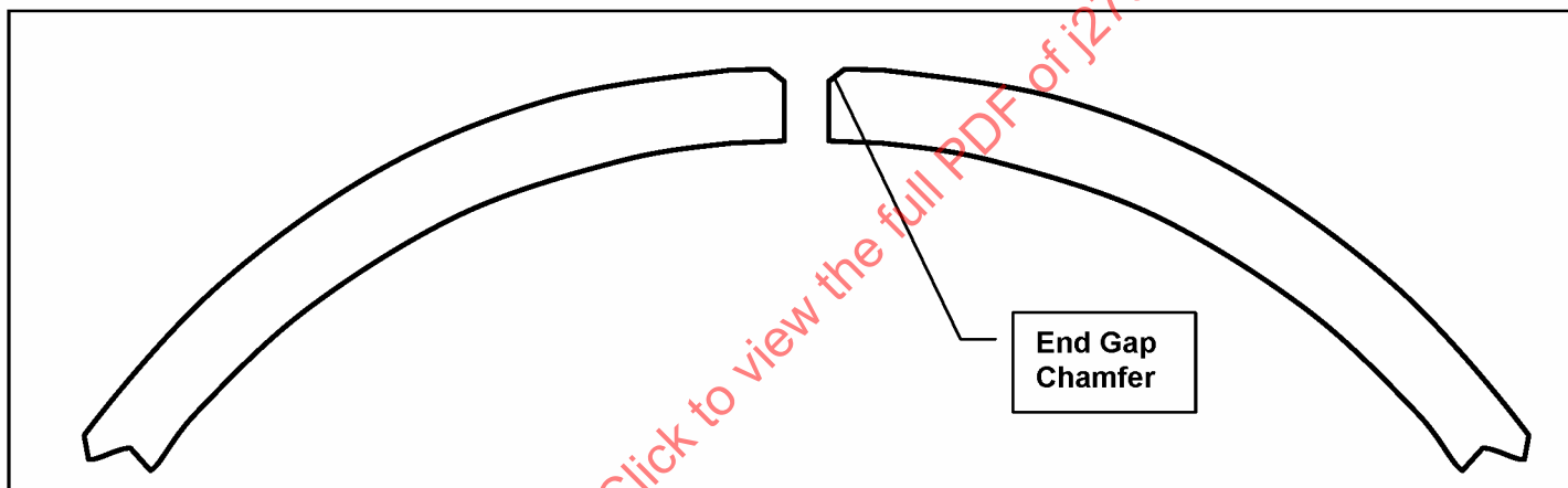
FIGURE 23 - END GAP CHAMFER
