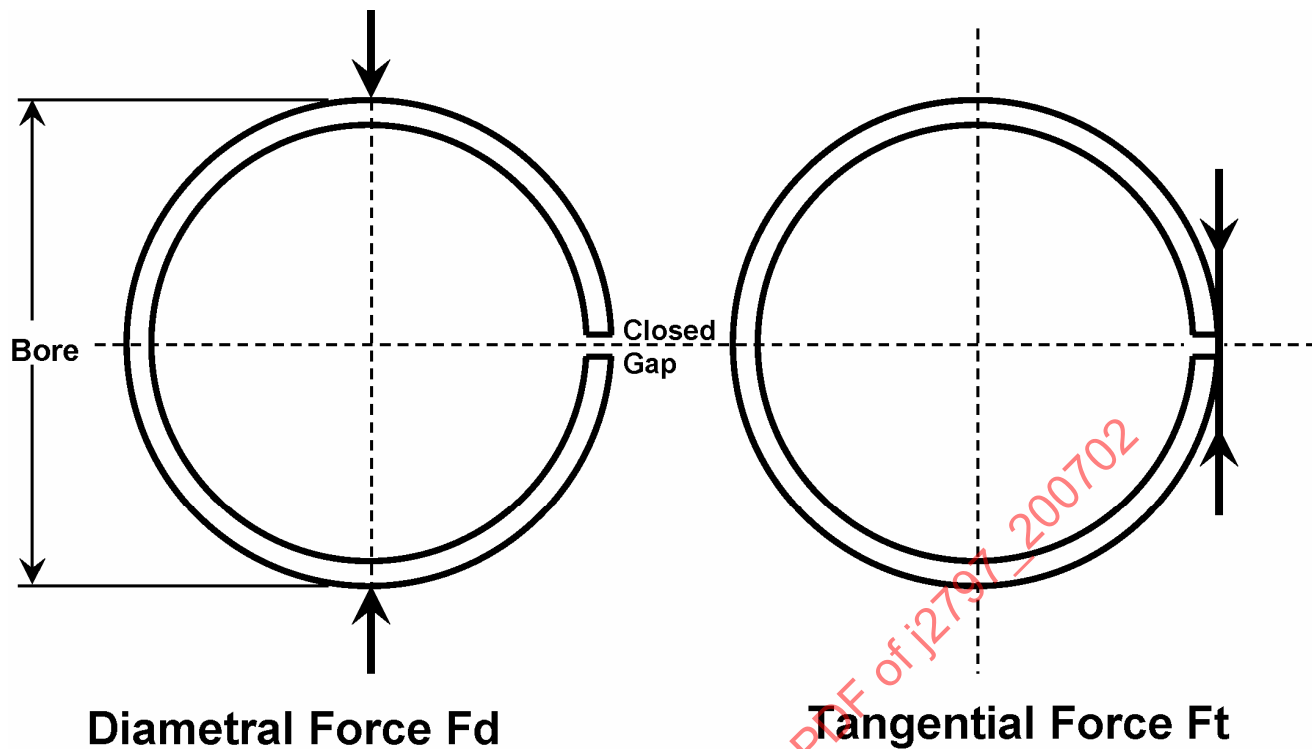
FIGURE 20 - ILLUSTRATION OF RING TENSION MEASUREMENTS
