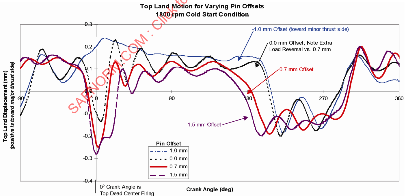
FIGURE 14 - EXAMPLE OF THE EFFECT OF PIN OFFSET ON PISTON MOTION
