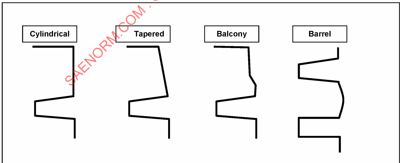
FIGURE 9 - LAND PROFILES
