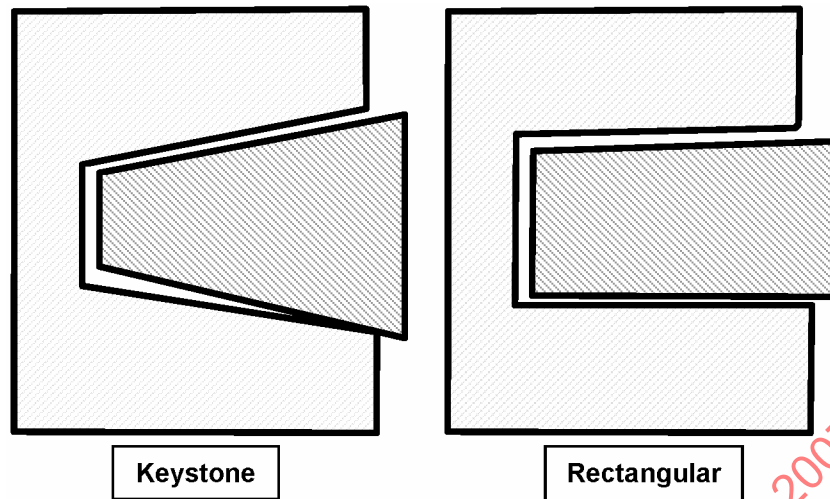
FIGURE 4 - TYPES OF RINGS AND GROOVES
