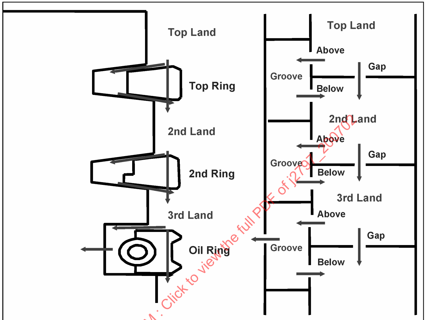
FIGURE 3 - RING PACK - ORIFICE/VOLUME MODEL
