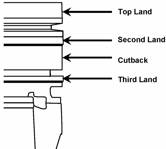
FIGURE 8 - LAND DIAMETERS
