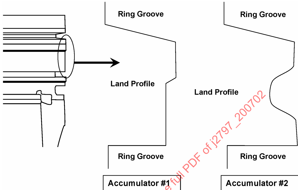
FIGURE 11 - LAND ACCUMULATOR GROOVES
