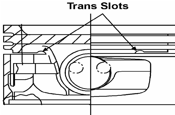
FIGURE 13 - OIL DRAIN TRANS SLOTS
