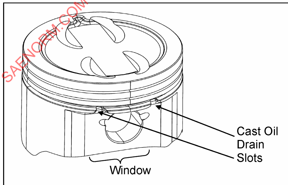
FIGURE 12 - OIL DRAIN SLOTS
