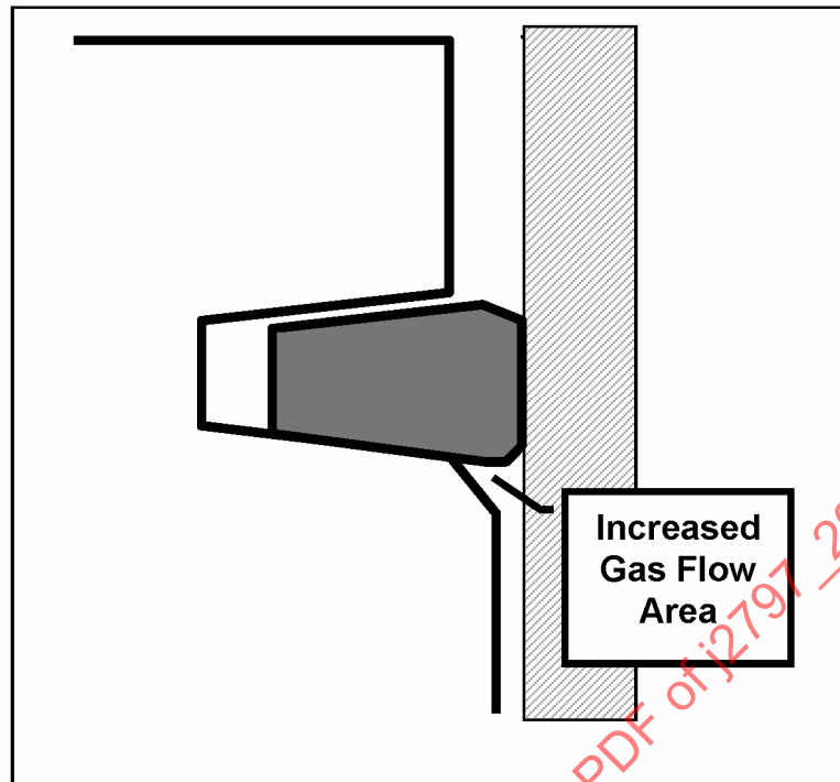
FIGURE 7 - EFFECT OF THE LARGE OUTSIDE DIAMETER EDGE BREAK
