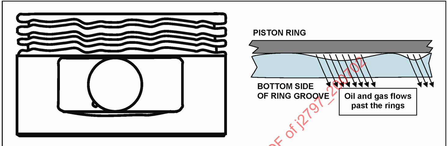
FIGURE 6 - GROOVE WAVINESS
