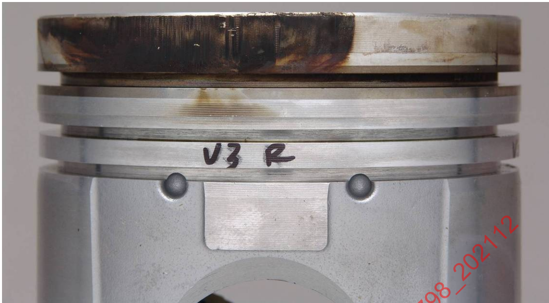
Figure 6 - Example of carbon tracking caused by excessive bore distortion
