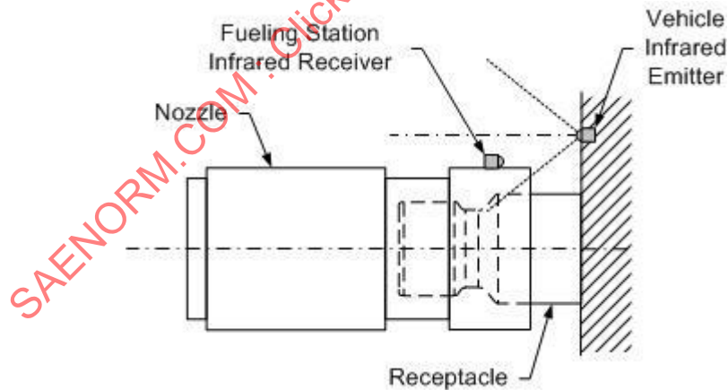
FIGURE 2 - CONNECTOR WITH INFRARED COMMUNICATIONS LINK
