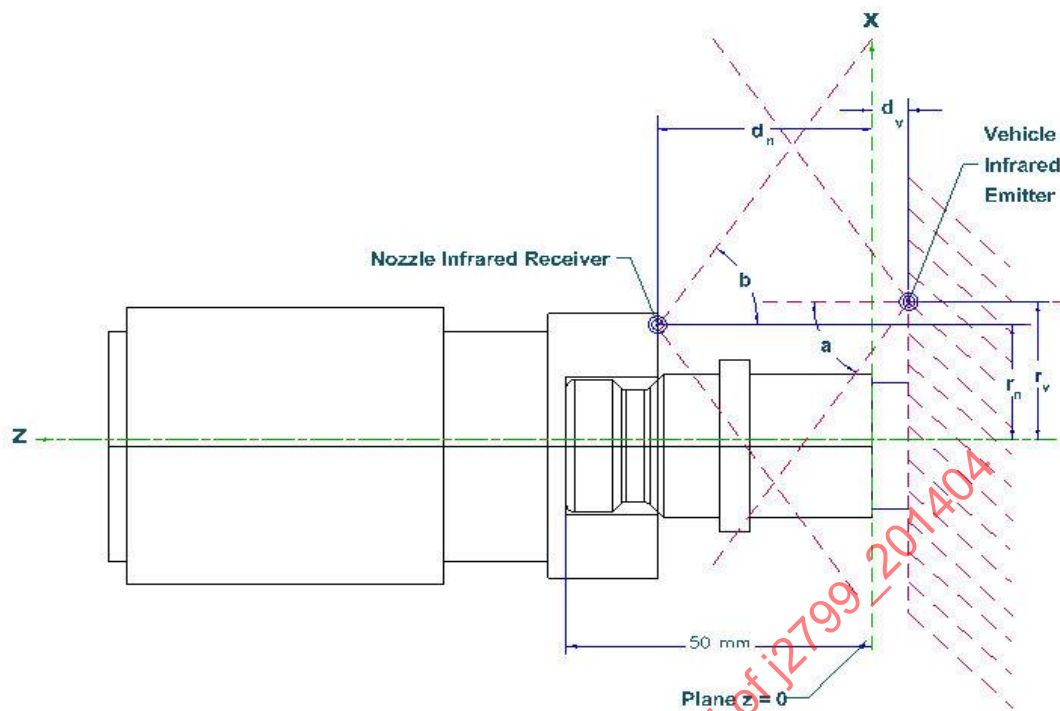
FIGURE 9 - VEHICLE RECEPTACLE (SIDE VIEW)
