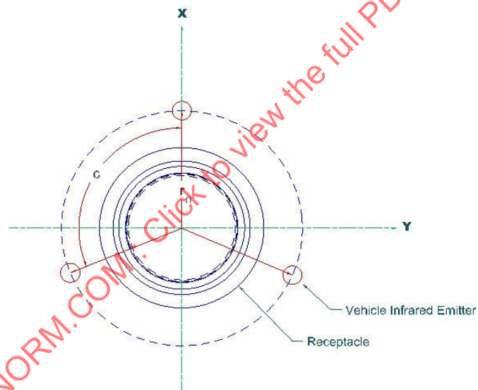
FIGURE 7 - VEHICLE TRANSMITTER (FRONT VIEW)
