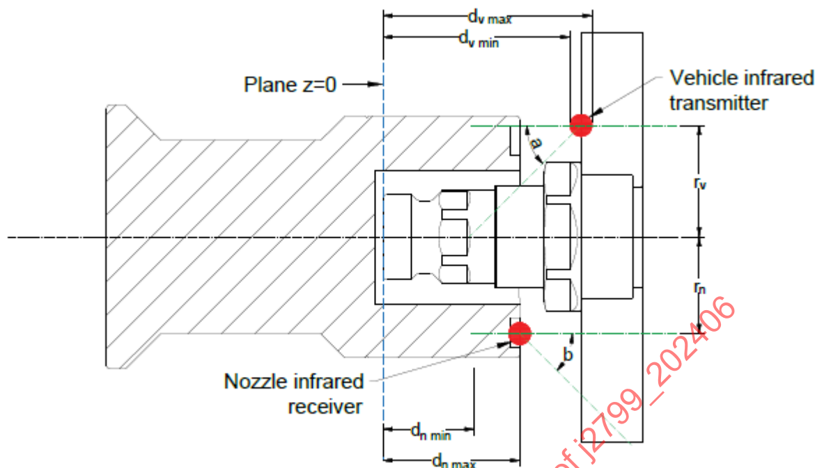
Figure 7 - Vehicle receptacle (side view)
