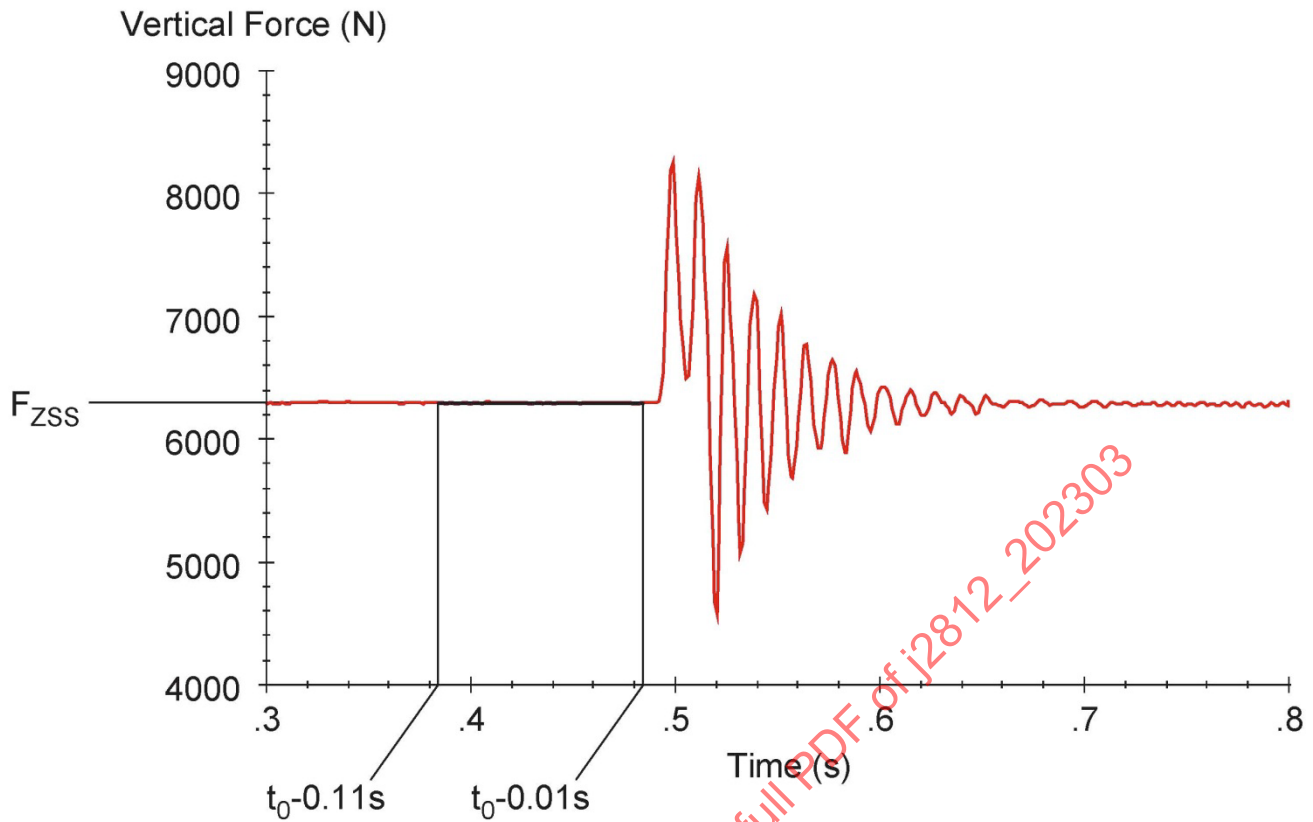
FIGURE 5 – STEADY-STATE OFFSET ELIMINATION - AVERAGING
