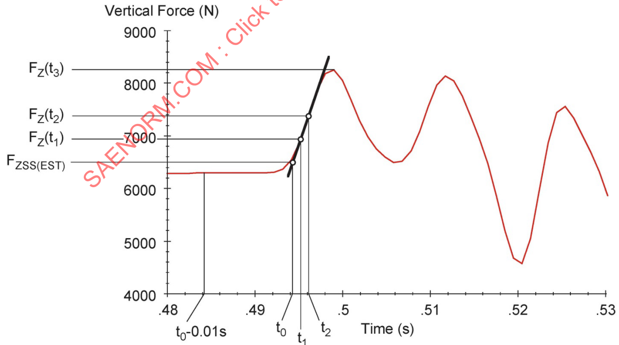
FIGURE 4 – STEADY-STATE OFFSET ELIMINATION – START OF DYNAMIC RESPONSE
