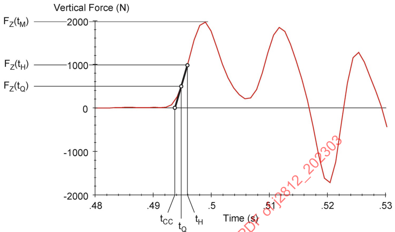
FIGURE 6 – TIME OF FIRST CLEAT CONTACT
