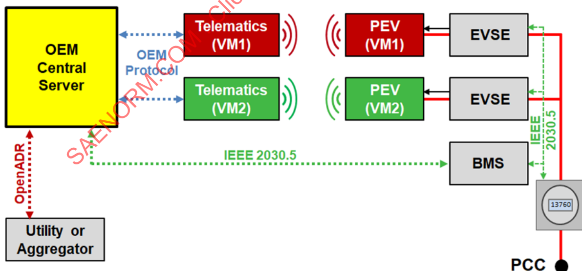
Figure 8 - OEM telematics
