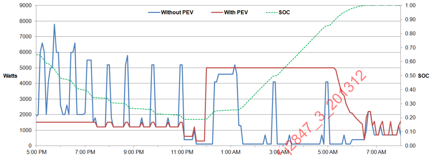
FIGURE B.1 - HOME ENERGY MANAGEMENT SIMULATION
