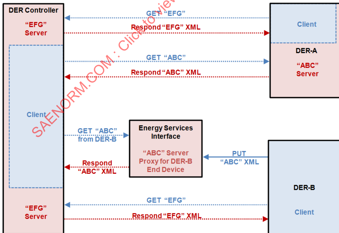
FIGURE 2 - DER DEVICE AS CLIENT OR SERVER
