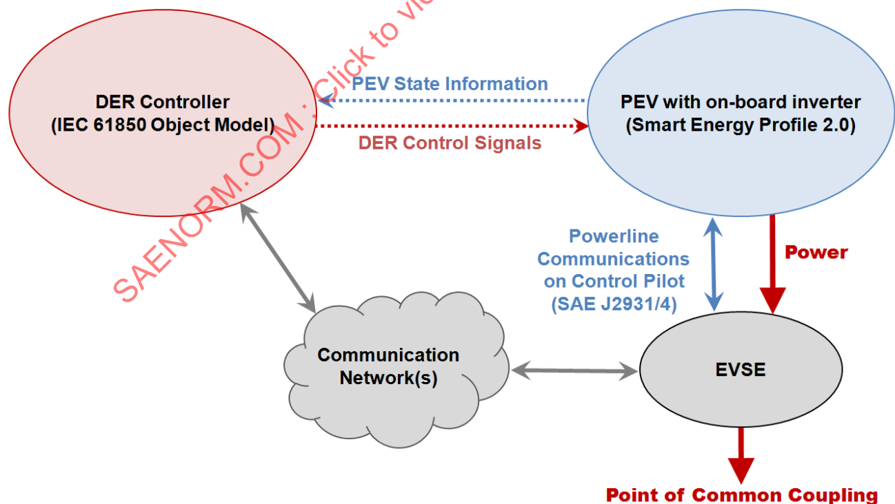
FIGURE 1 - BASIC SYSTEM ARCHITECTURE
