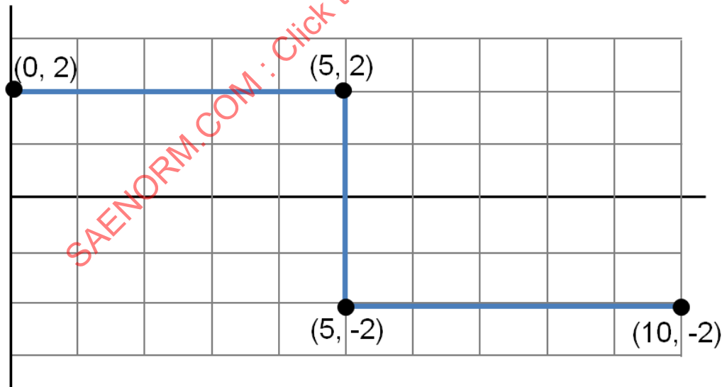
FIGURE 17 - DISCONTINUOUS FUNCTION
