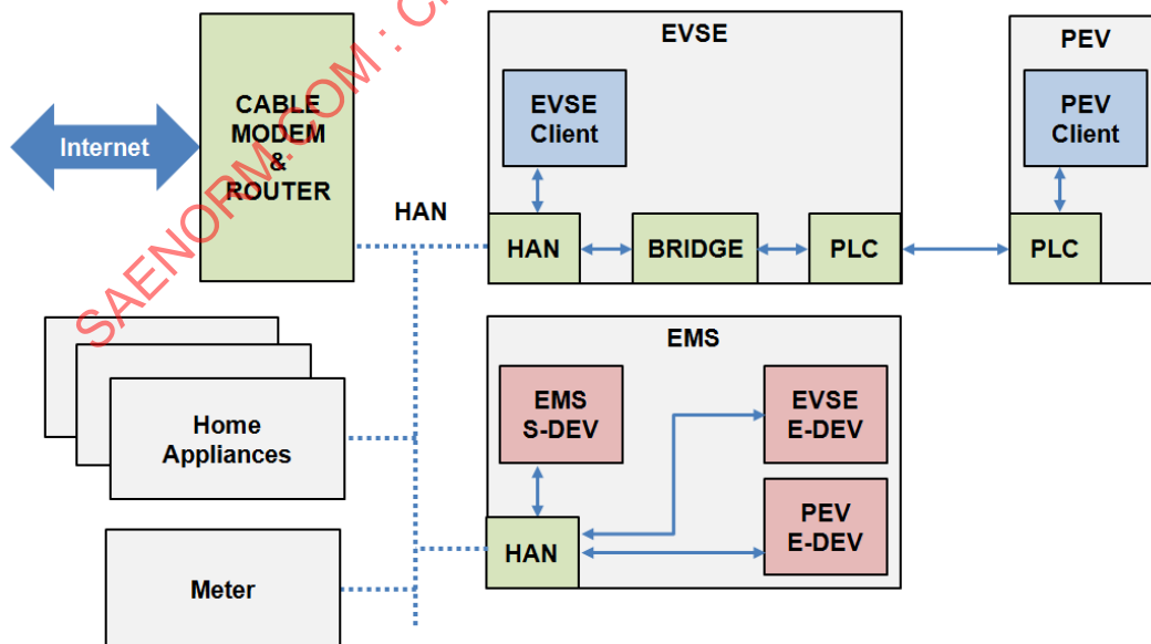
FIGURE B.2 – SYSTEM ARCHITECTURE FOR HOME ENERGY MANAGEMENT EXAMPLE
