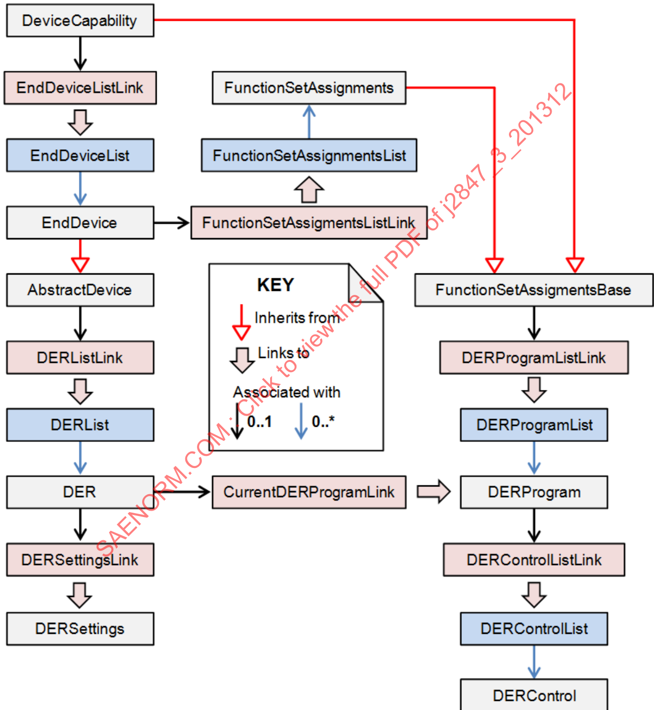
FIGURE 8 - CONNECTING RESOURCES
