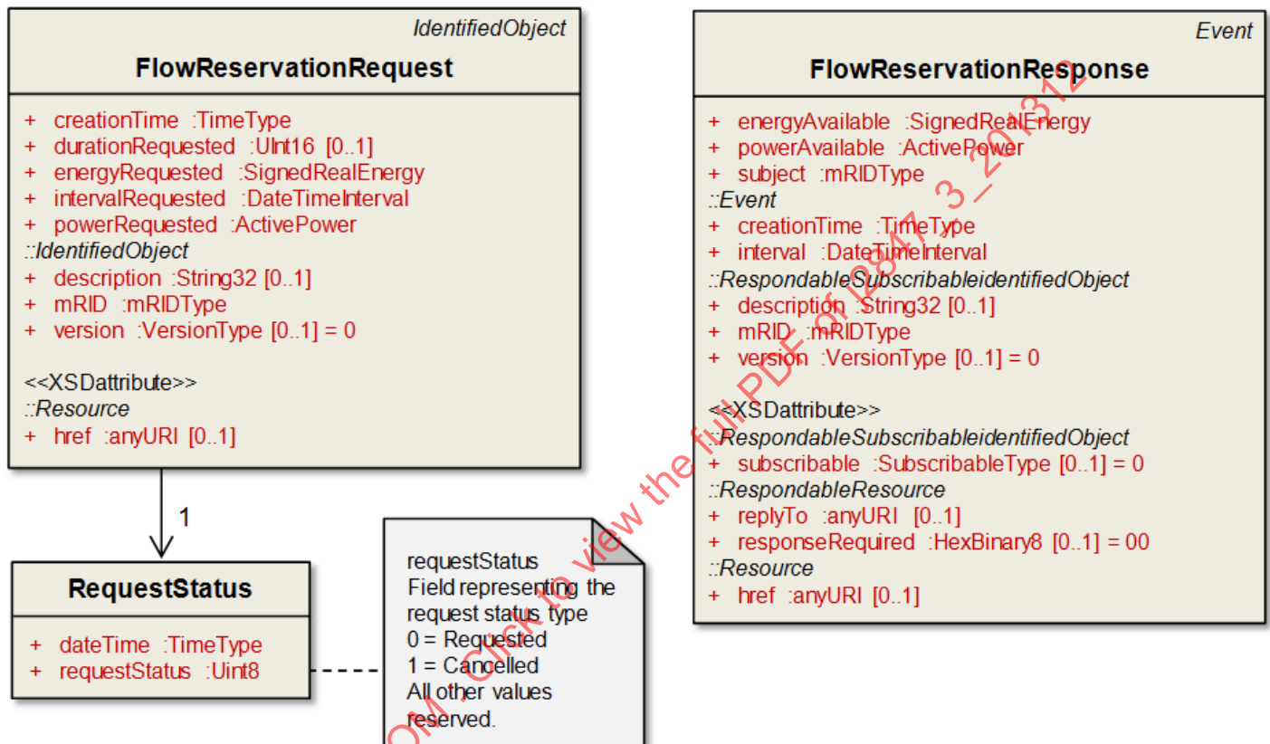
FIGURE 5- EXCERPTS FROM FLOW RESERVATION CLASS DIAGRAM
