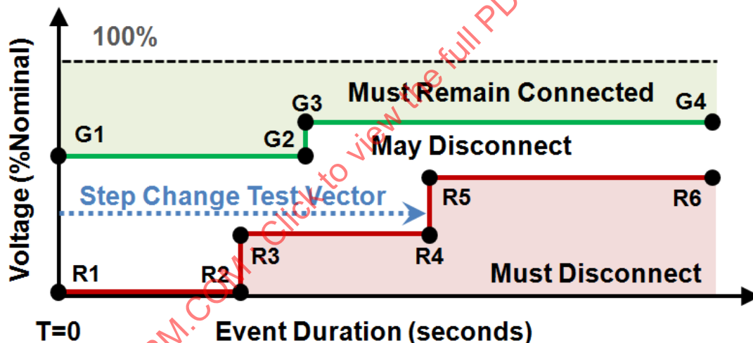
FIGURE 19 - LOW VOLTAGE RIDE THROUGH FUNCTION EXAMPLE
