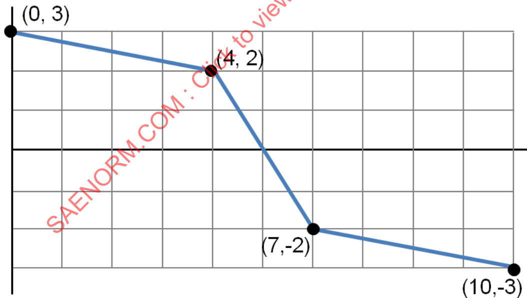
FIGURE 15 - NORMAL PIECEWISE LINEAR CURVE
