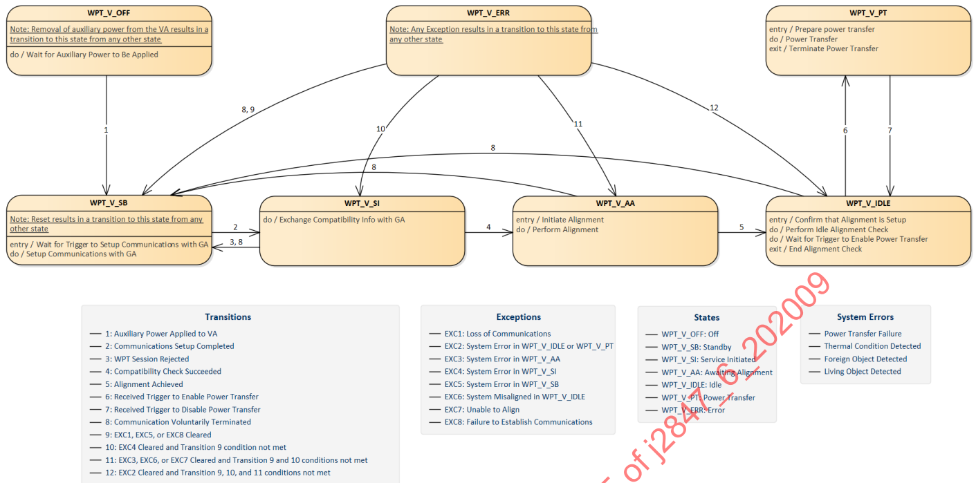
Figure 4 - VA system state diagram
