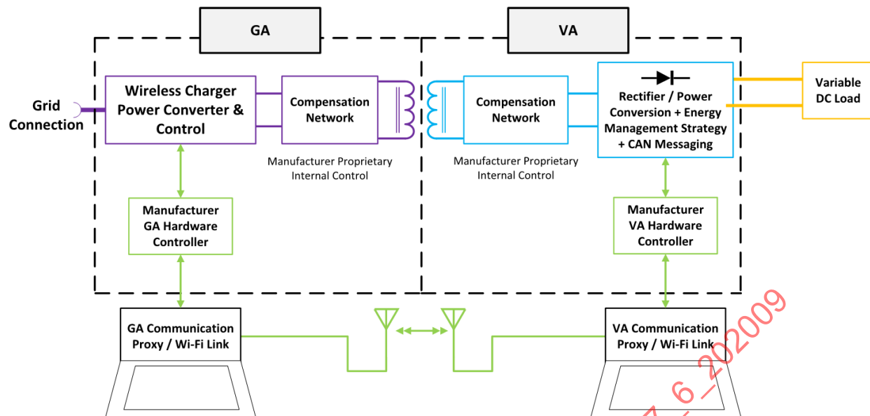
Figure 2 - GA and VA with SAE J2847/6 communication proxy for lab bench testing
