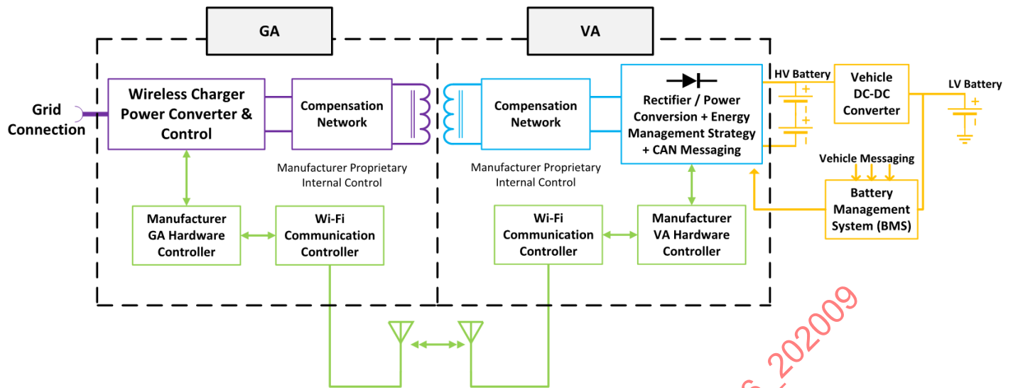
Figure 1 - Functional decomposition of a WPT system
