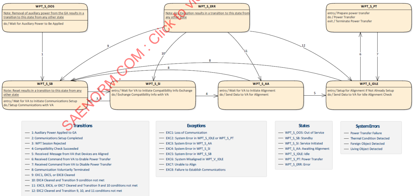
Figure 5 - GA system state diagram
