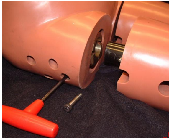
Figure 29 - Shoulder bolt connects thigh to the femur component
