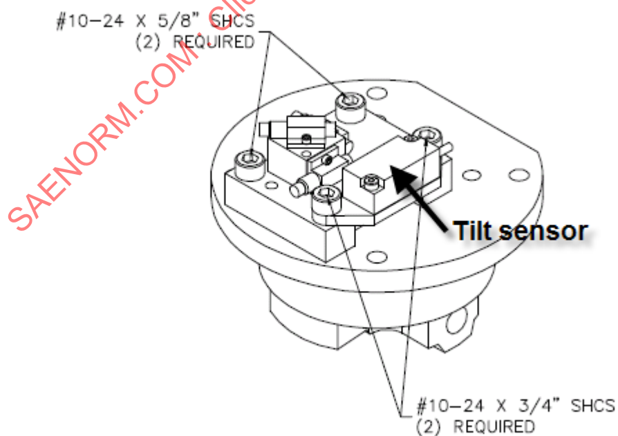
Figure 5 - Optional accelerometer block for the 10YO dummy head
