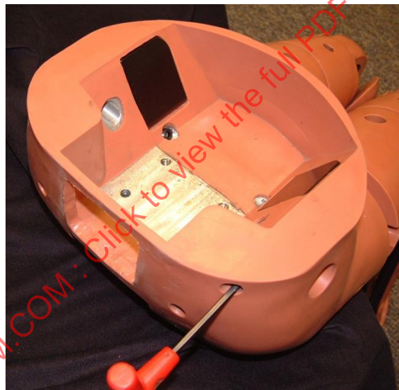
Figure 28 - Access for installing iliac load cells
