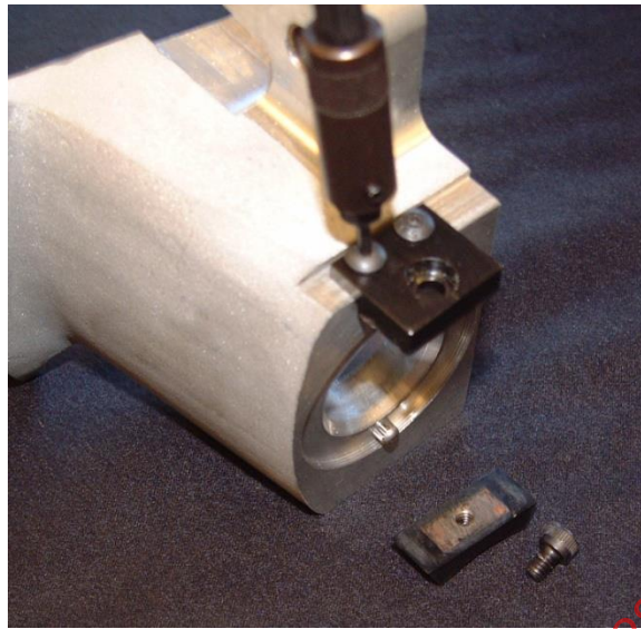
Figure 19 - Removal of shoulder stop components
