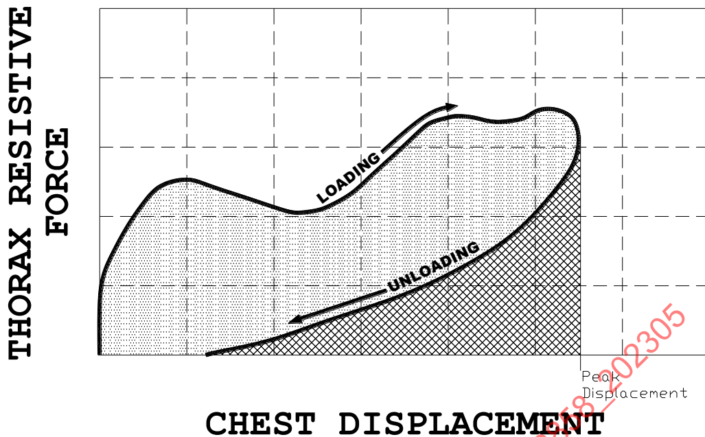
Figure 39 - Hysteresis calculation
