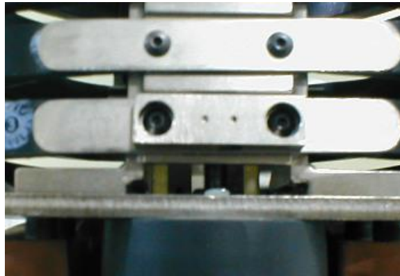
Figure 15 - Back rib stiffeners and posterior lower thorax accelerometer mount
