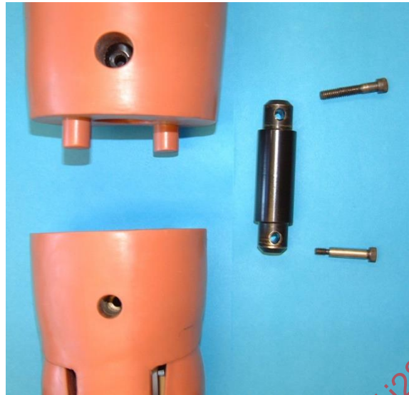
Figure 31 - The thigh and knee assembly are connected by the femur load cell replacement
