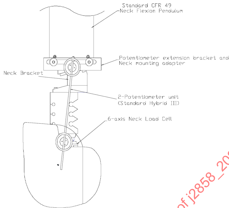
Figure 37 - Instrumentation setup for neck flexion test
