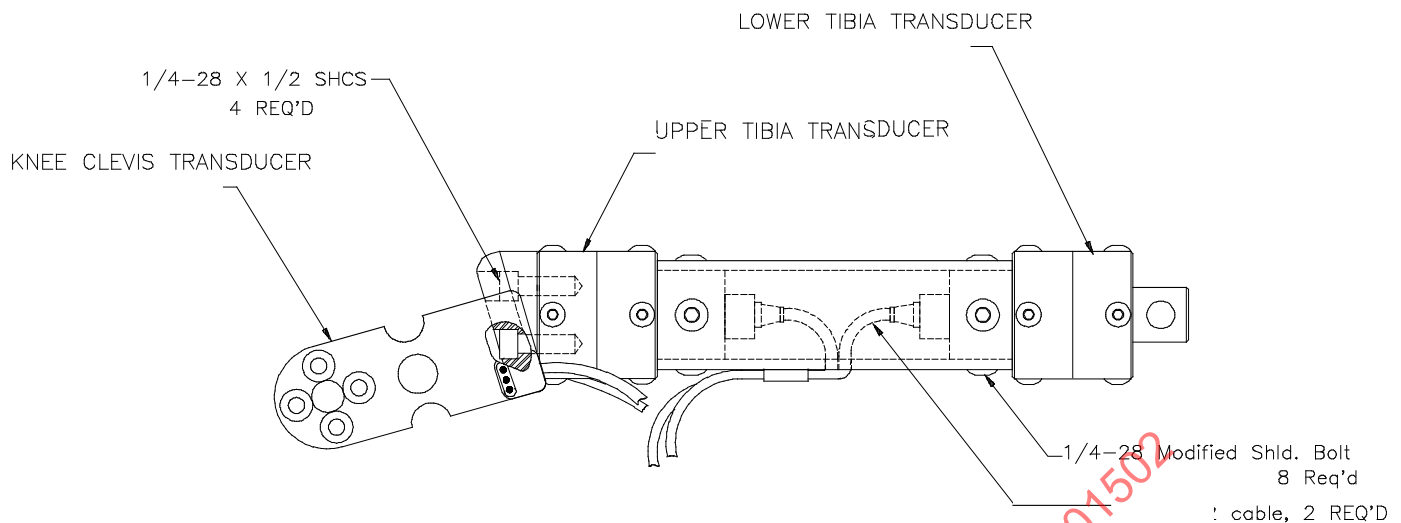
Figure 24 - Instrumented lower leg
