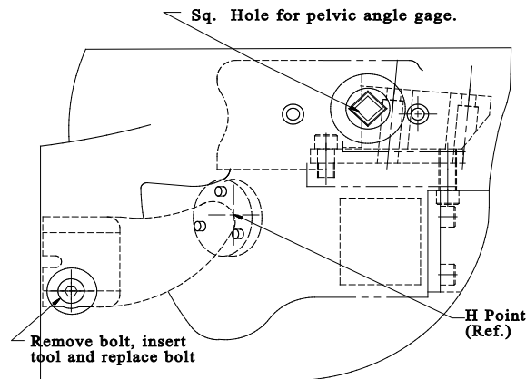
Figure 19 – “H” Point location
