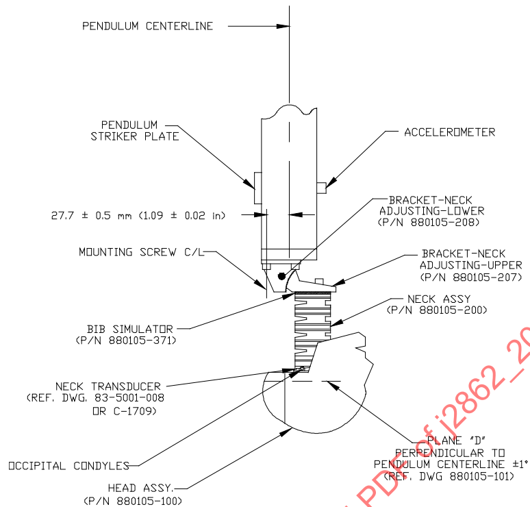
Figure 28 - Neck extension setup specifications
