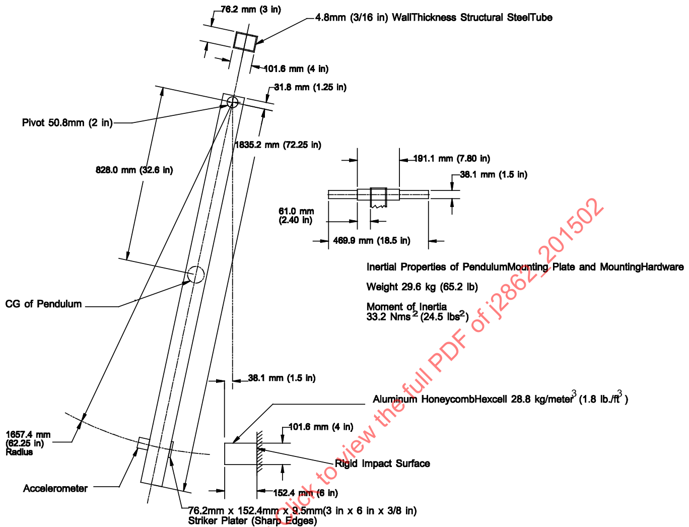
Figure 27 - Neck pendulum arm specifications
