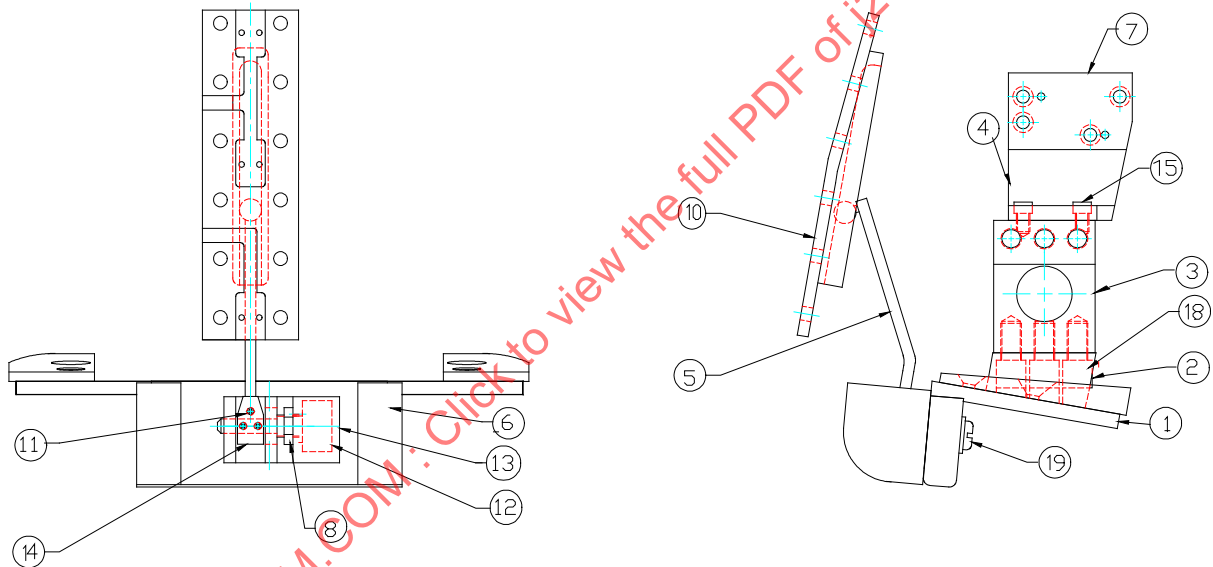
Figure 12 - Chest deflection assembly
