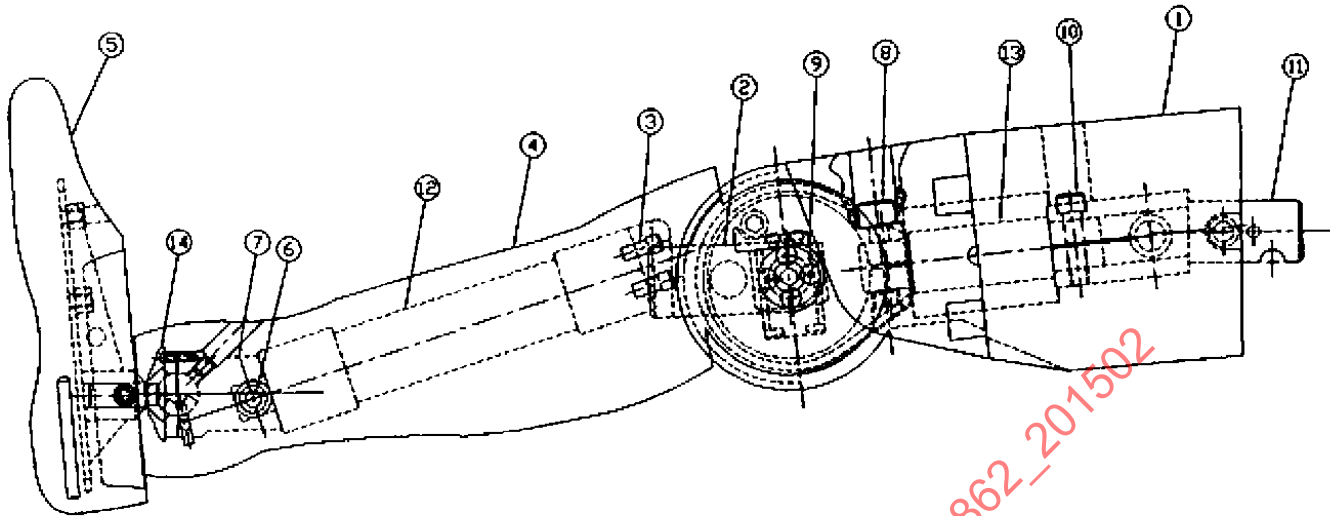
Figure 22 - Leg assembly
