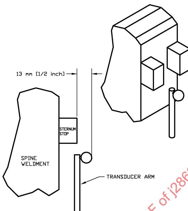
Figure 13 - Transducer arm clearance check
