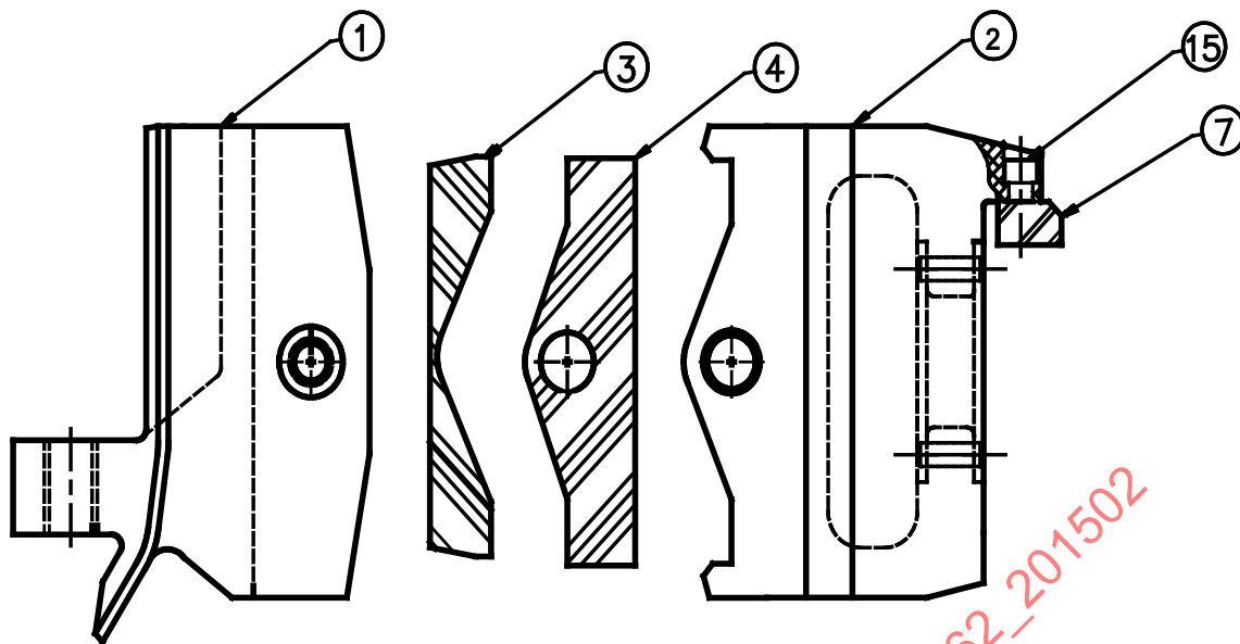
Figure 14 - Clavicle assembly
