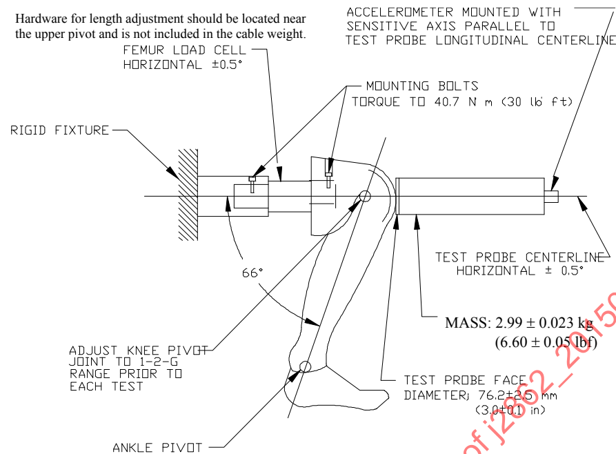
Figure 32 - Knee impact test setup specifications
