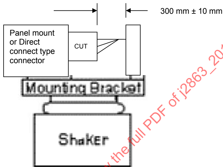
FIGURE 5 - VIBRATION TESTING MOUNTING POSITION
