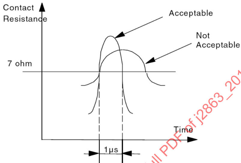
FIGURE 3 - INTERMITTENCY MEASUREMENT
