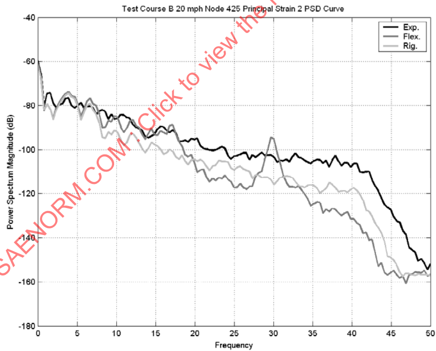
FIGURE 132 - NODE 425 PSD COMPARISON BETWEEN RIGID, FLEXIBLE, AND EXPERIMENT FOR TEST COURSE B
