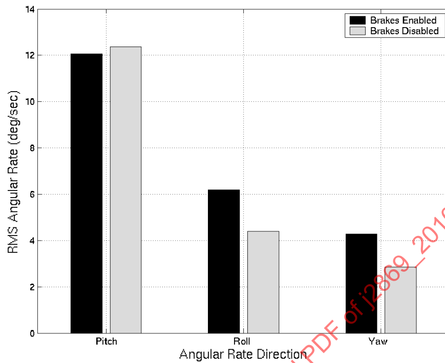
FIGURE C20 - RATE-GYRO RMS ANGULAR RATES (10 MPH)
