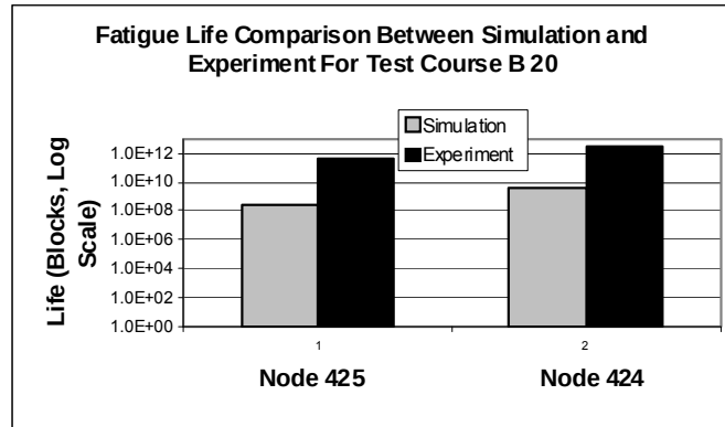
FIGURE 108 - COMPARISON OF LIVES BETWEEN SIMULATION AND EXPERIMENT FOR TEST COURSE B AT 20 MPH
