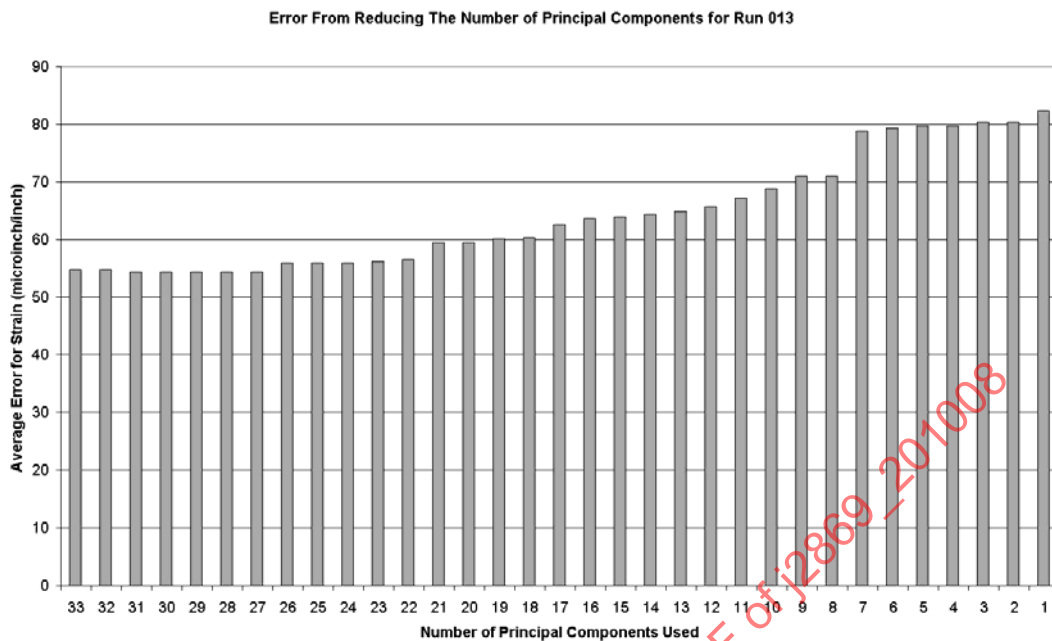
FIGURE 50 - AVERAGE STRAIN PREDICTION ERROR
