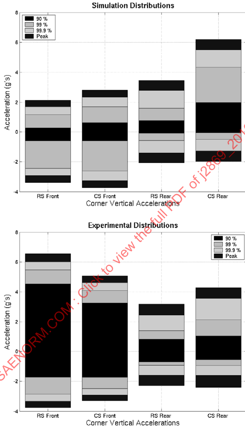
FIGURE 66 - TEST COURSE A TRAILER CORNER VERTICAL ACCELERATION DISTRIBUTIONS
