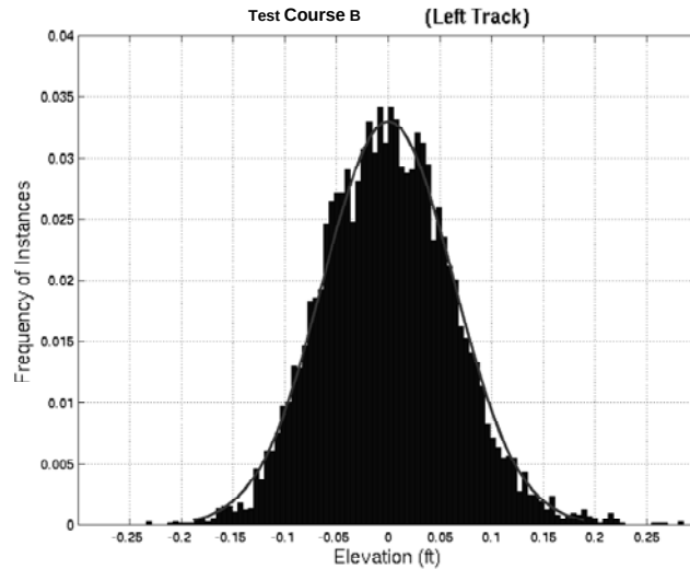
FIGURE B4 - FREQUENCY DISTRIBUTION HISTOGRAM OF TEST COURSE B PROFILE
