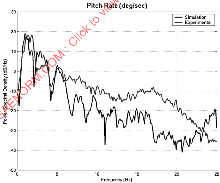
FIGURE 74 - TEST COURSE B TRAILER PITCH RATE PSD COMPARISON
