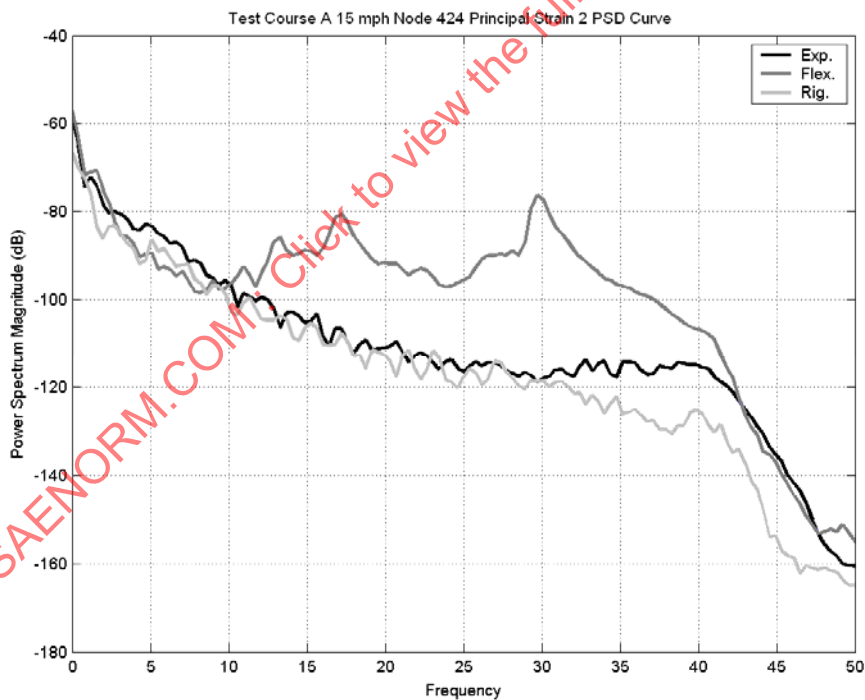
FIGURE 131 - NODE 424 PSD COMPARISON BETWEEN RIGID, FLEX., AND EXPERIMENT FOR TEST COURSE A
