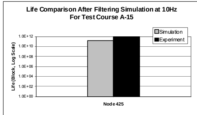
FIGURE 110 - LIFE COMPARISON BETWEEN FILTERED SIMULATION STRAIN AND EXPERIMENTAL STRAIN
