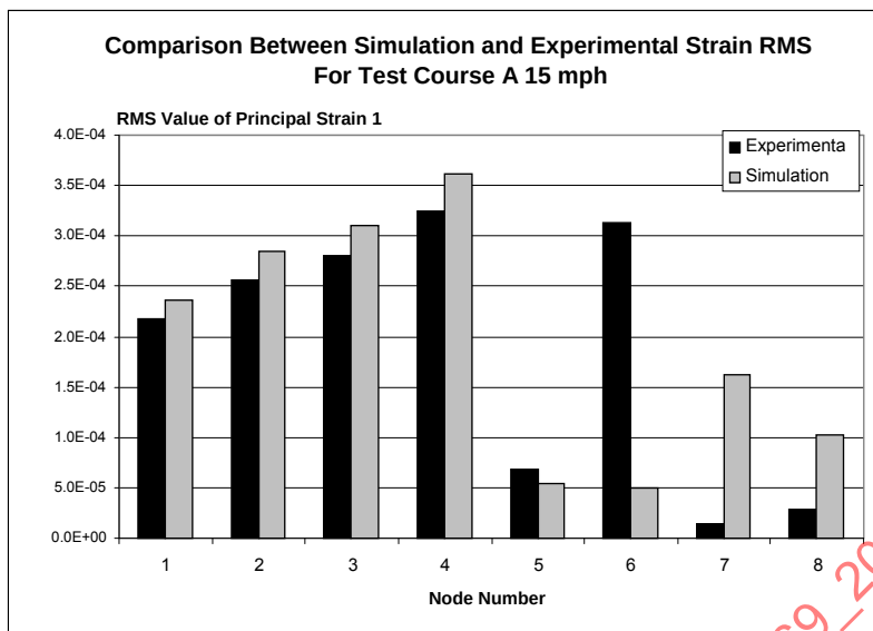
FIGURE 88 - RMS VALUE COMPARISON OF PRINCIPAL STRAIN 1
