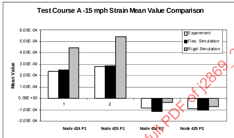
FIGURE 118 - MEAN VALUE COMPARISON OF STRAIN FOR TEST COURSE A
