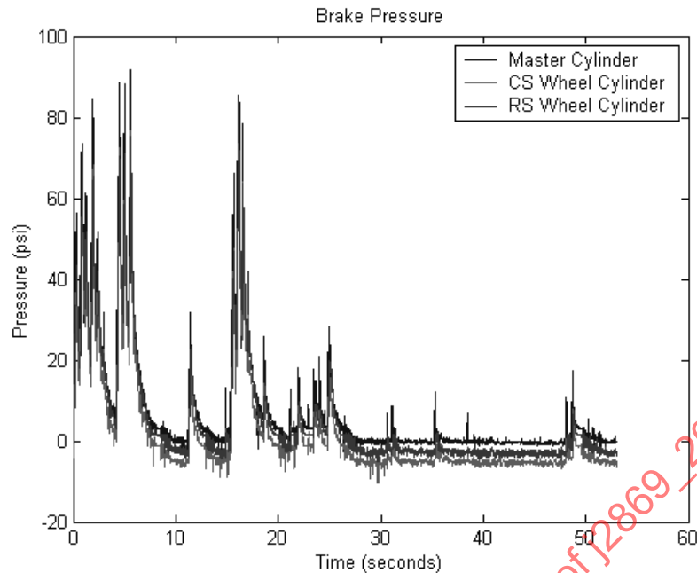
FIGURE 48 - SURGE BRAKE PRESSURES FOR TEST COURSE B
