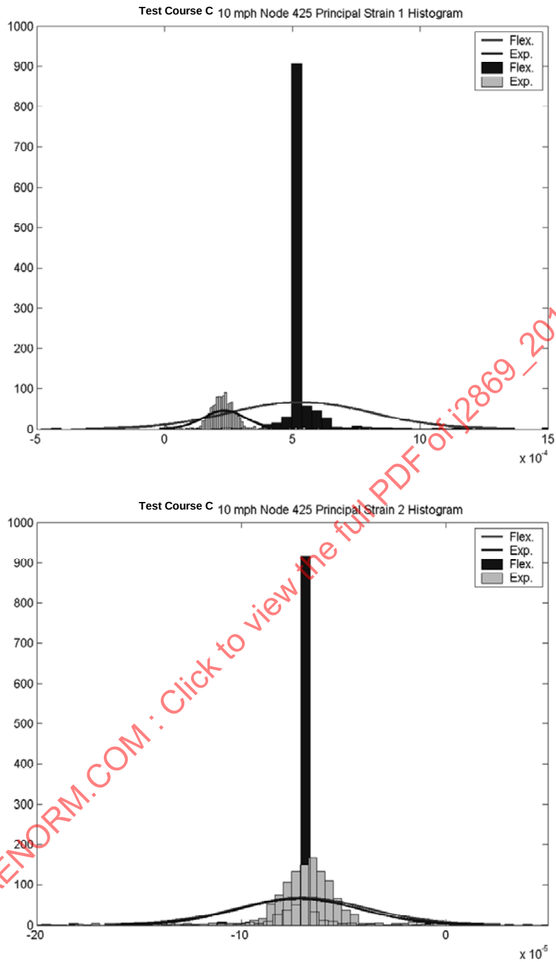
FIGURE 100 - TEST COURSE C HISTOGRAM FOR BOTH SIMULATION AND EXPERIMENT OF NODE 425
