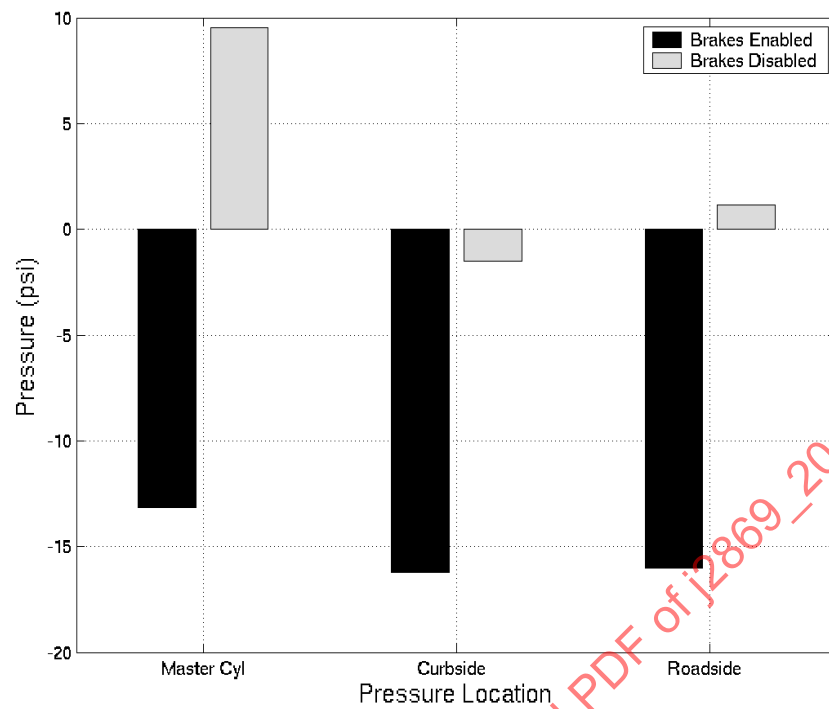
FIGURE 44 - AVERAGE BRAKE PRESSURE VALUES (PSI)
