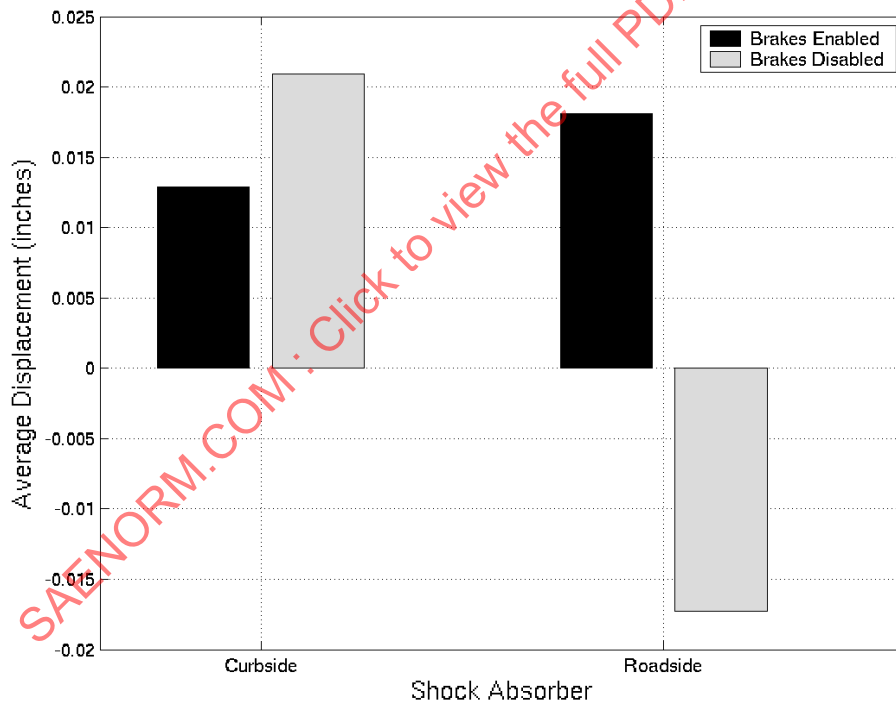
FIGURE C22 - LINEAR DISPLACEMENT AVERAGE VALUE (10 MPH)
