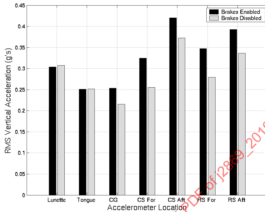
FIGURE C12 - VERTICAL RMS ACCELERATIONS FOR SEVERAL TRAILER LOCATIONS (10 MPH)
