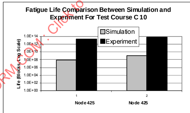
FIGURE 109 - COMPARISON OF LIVES BETWEEN SIMULATION AND EXPERIMENT FOR TEST COURSE C AT 10 MPH
