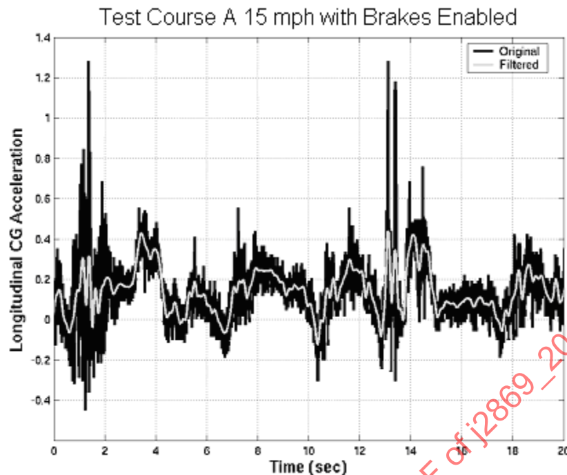
FIGURE B1 - FILTERED AND UNFILTERED LONGITUDINAL ACCELERATION TIME RESPONSES
