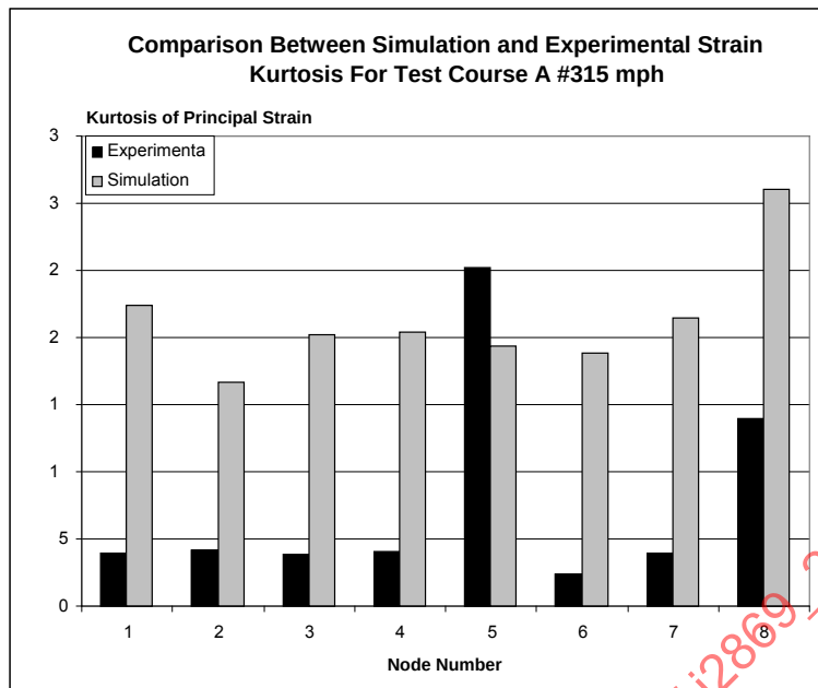
FIGURE 90 - KURTOSIS COMPARISON OF PRINCIPAL STRAIN 1
