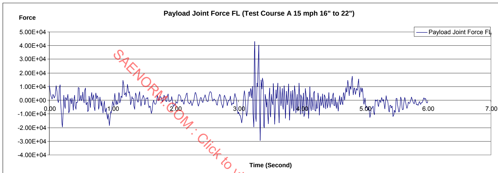
FIGURE 117 - PARTIAL ENLARGEMENT (16 TO 22 INCHES)
