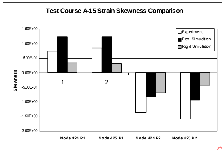
FIGURE 120 - SKEWNESS COMPARISON OF STRAIN FOR TEST COURSE A
