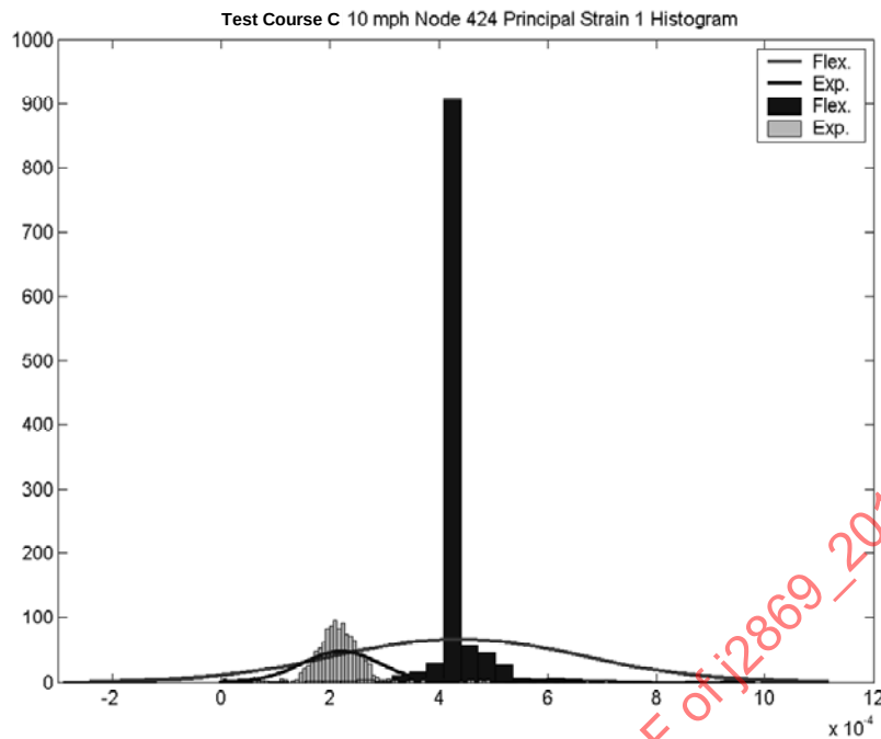
FIGURE 99 - TEST COURSE C HISTOGRAM FOR BOTH SIMULATION AND EXPERIMENT OF NODE 424
