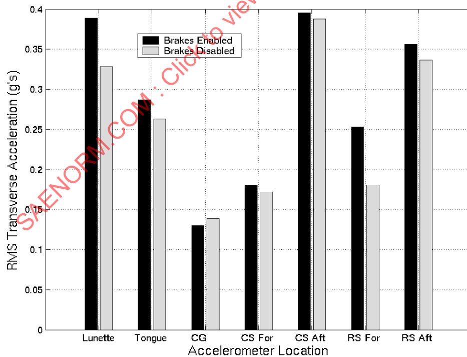
FIGURE 30 - TRANSVERSE RMS ACCELERATIONS FOR SEVERAL TRAILER LOCATIONS
