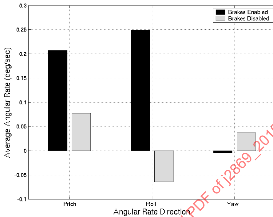
FIGURE C18 - AVERAGE RATE-GYRO ANGULAR RATES (10 MPH)
