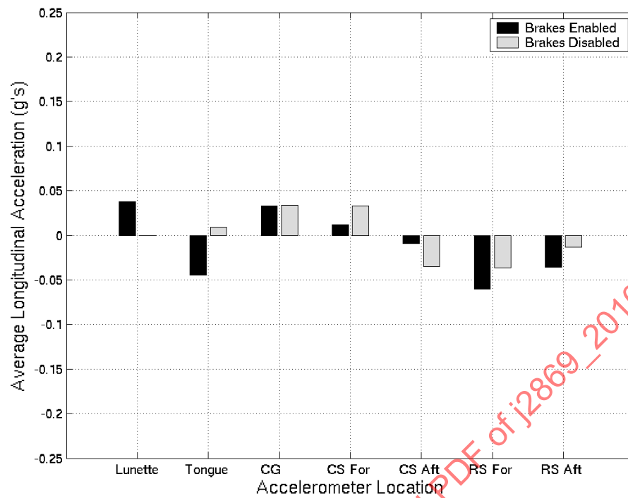
FIGURE C8 - AVERAGE LONGITUDINAL ACCELERATIONS FOR SEVERAL TRAILER LOCATIONS (10 MPH)
