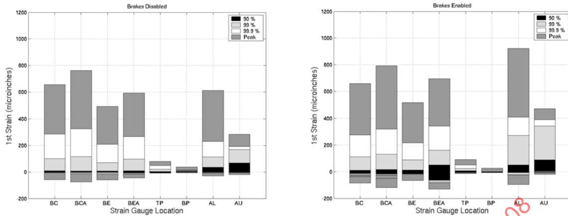
FIGURE C4 - DISTRIBUTION OF 1 ST PRINCIPAL STRAINS (10 MPH)
