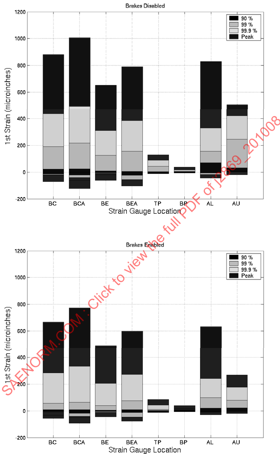
FIGURE 21 - DISTRIBUTION OF FIRST (1 ST ) PRINCIPAL STRAINS
