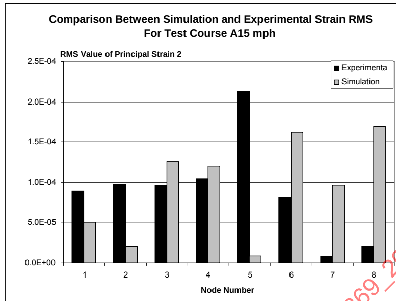
FIGURE 92 - RMS VALUE COMPARISON OF PRINCIPAL STRAIN 2
