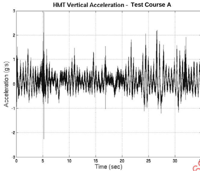
FIGURE B6 - TIME DOMAIN REPRESENTATION OF DATA
