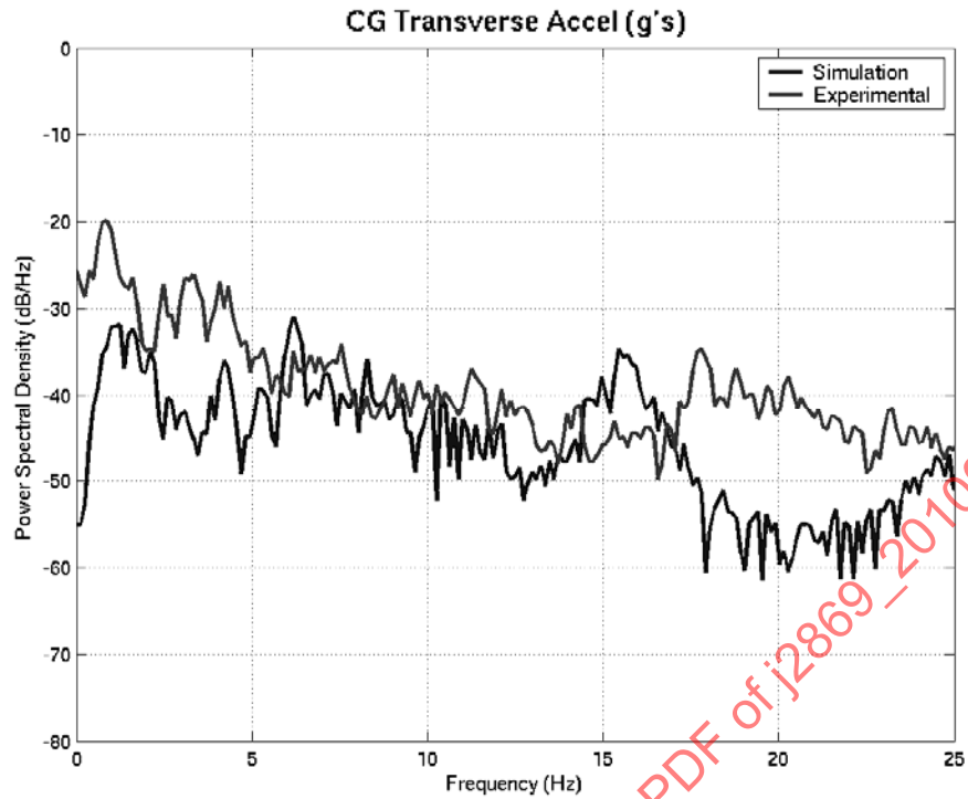
FIGURE 54 - TEST COURSE A CG TRANSVERSE ACCELERATION PSD COMPARISON
