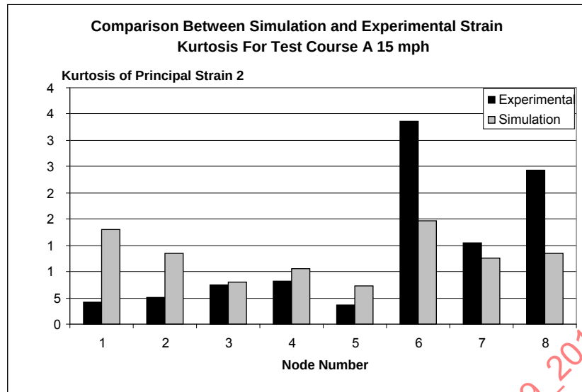
FIGURE 94 - KURTOSIS COMPARISON OF PRINCIPAL STRAIN 2
