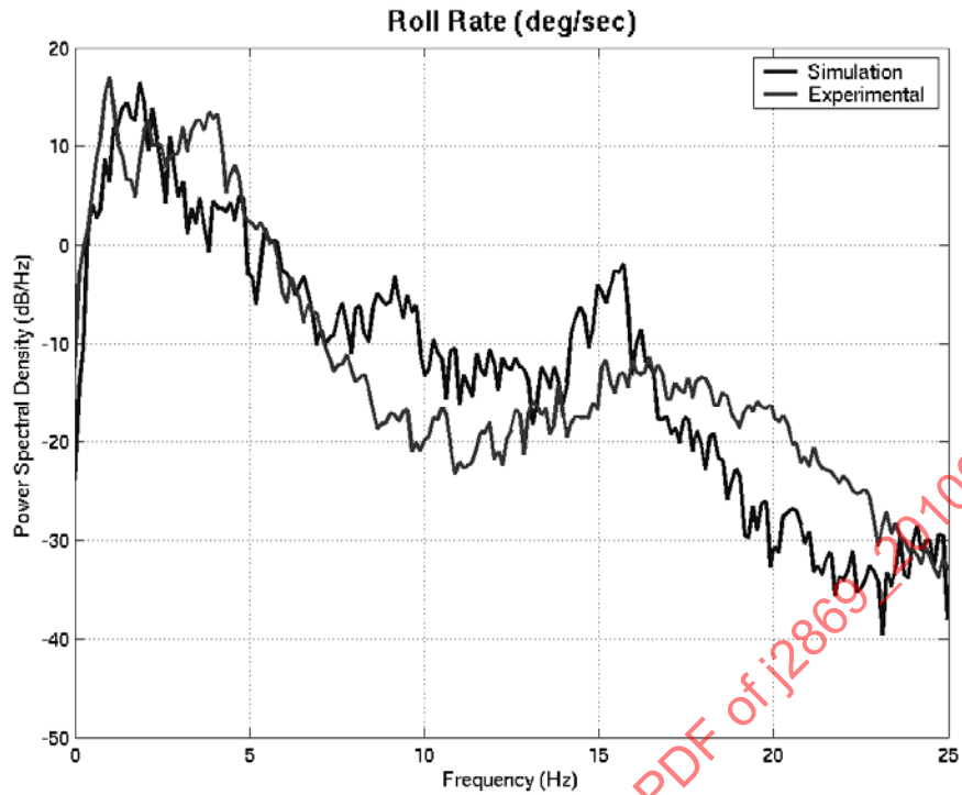
FIGURE 73 - TEST COURSE B TRAILER ROLL RATE PSD COMPARISON
