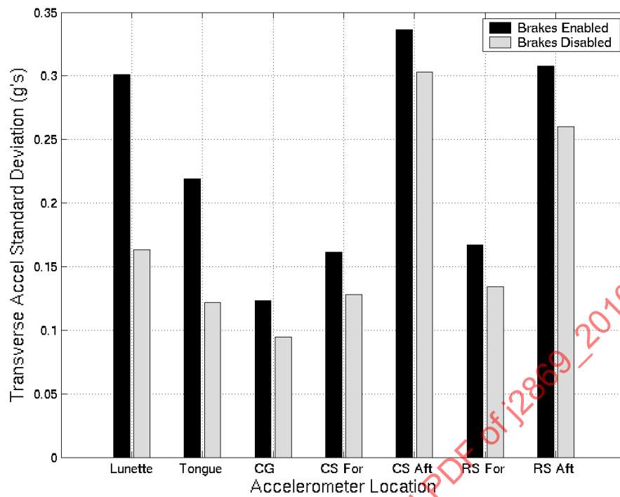
FIGURE C10 - TRANSVERSE ACCELERATION STANDARD DEVIATION FOR SEVERAL TRAILER LOCATIONS (10 MPH)
