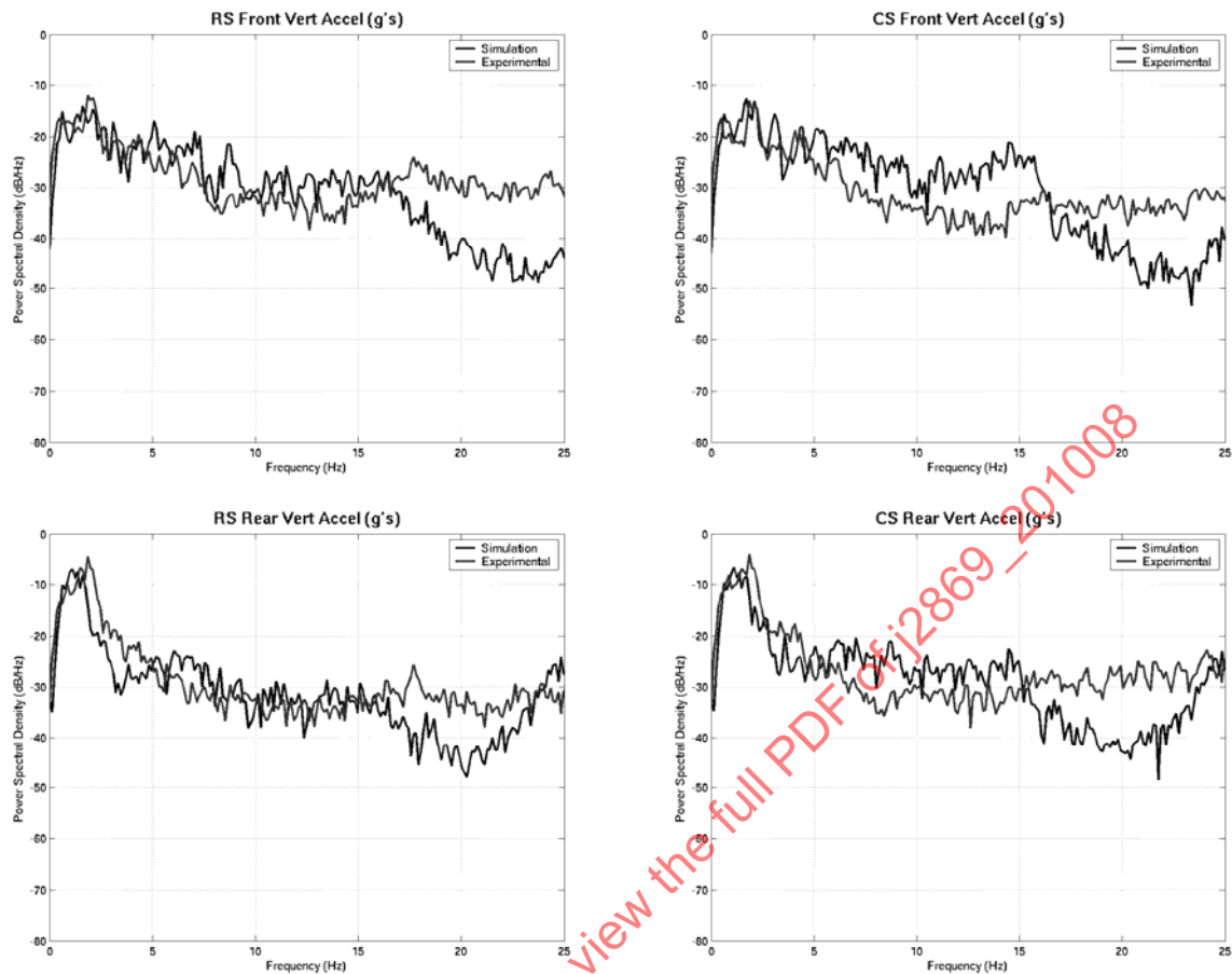
FIGURE 65 - TEST COURSE A TRAILER CORNER VERTICAL ACCELERATION PSD COMPARISON
