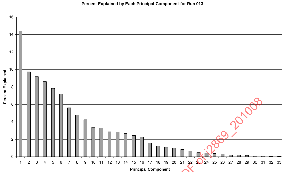
FIGURE 49 - PERCENT OF DATA EXPLAINED BY EACH PRINCIPAL COMPONENT (BRAKES ENABLED)
