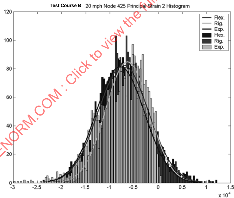
FIGURE 129 - HISTOGRAM FOR BOTH RIGID AND FLEXIBLE BODY SIMULATION AND EXPERIMENT OF NODE 425
