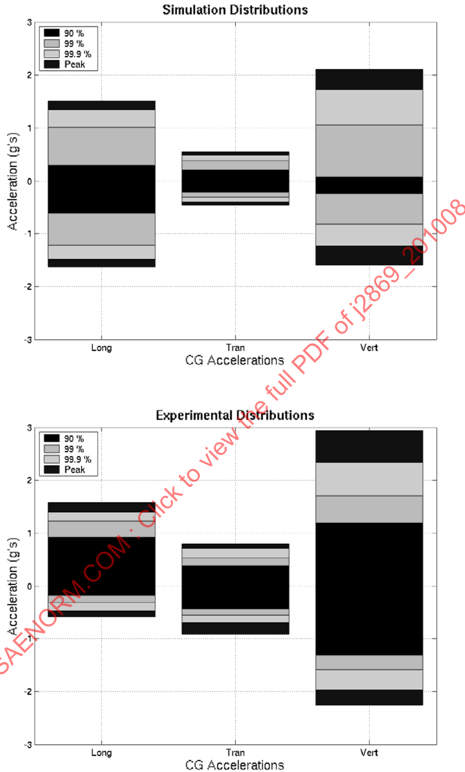
FIGURE 56 - TEST COURSE A CG ACCELERATION STATISTICAL DISTRIBUTIONS
