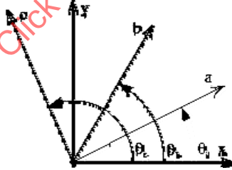
FIGURE B2 - GENERALIZED STRAIN-GAUGE ROSETTE ORIENTATIONS
