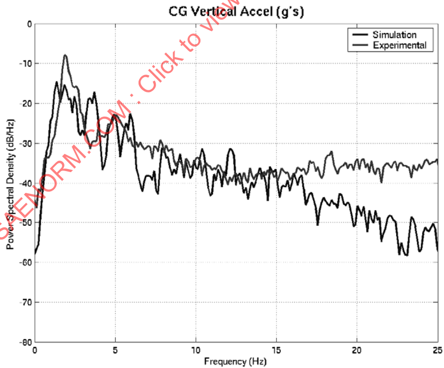
FIGURE 71 - TEST COURSE B CG VERTICAL ACCELERATION PSD COMPARISON
