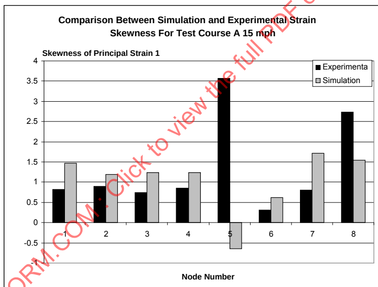
FIGURE 89 - SKEWNESS COMPARISON OF PRINCIPAL STRAIN 1
