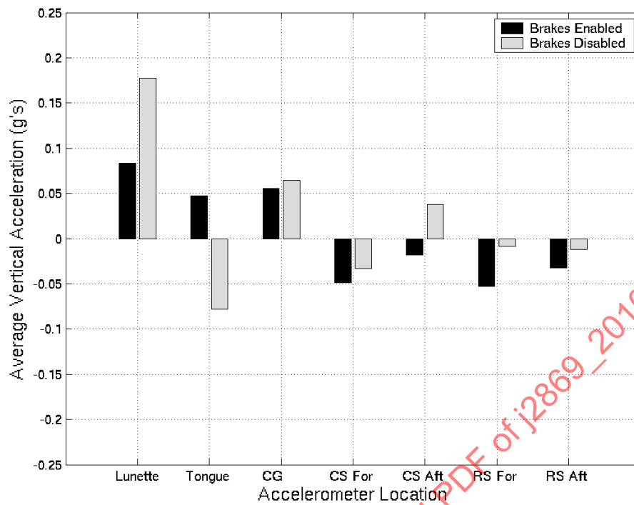
FIGURE C6 - AVERAGE VERTICAL ACCELERATIONS FOR SEVERAL TRAILER LOCATIONS (10 MPH)
