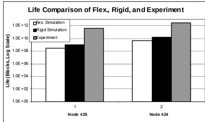
FIGURE 135 - LIFE COMPARISON OF FLEXIBLE, RIGID SIMULATION AND EXPERIMENT FOR TEST COURSE B
