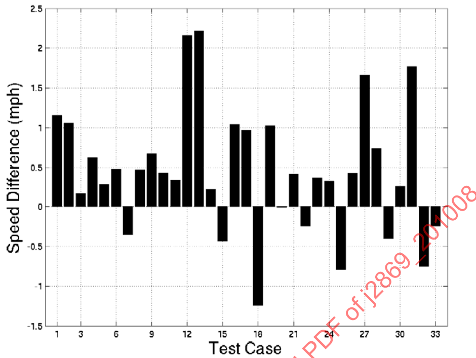
FIGURE 14 - DIFFERENCE BETWEEN AVERAGE AND NOMINAL SPEEDS
