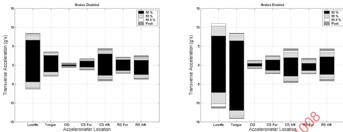
FIGURE C16 - TRANSVERSE ACCELERATION STATISTICS FOR SEVERAL TRAILER LOCATIONS (10 MPH)
