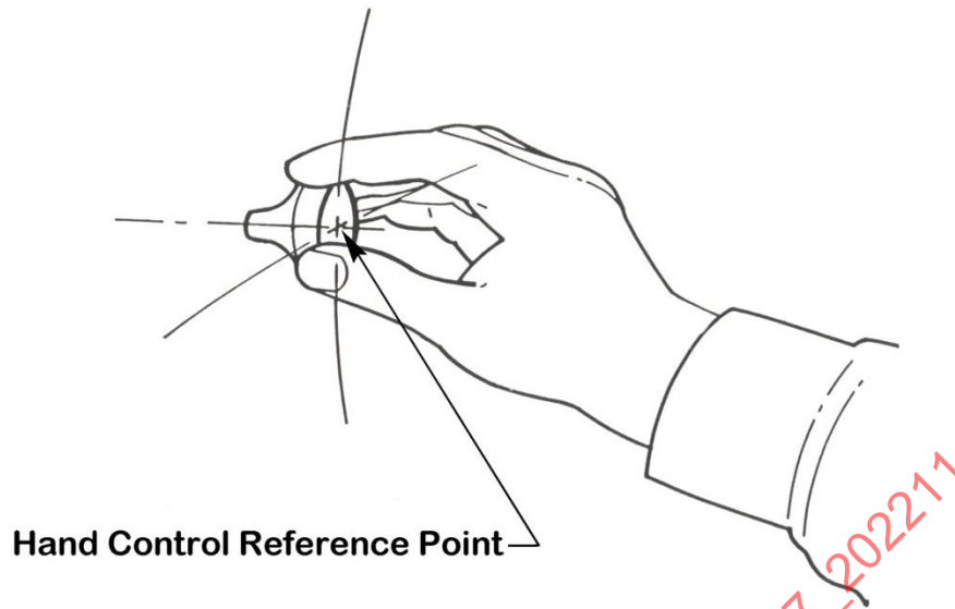
Figure 1 - three-finger grasping reach to a 25 mm diameter control knob; All measurements for the hand reach envelopes are referenced to the center of the control knob face
