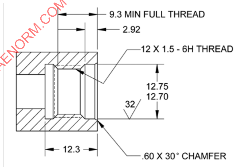
Figure 4 - Female fitting
