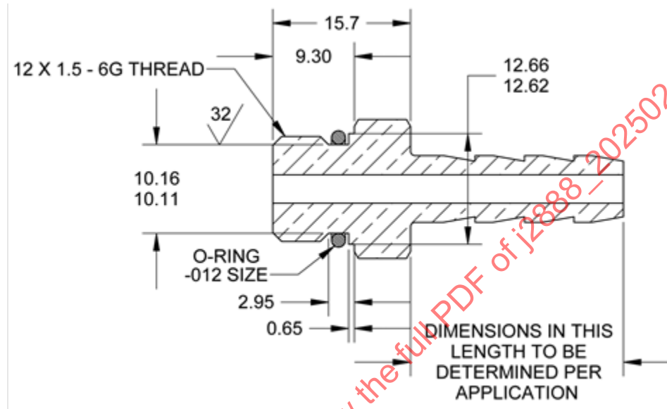
Figure 3 - Barb and thread
