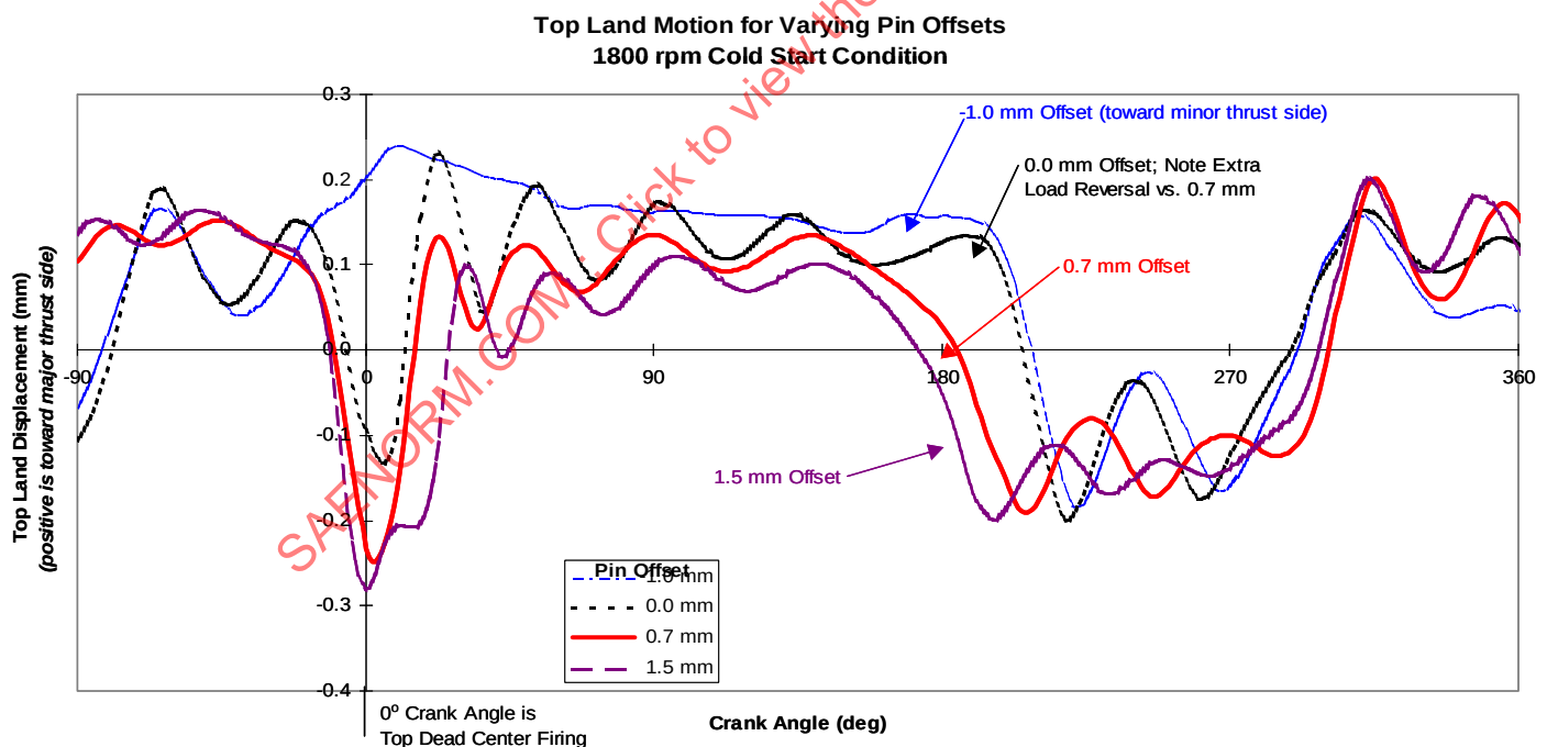
FIGURE 15 - EXAMPLE OF THE EFFECT OF PIN OFFSET ON PISTON MOTION
