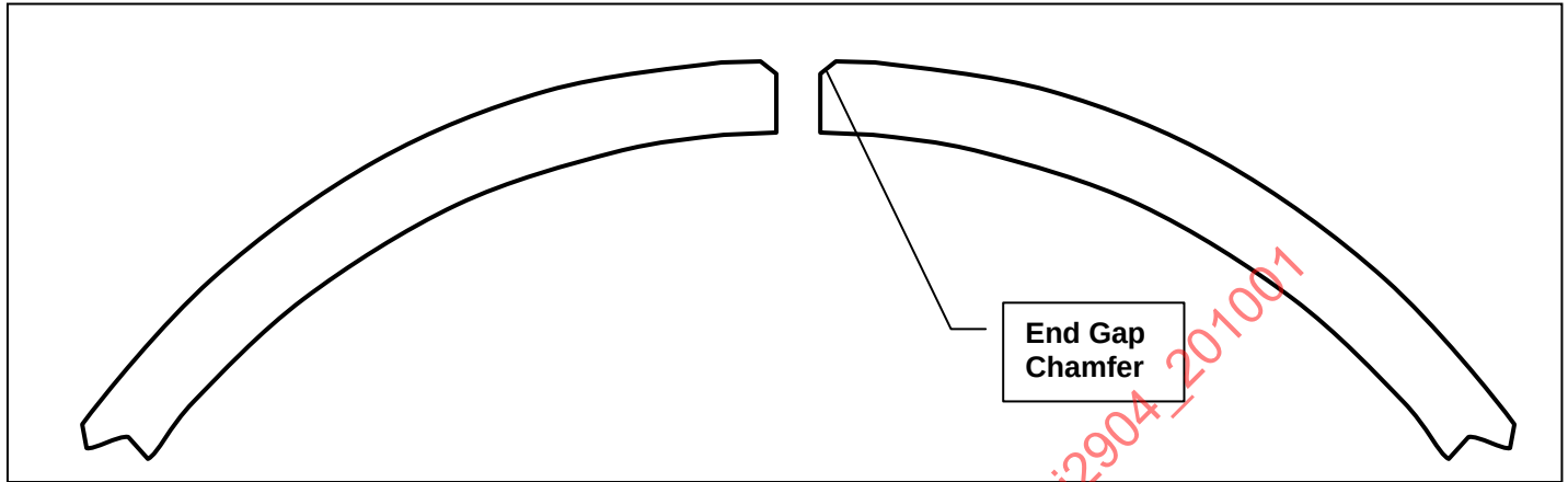
FIGURE 33 - END GAP CHAMFER
