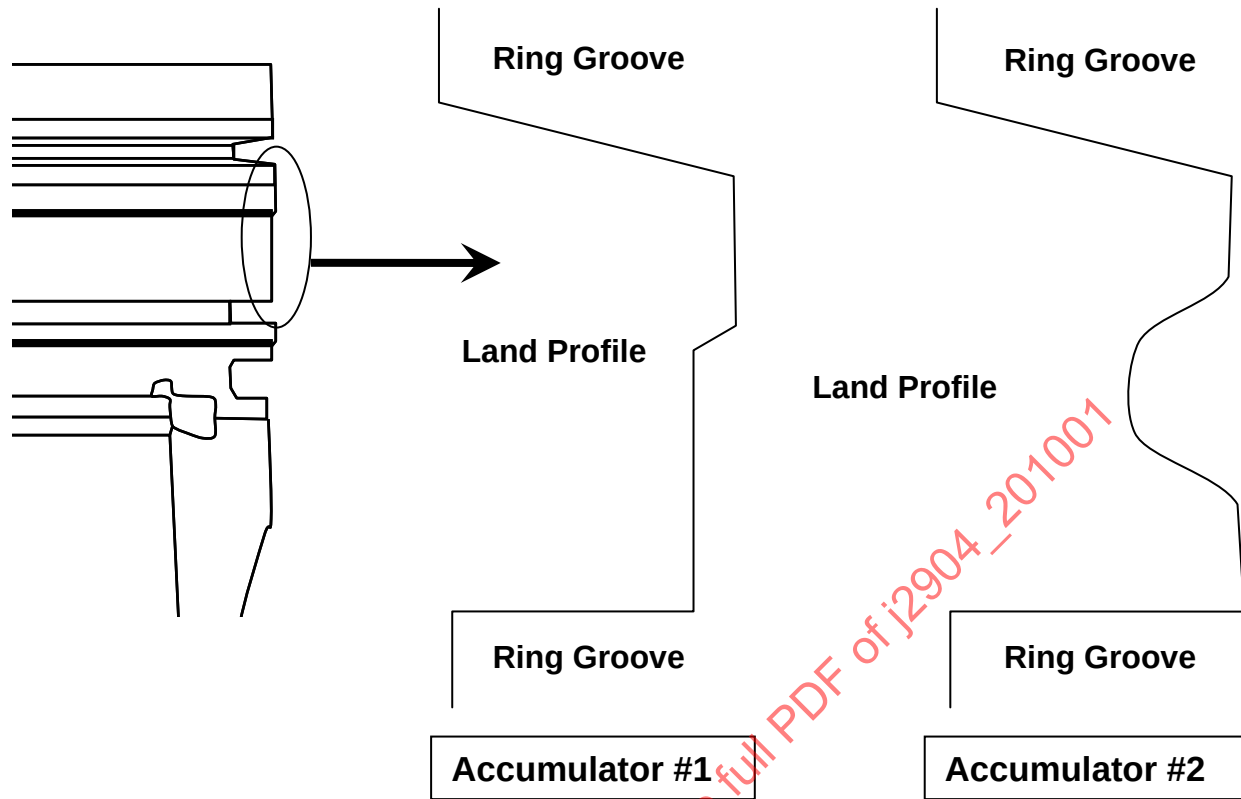
FIGURE 12 - LAND ACCUMULATOR GROOVES
