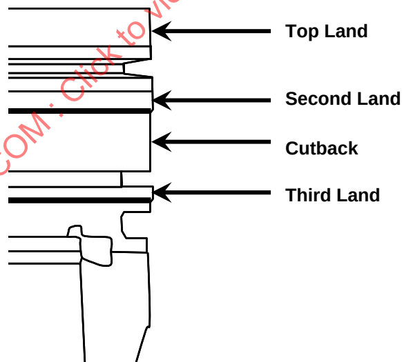
FIGURE 9 - LAND DIAMETERS
