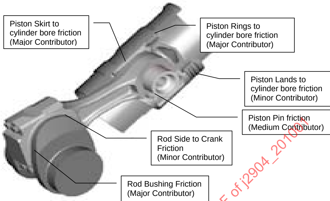
FIGURE 1 - LOCATIONS OF POWER CYLINDER FRICTION
