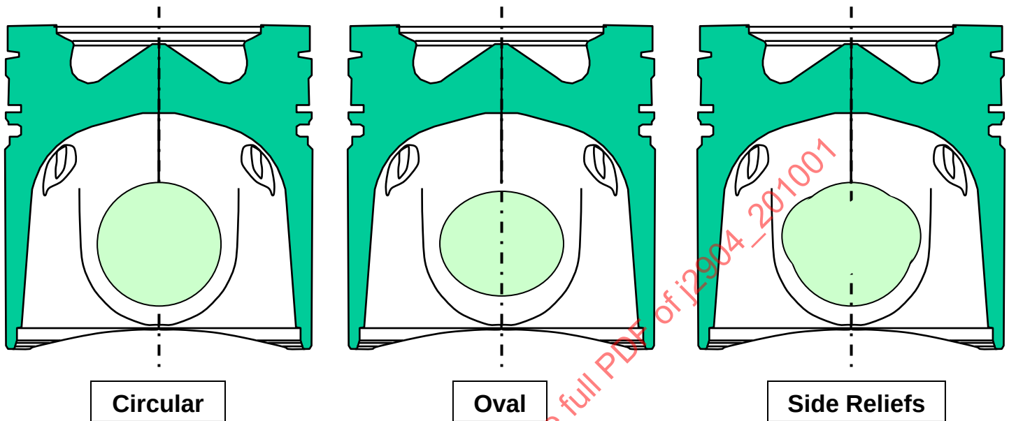
FIGURE 24 - EXAMPLES OF DIFFERENT PIN BORE CIRCUMFERENTIAL PROFILES
