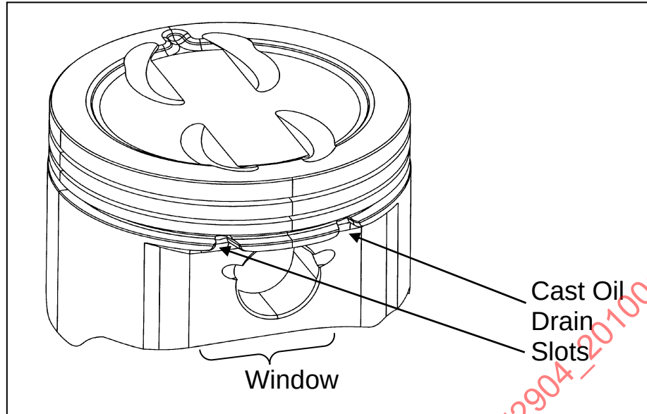
FIGURE 13 - OIL DRAIN TRANS SLOTS
