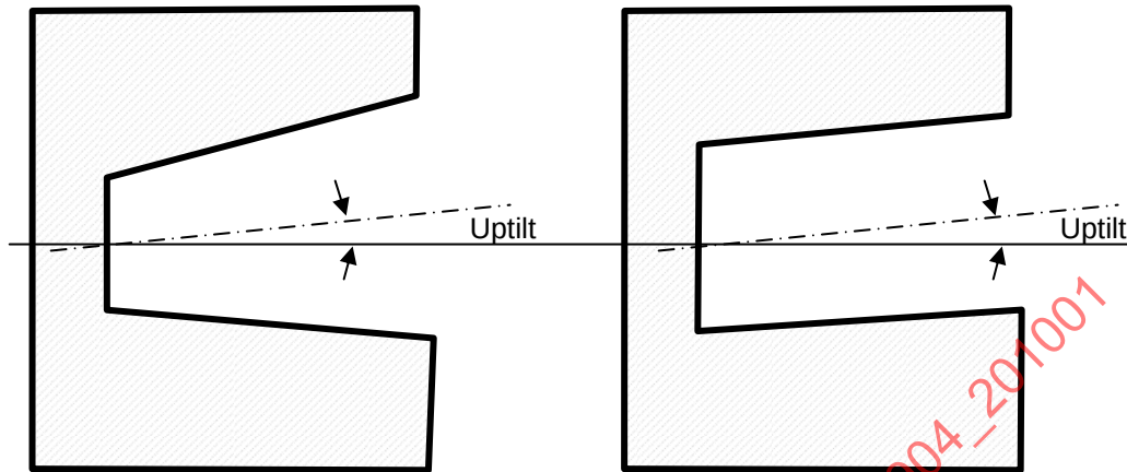
FIGURE 6 - GROOVE UPTILT
