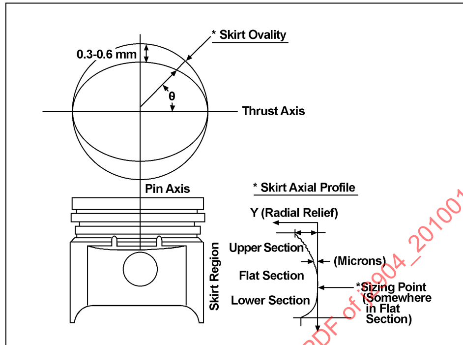
FIGURE 16 - PISTON PROFILES
