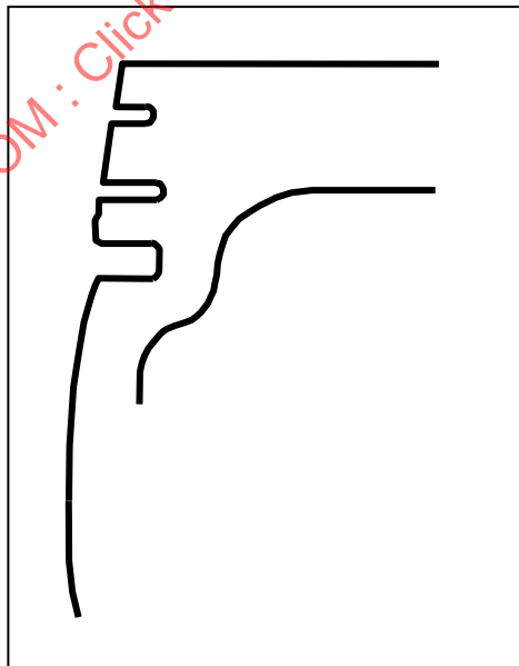
FIGURE 11 - LAND AND SKIRT PROFILE EXAMPLE
