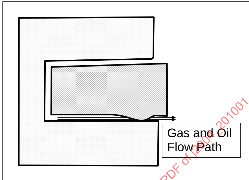
FIGURE 37 - RING STRAIGHTNESS EXAMPLE
