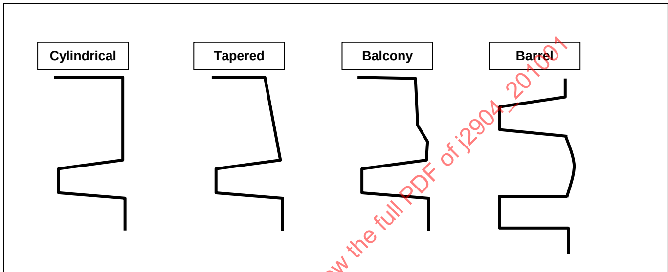
FIGURE 10 - LAND PROFILES
