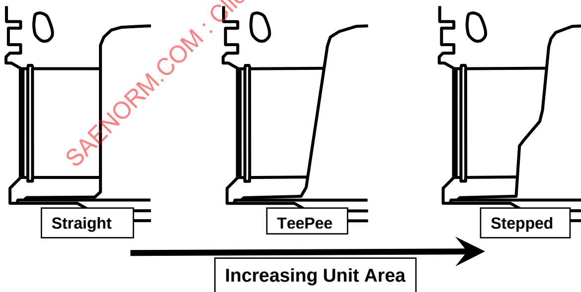
FIGURE 21 - EXAMPLES OF PIN BORE DESIGNS
