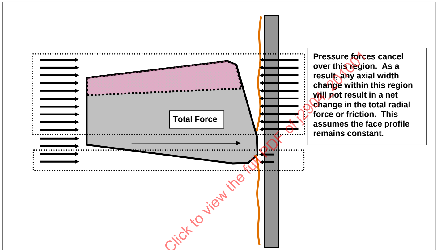
FIGURE 28 - ILLUSTRATION OF RADIAL GAS FORCES ACTING ON THE RING
