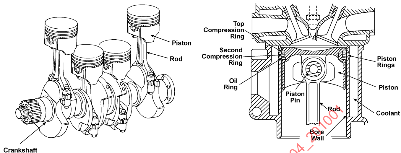
FIGURE 2 - POWER CYLINDER
