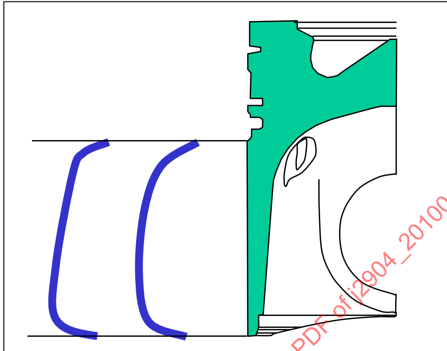
FIGURE 17 - SKIRT AXIAL PROFILES
