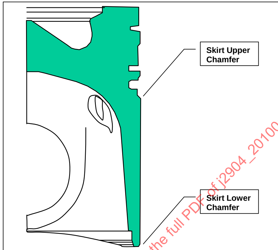
FIGURE 19 - SKIRT CHAMFERS
