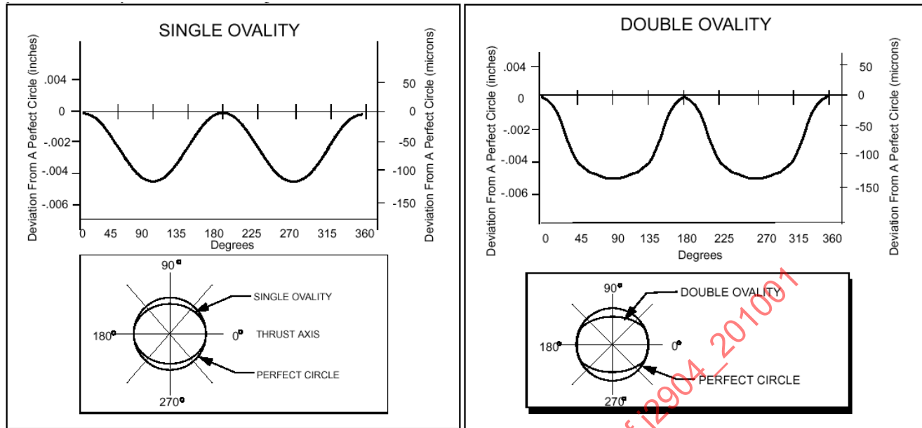
FIGURE 18 - SKIRT CIRCUMFERENTIAL CONTOURS
