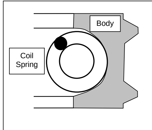
FIGURE 38 - TWO PIECE OIL RING
