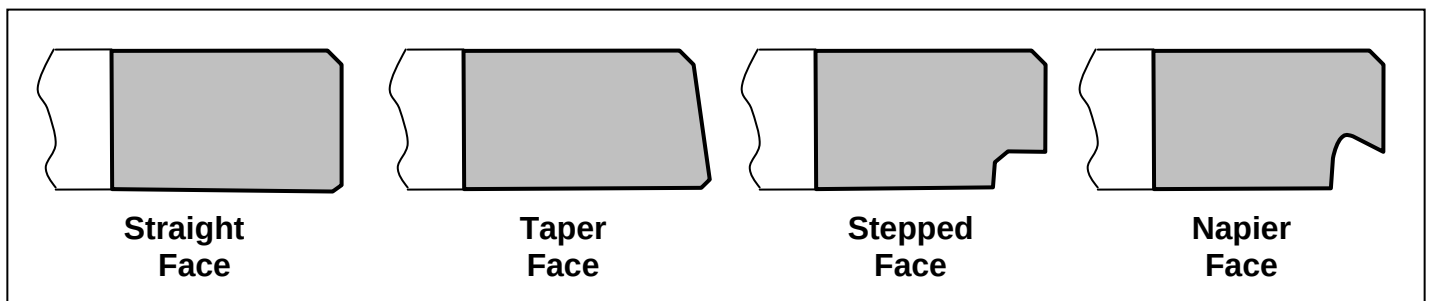
FIGURE 32 - SECOND RING FACE PROFILES
