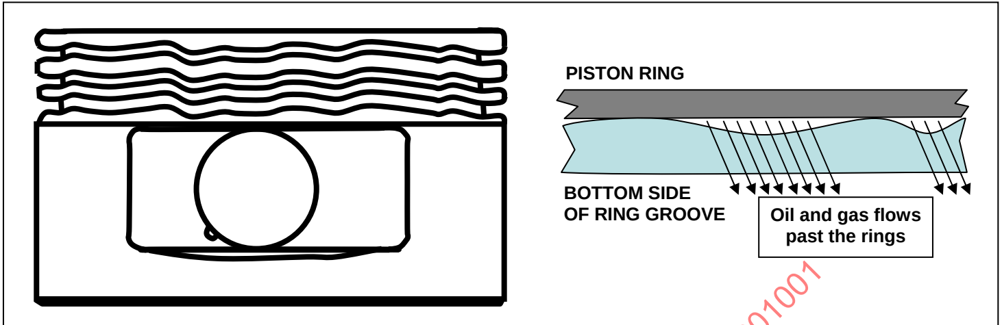
FIGURE 7 - GROOVE WAVINESS
