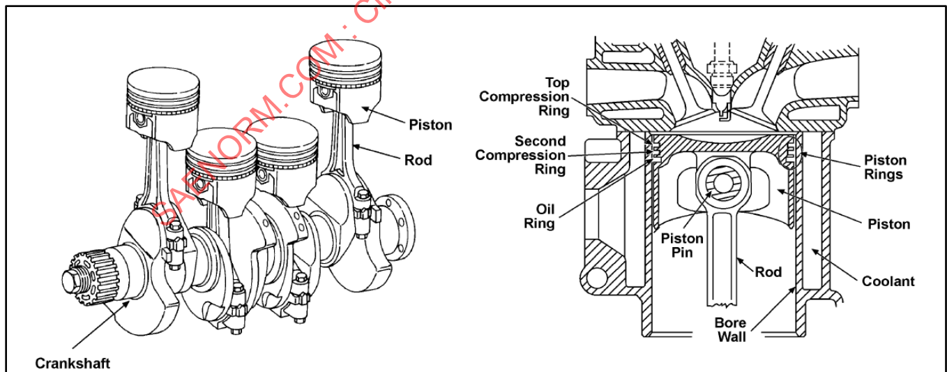
Figure 2 - Power cylinder
