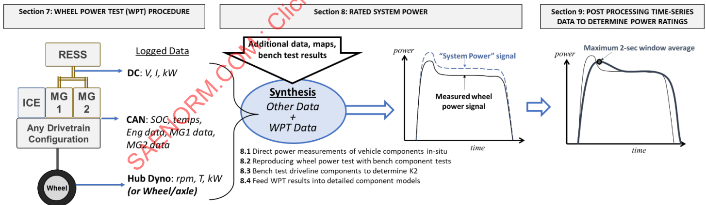
Figure 3 - SAE J2908 testing and post-processing workflow diagram
