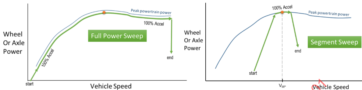
Figure 2 - Finding V_{MP} using power sweep procedure
