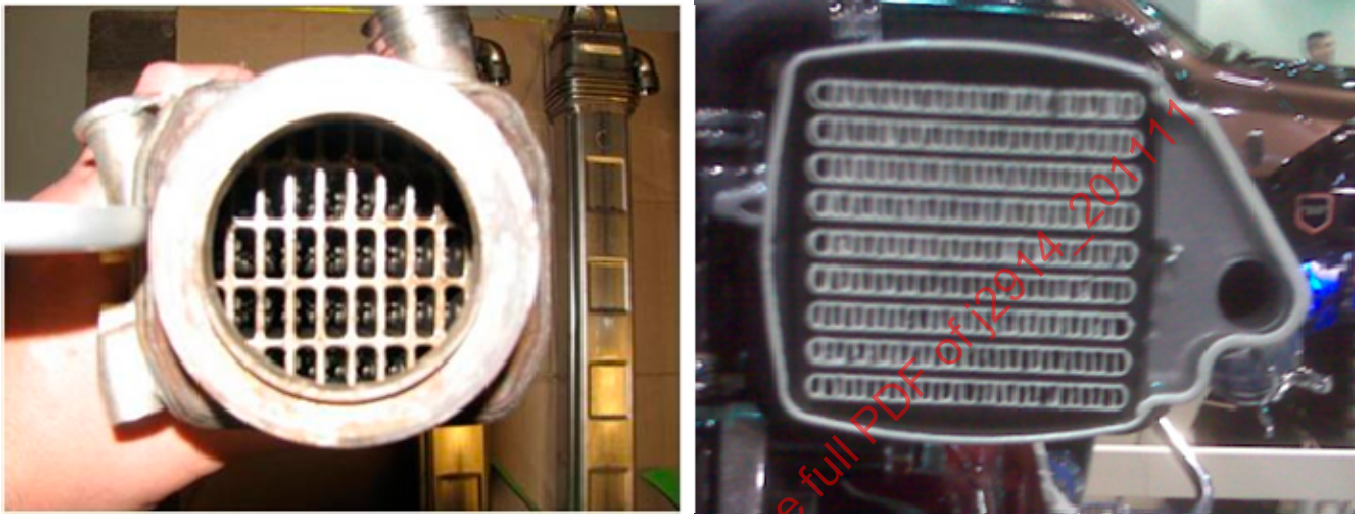
FIGURE 6 - RECTANGULAR TUBES IN STACKED OR TUBE MATRIX INTERNAL CONFIGURATIONS
