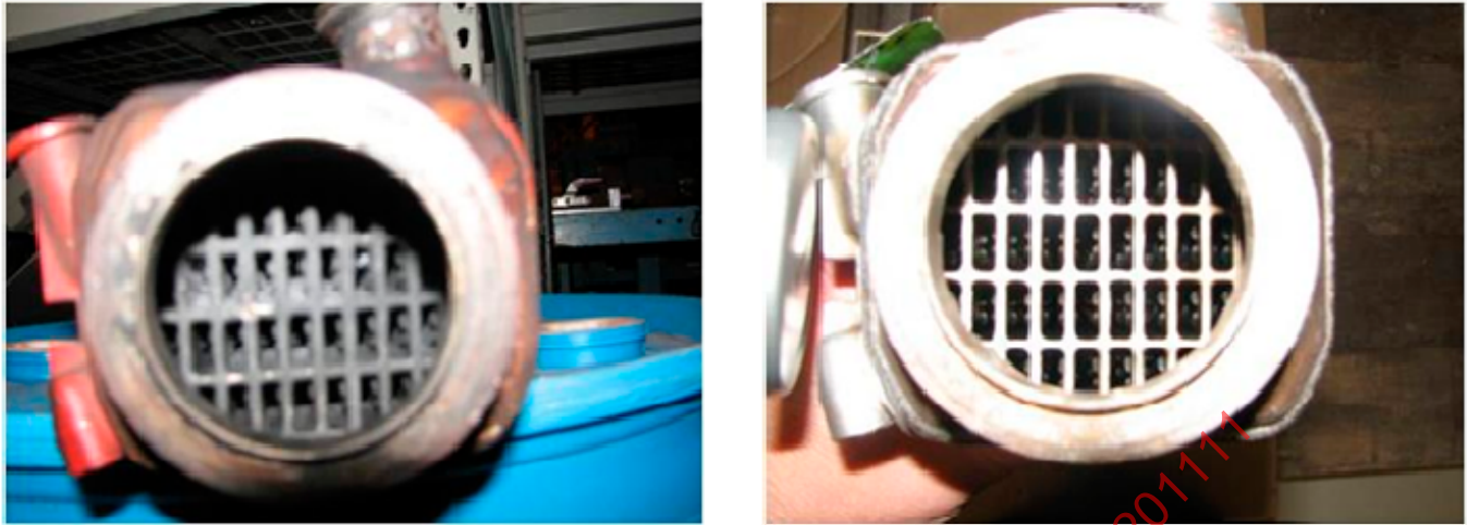
FIGURE 8 - VISUAL ILLUSTRATION OF FOULED EGR COOLER INLET AND TUBES
