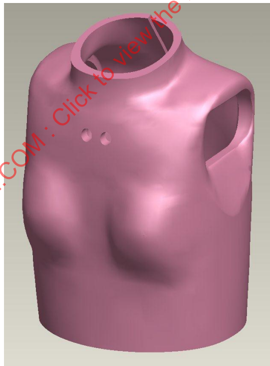
FIGURE 3 - 3D SHAPE OF THE HARMONIZED SMALL FEMALE JACKET
