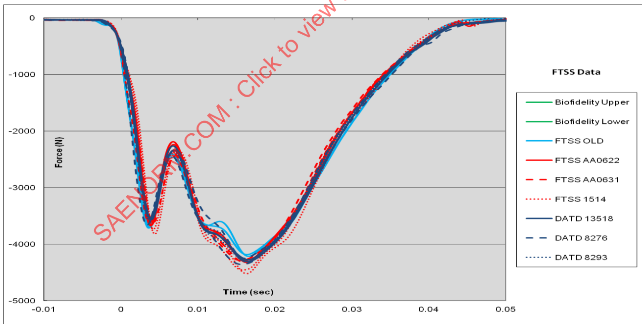
FIGURE 10 - COMPARISON OF PENDULUM FORCE OF AN OLD AND NEW JACKET ON THE SAME DUMMY
