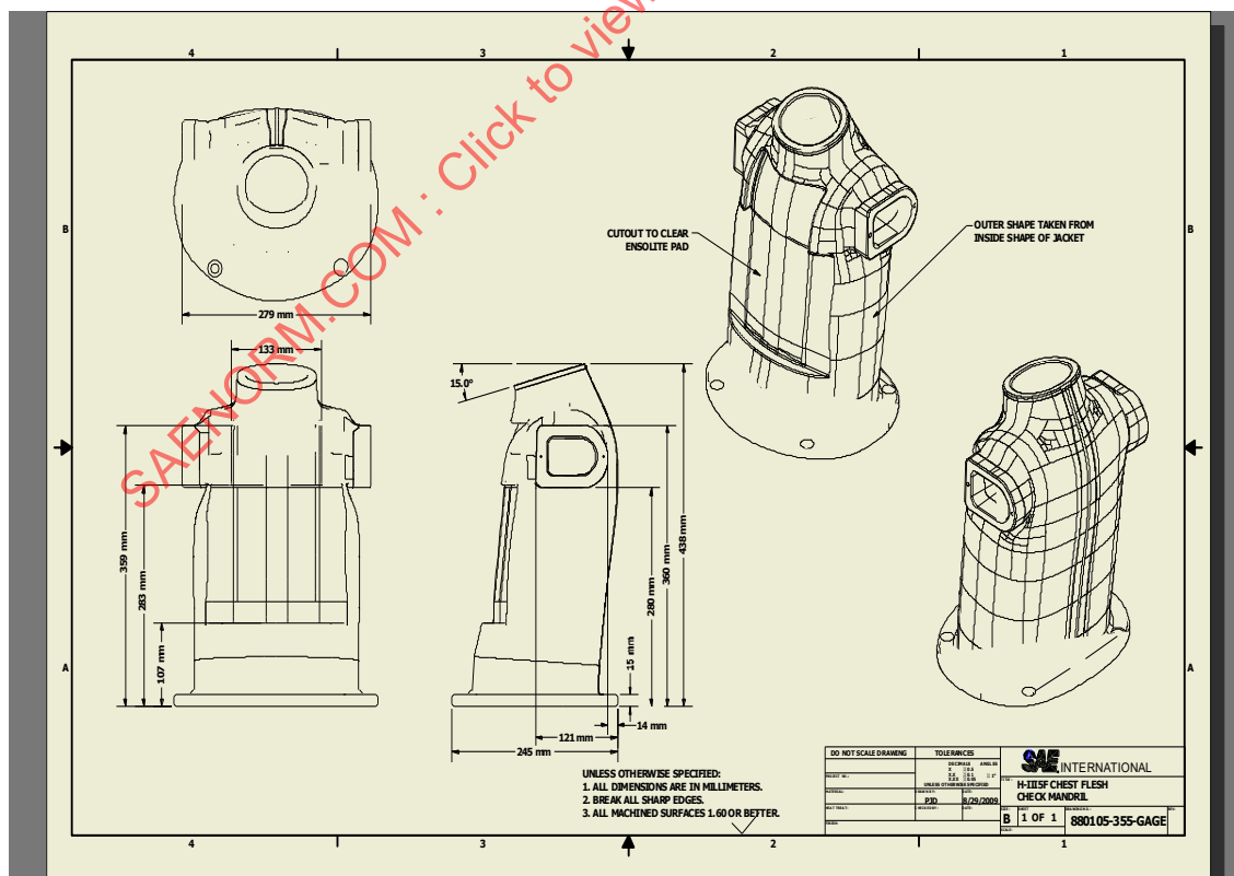
FIGURE 8 - MANDREL DRAWING
