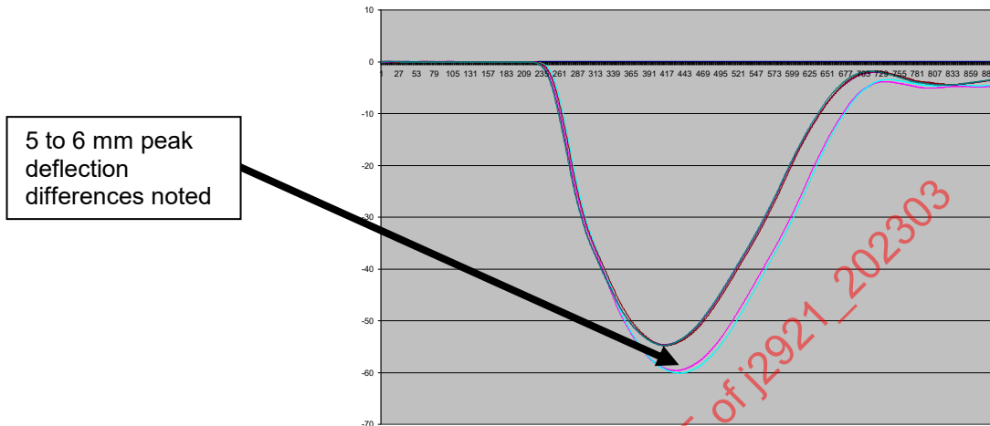
FIGURE 2 - COMPARISON OF TWO JACKETS USING SAME DUMMY FOR STANDARD THORAX IMPACT TEST
