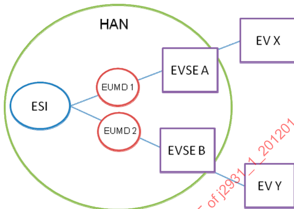
FIGURE 3 - ELECTRICAL NETWORK – MULTIPLE EVSE AND MULTIPLE EUMD
