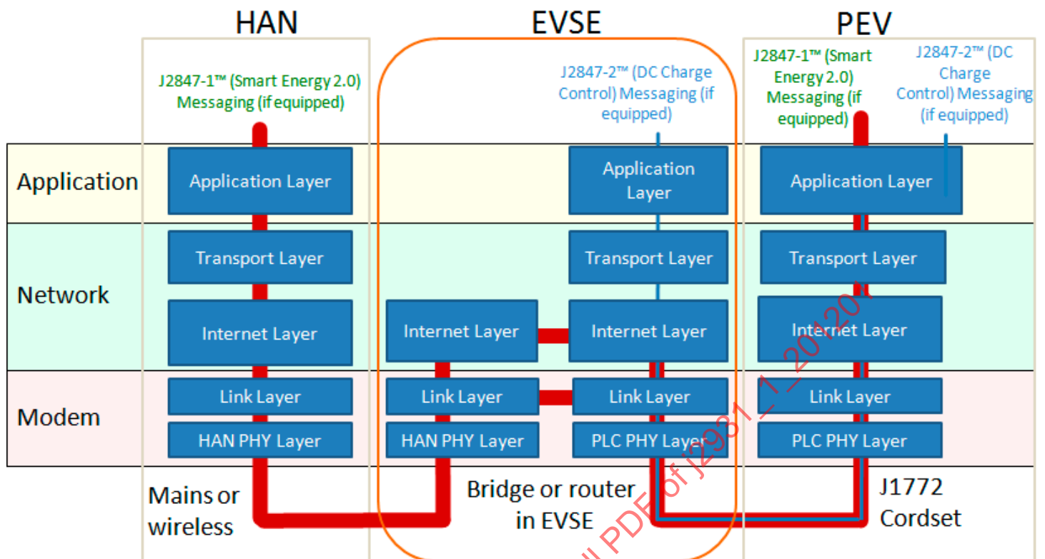
FIGURE 6 – PROPOSED COMMUNICATION STACK
