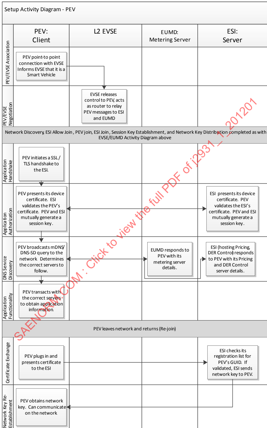
FIGURE 10 - SETUP ACTIVITY DIAGRAM – PEV (W/ASSOCIATION)
