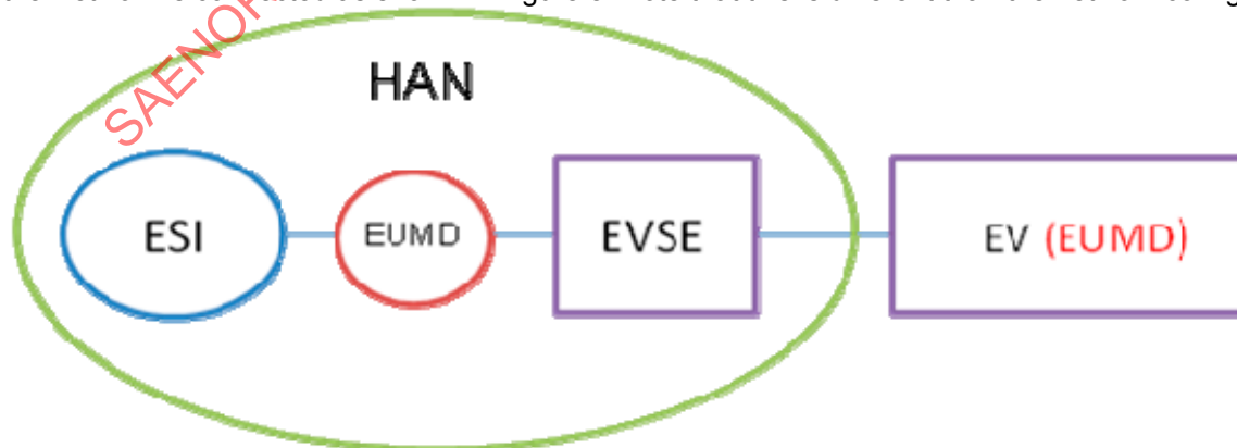
FIGURE 8 - OVERALL ELECTRICAL SYSTEM ARCHITECTURE
