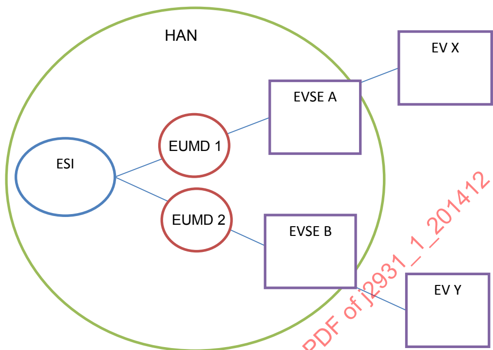
FIGURE 6 - ELECTRICAL NETWORK – MULTIPLE EVSE AND MULTIPLE EUMD
