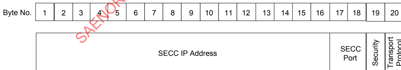
FIGURE 20 - SECC DISCOVERY RESPONSE MESSAGE PAYLOAD
