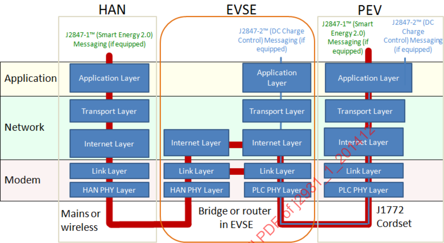
FIGURE 9 - PROPOSED COMMUNICATION STACK
