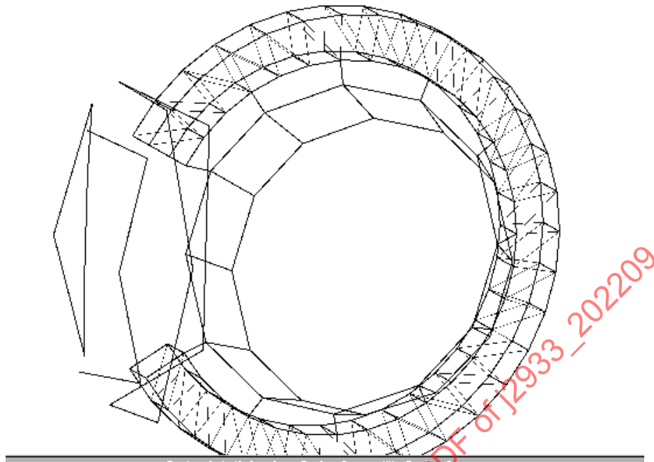
Figure B1 - Disc brake corner and component geometry example
