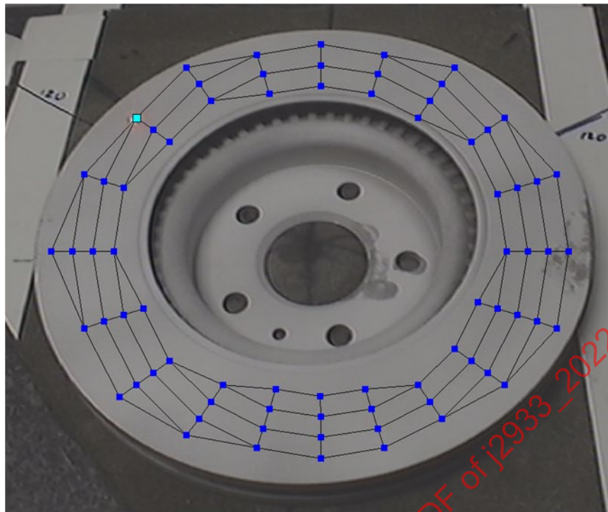
Figure B3 - Rotor example laser vibrometer measurement points
