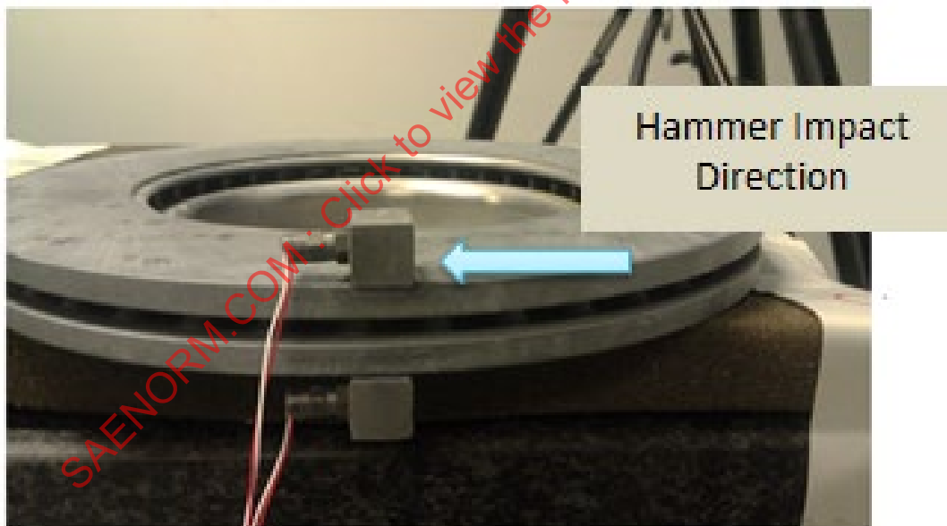
Figure B4 - Rotor in-plane mode alternative measurement method
