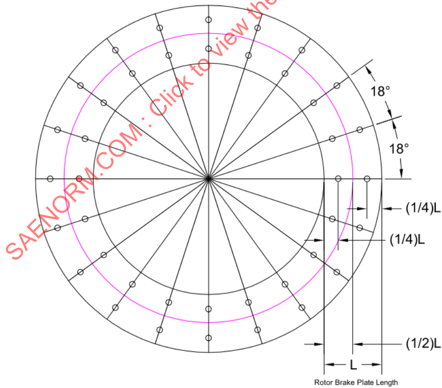
Figure B2 - Minimal point placement on rotor
