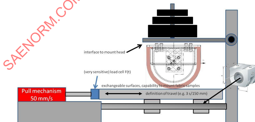
Figure 7 - Friction measuring device concept
