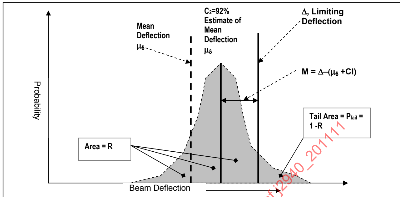
FIGURE 6 - USING VALIDATED MODEL TO ASSESS RELIABILITY; A SIMPLIFIED DEPICTION
