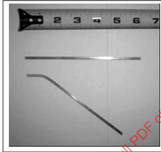
FIGURE 4 - V&V OF RESULTS: SQUARE SECTION BEAM IN PLASTIC BENDING TEST
