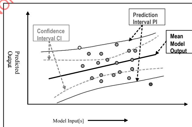
FIGURE 8 - PROCEDURE TO DEMONSTRATE AND ASSESS PREDICTIVE CAPABILITY, A TEST OF BOTH THE MODEL AND THE V&V PROCESS ITSELF. THE RESULT IS A “DATA-CENTRIC” FORM OF PEER REVIEW: THE NEW DATA SERVE AS “PEERS” IN THE REVIEW
