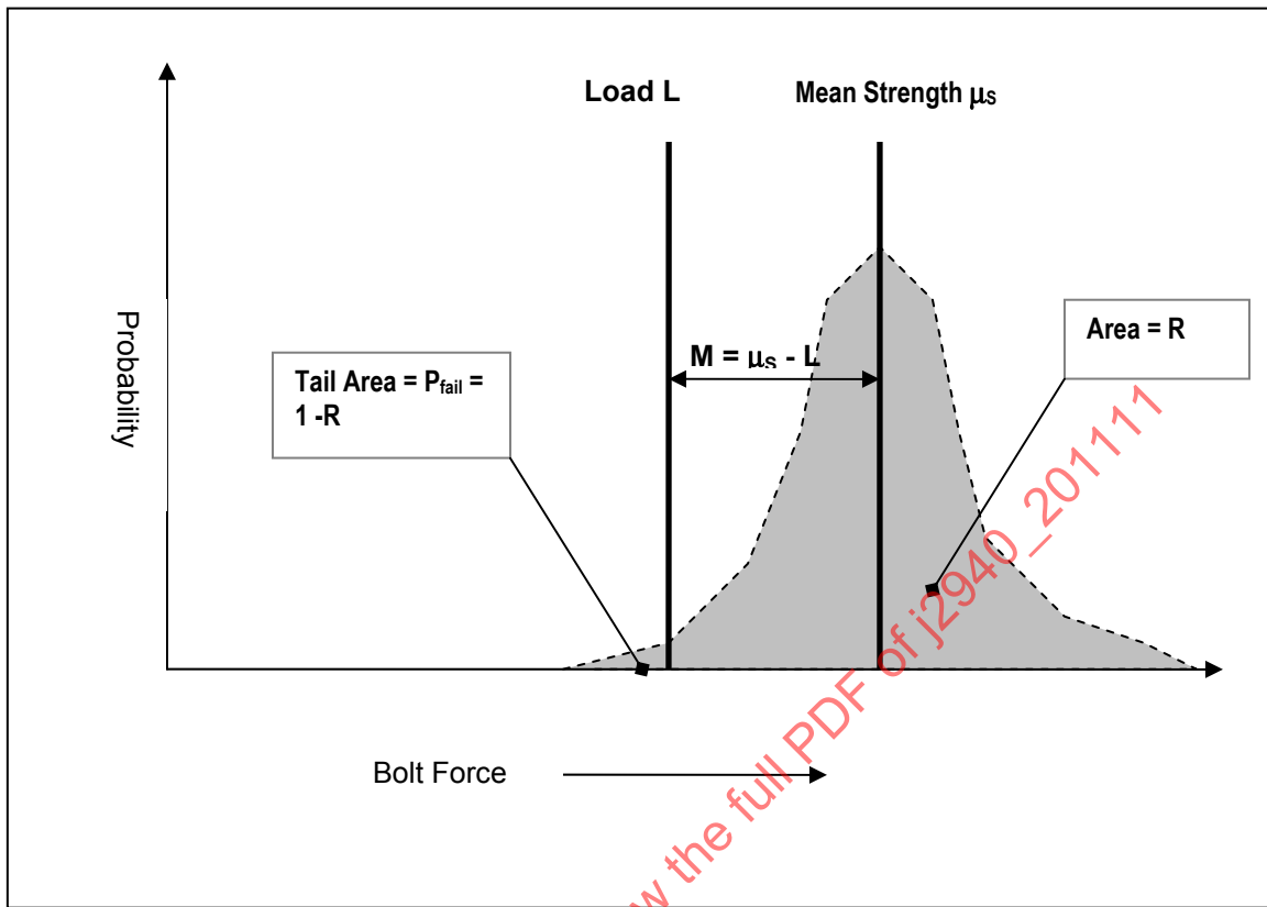
FIGURE 1 - QUANTITIES FOR SIMPLE RELIABILITY ASSESSMENT, NORMAL DISTRIBUTION.
