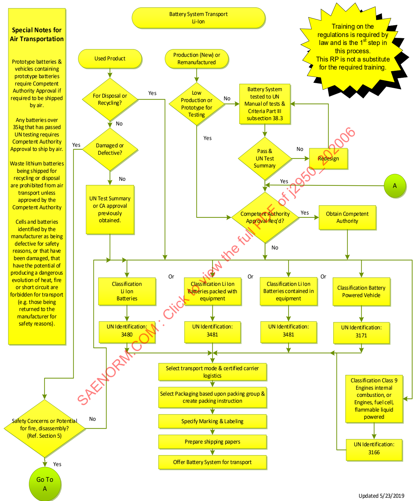
Figure 1 - Battery type determination
