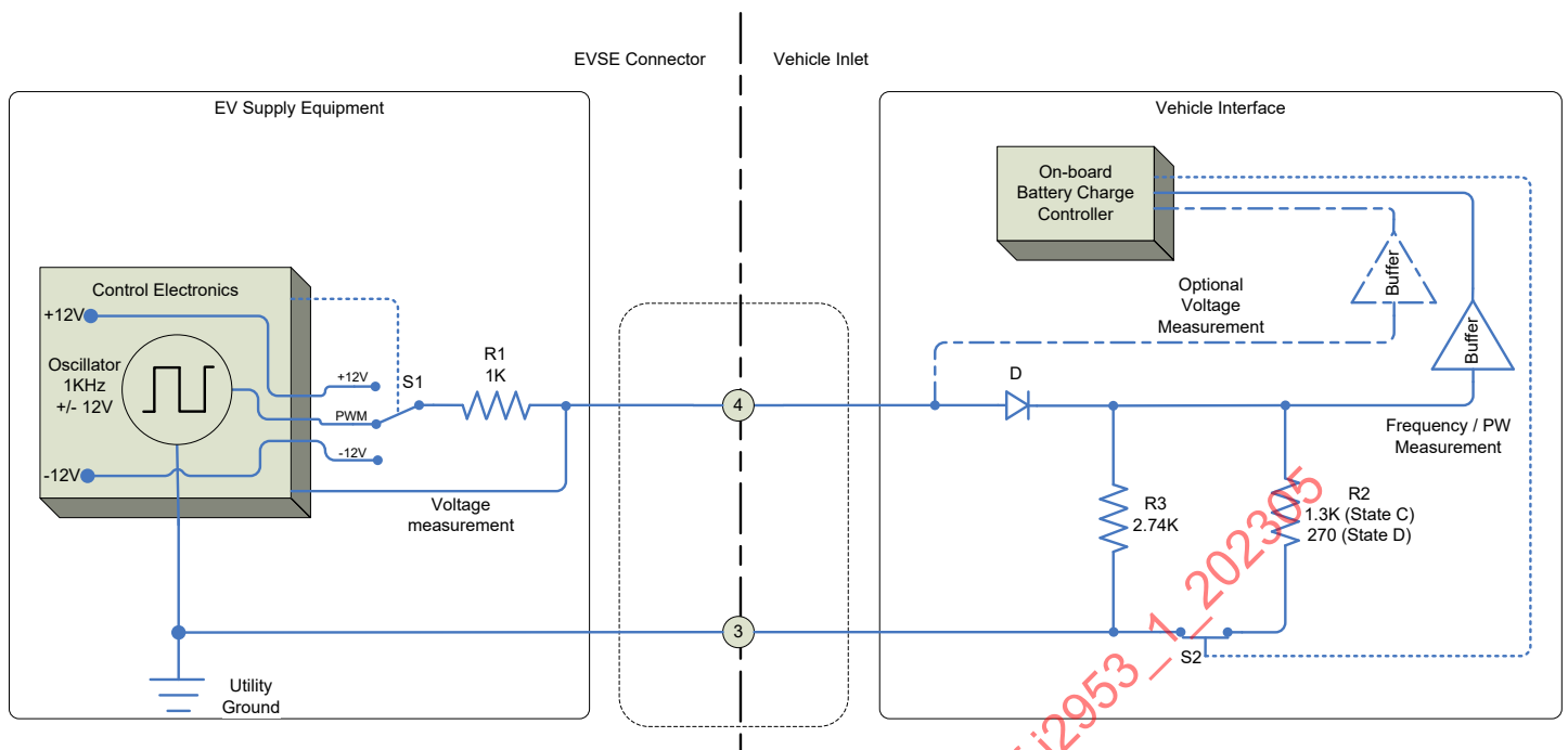
FIGURE 4.3 - AC LEVEL 1 AND AC LEVEL 2 CONTROL PILOT CIRCUIT
