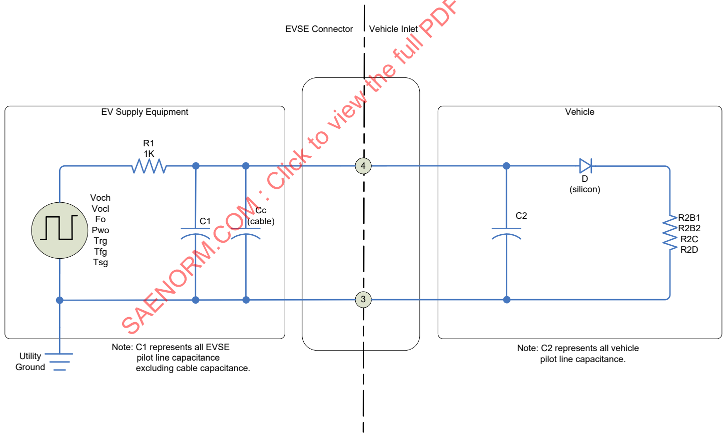
FIGURE A.1 - CONTROL PILOT EQUIVALENT CIRCUIT
