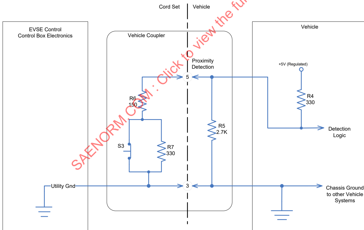
FIGURE 4.4 - AC LEVEL 1 AND AC LEVEL 2 PROXIMITY CIRCUIT
