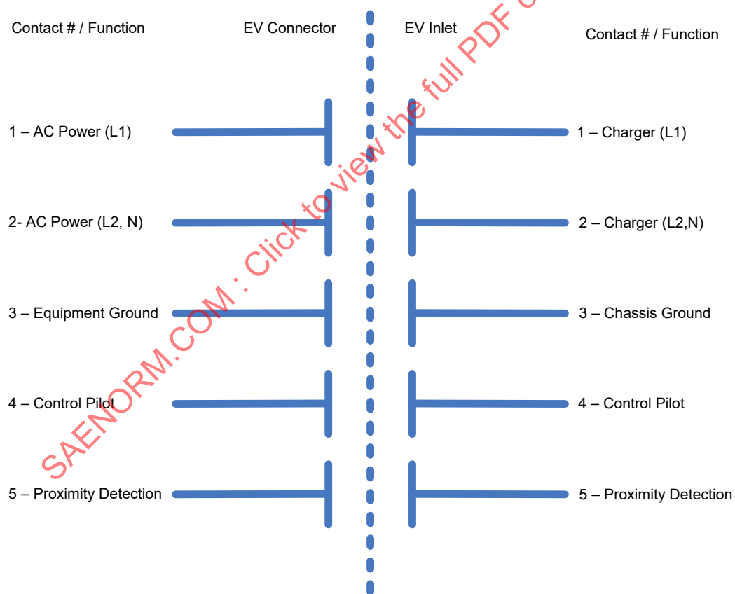
FIGURE 4.2 - AC LEVEL 1 AND AC LEVEL 2 CONDUCTIVE COUPLER CONTACT INTERFACE FUNCTIONS
