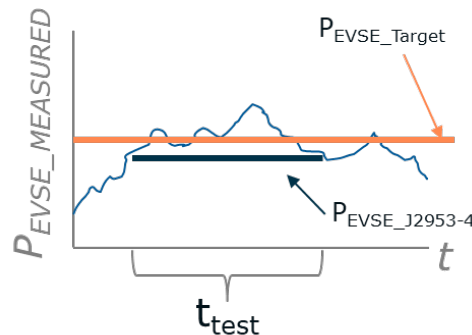
Figure 2 Example identification of SAE J2953-4 EVSE Power during varying charge power
