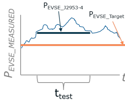
Figure 3 Example identification of SAE J2953-4 EVSE Power for higher than expected values
