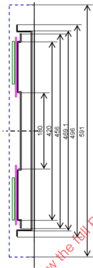
Figure G2 - Mechanical dimensions of the GA WPT1
