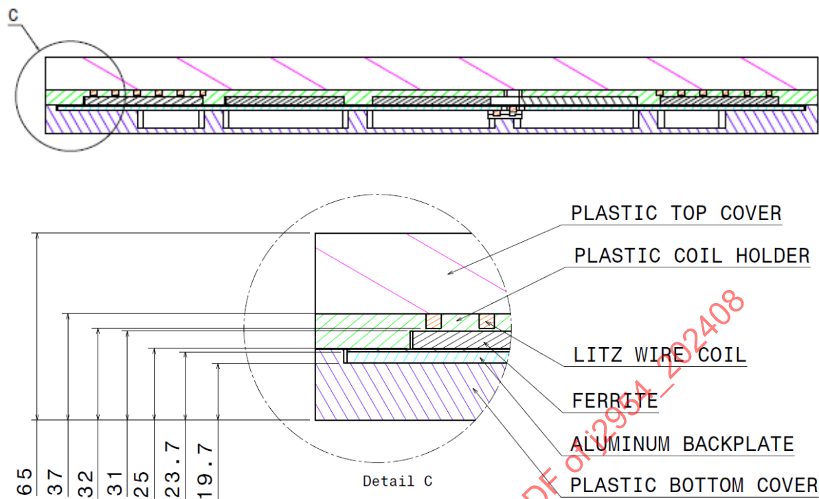
Figure I2 - Detailed cross-section view of the Product GA WPT2
