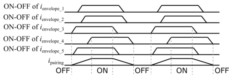
Figure C10 - Example of ON-OFF determination of i_{\text{pairing}}
