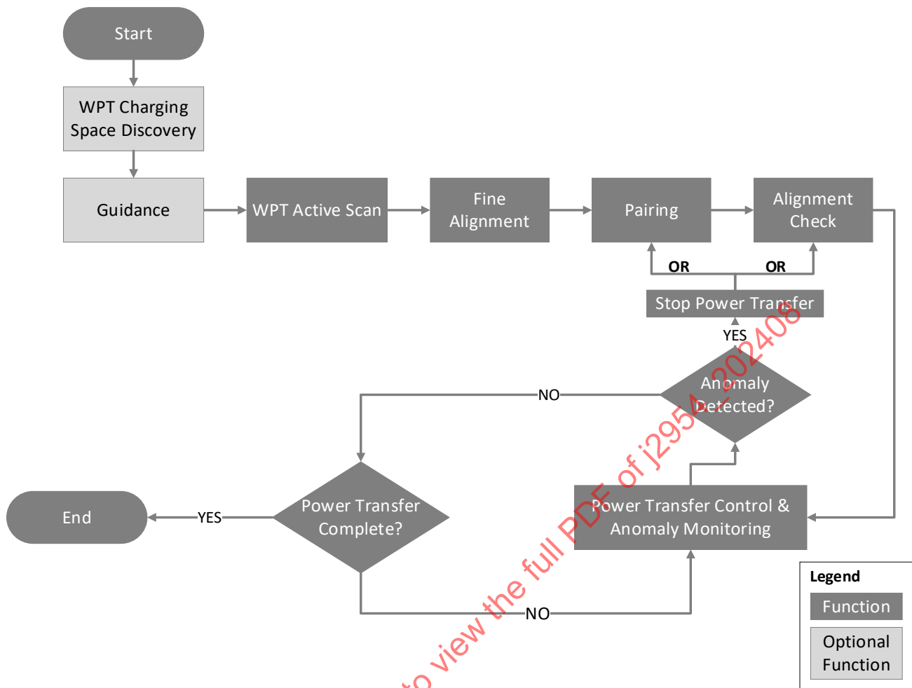
Figure 20 - Wireless charging process flow diagram
