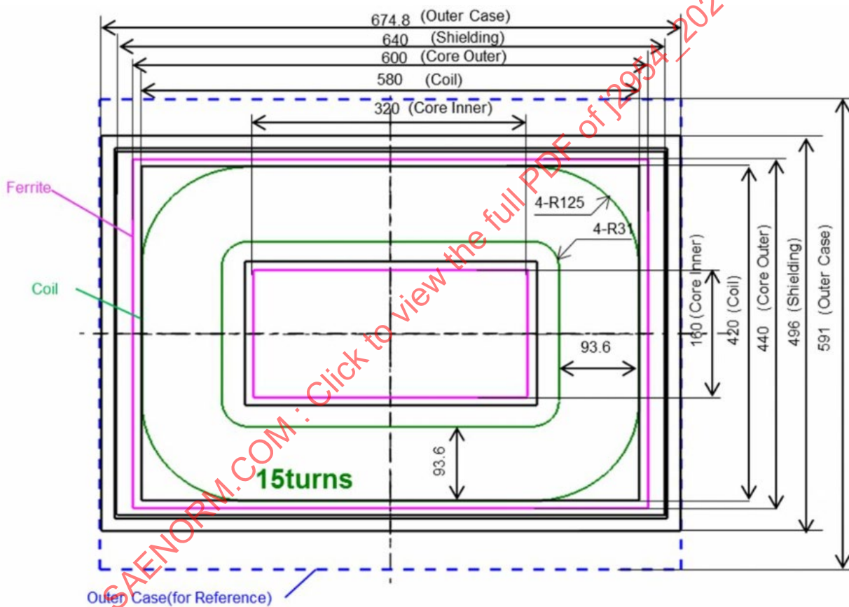
Figure G1 - Mechanical dimensions of the GA WPT1
