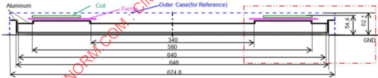
Figure G3 - Mechanical dimensions of the GA WPT1
