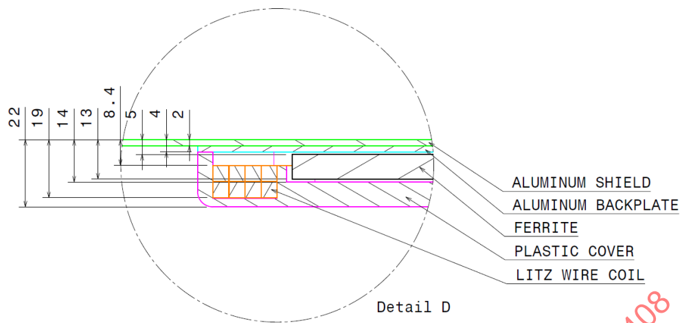
Figure H5 - Detailed cross-section view of the Product VA WPT2/Z2
