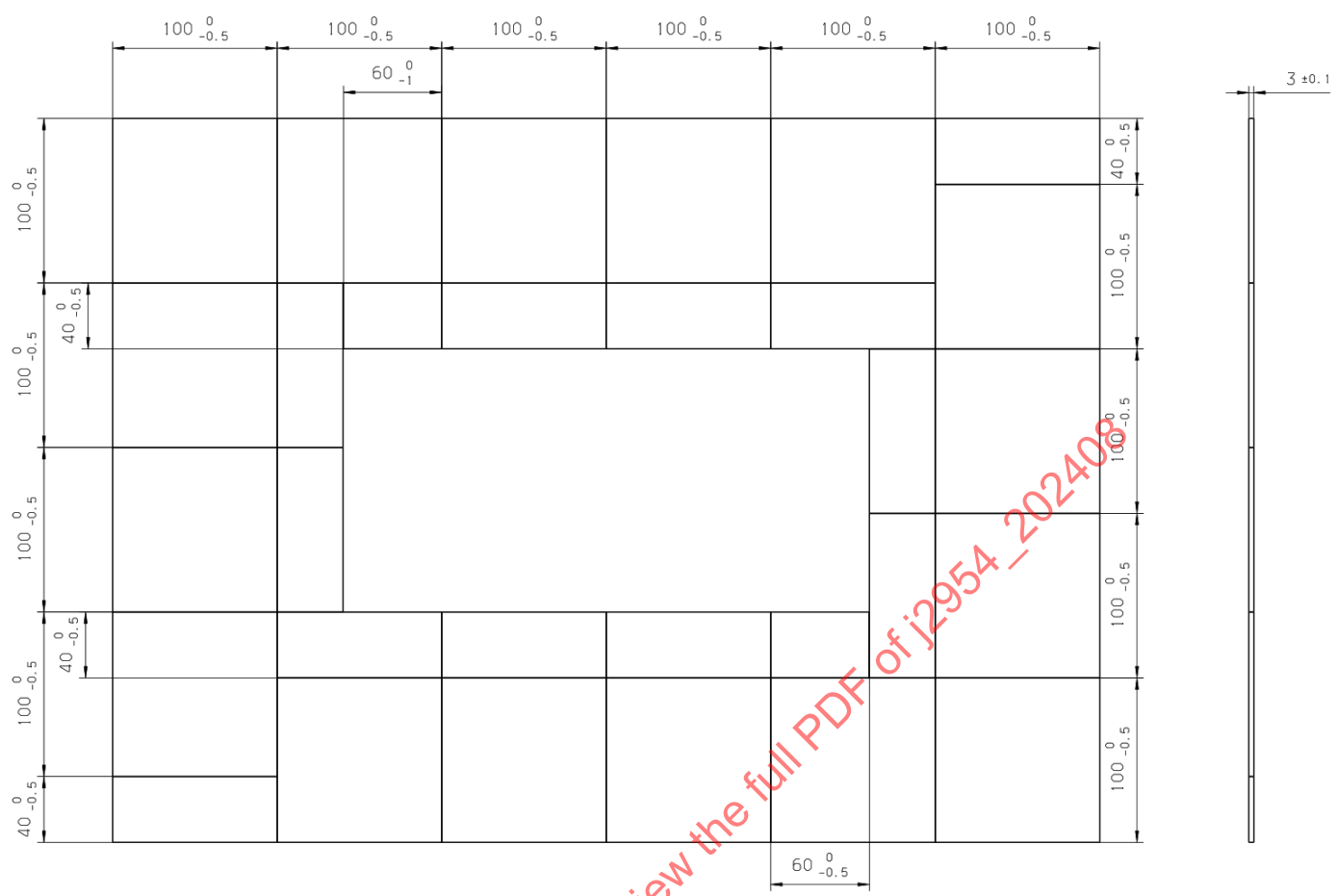
Figure G5 - Detail of the ferrite core construction
