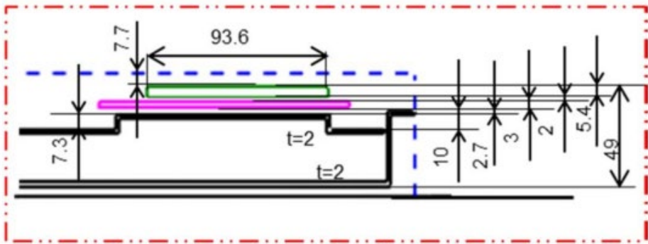
Figure G4 - Detailed cross-section view
