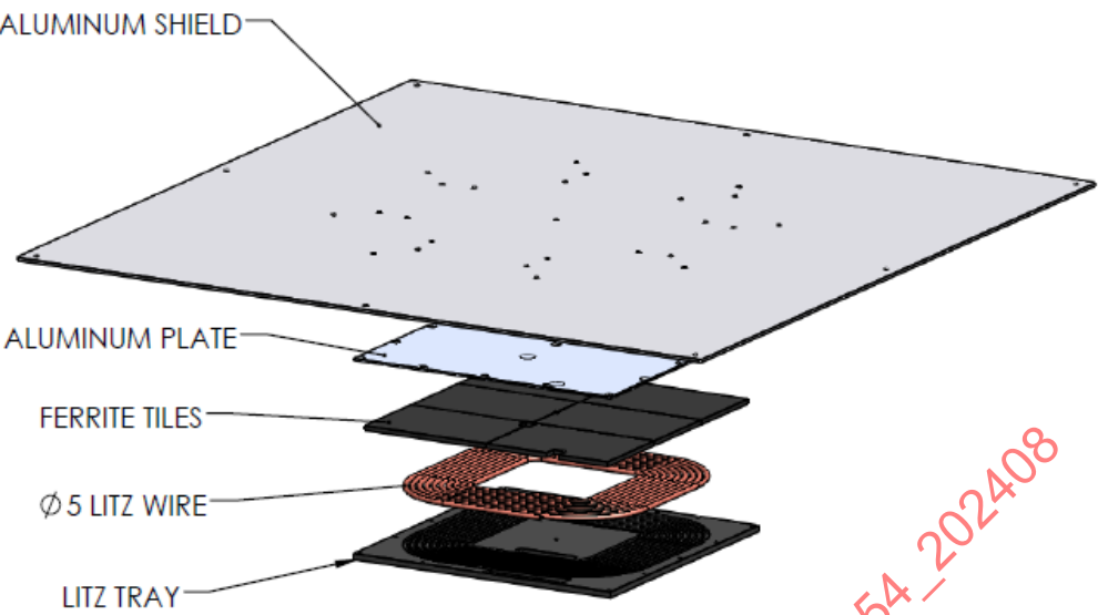
Figure A26 - Exploded view of the Test Station VA WPT3/Z1
