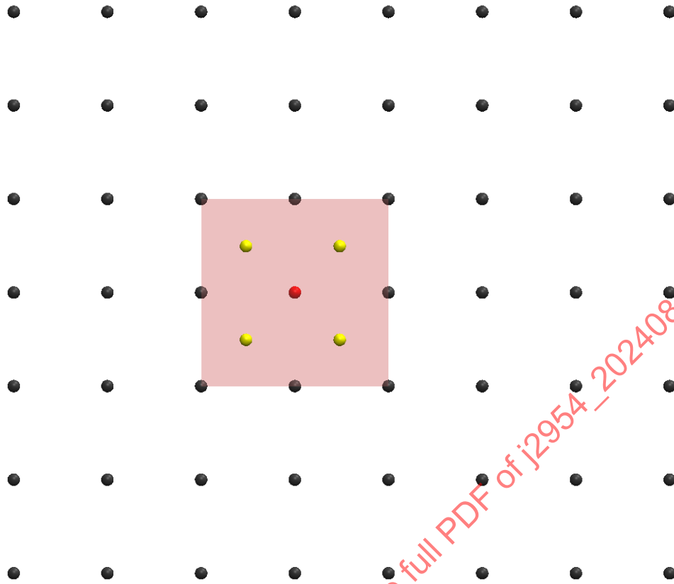
Figure 16 - Region for reference level average measurement - 2 x 2 grid with light color points indicate points of measurement centered around peak
