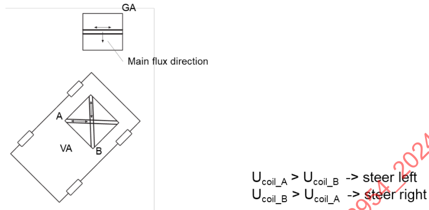
Figure D2 - Differential evaluation of the magnetic field
