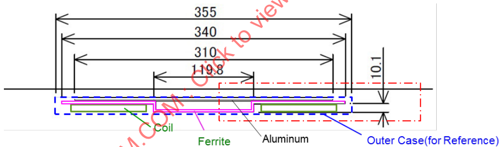
Figure A7 - Mechanical dimensions of the Test Station VA WPT1/Z2
