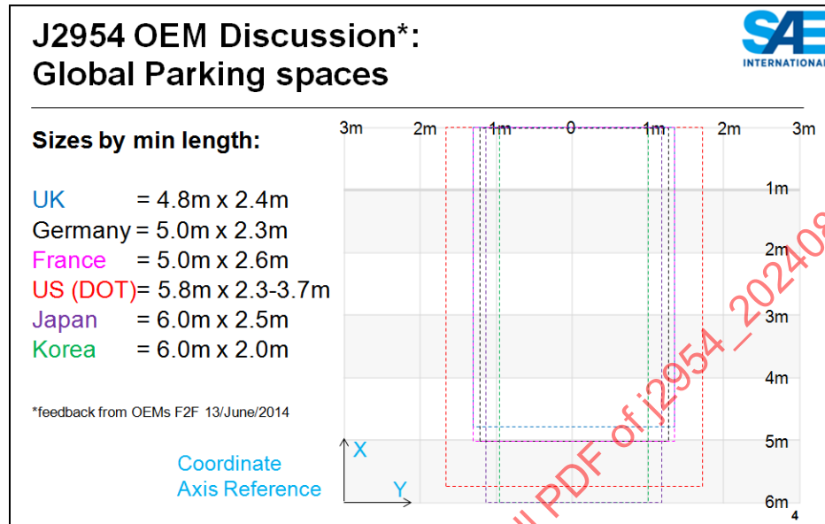
Figure F1 - SAE J2954 OEM survey for GA location in parking space
