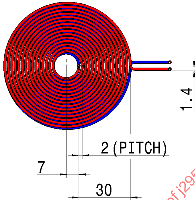
Figure C13 - Mechanical dimensions of a vertical field coil in the example GA
