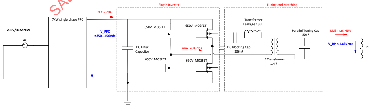
Figure I3 - Electrical specification of the Product GA WPT2
