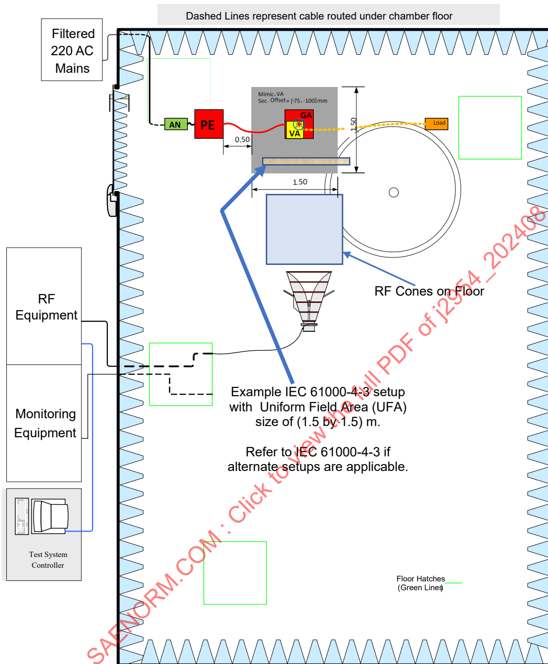
Figure 7 - Example of RI ALSE test setup for component-level wireless charging system (top view)
