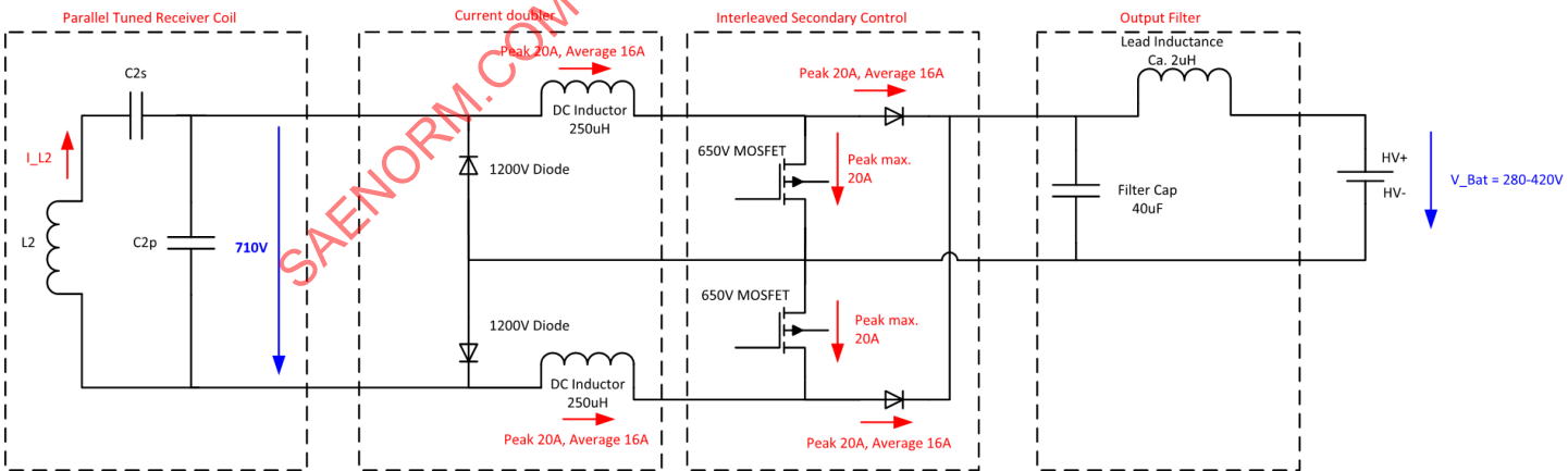
Figure H12 - Electrical specification of the Product VA WPT3/Z1
