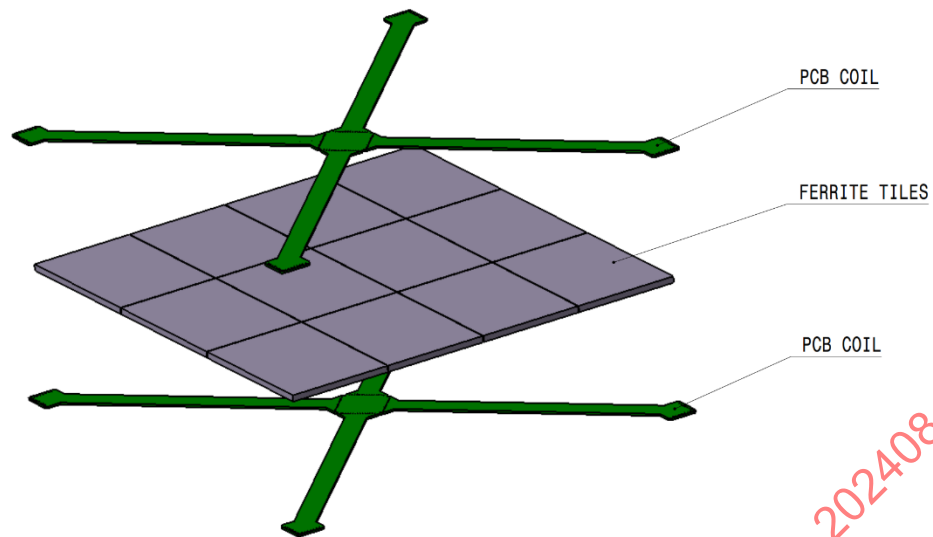
Figure C1 - Exploded view of the Test Device
