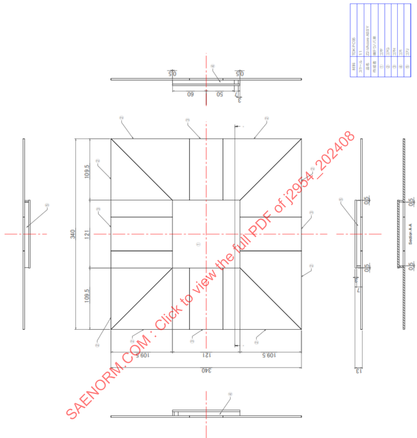
Figure A9 - Detail of the ferrite core construction
