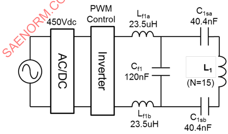
Figure G6 - Electrical specification of the GA WPT1
