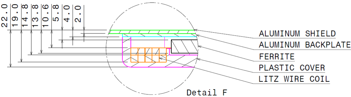
Figure H2 - Detailed cross-section view of the Product VA WPT2/Z1
