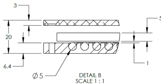
Figure A16 - Mechanical dimensions of the Test Station VA WPT2/Z1
