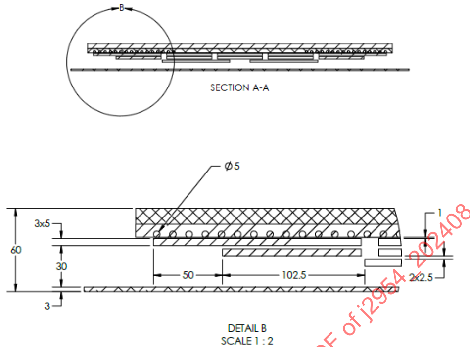
Figure B2 - Detailed cross-section view of the Test Station Universal GA
