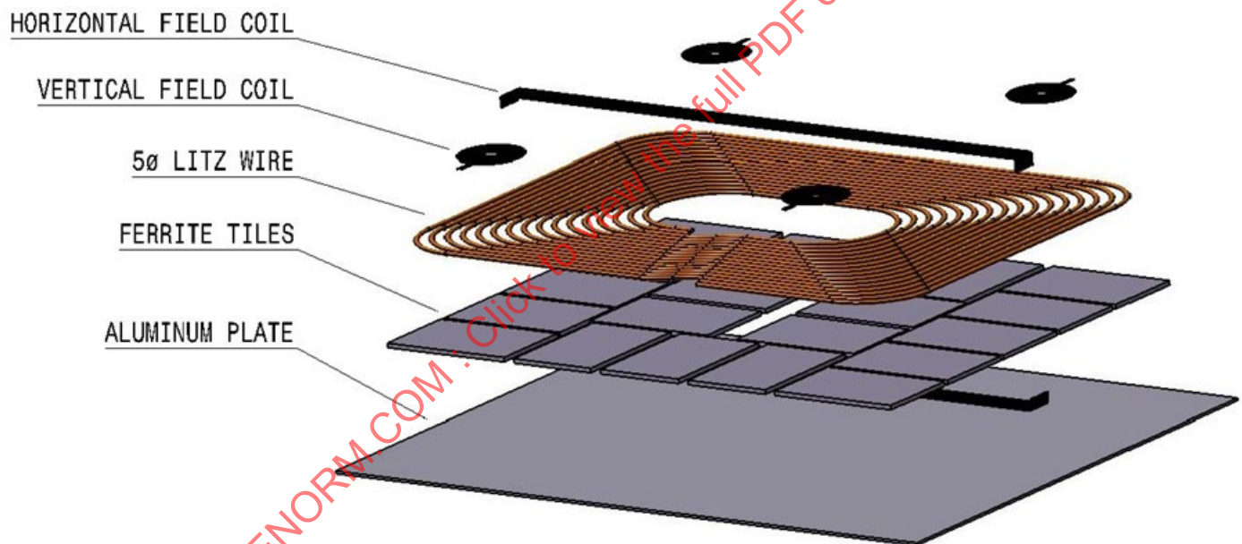
Figure 22 - Exploded view of an example of a DIPS-Enabled GA
