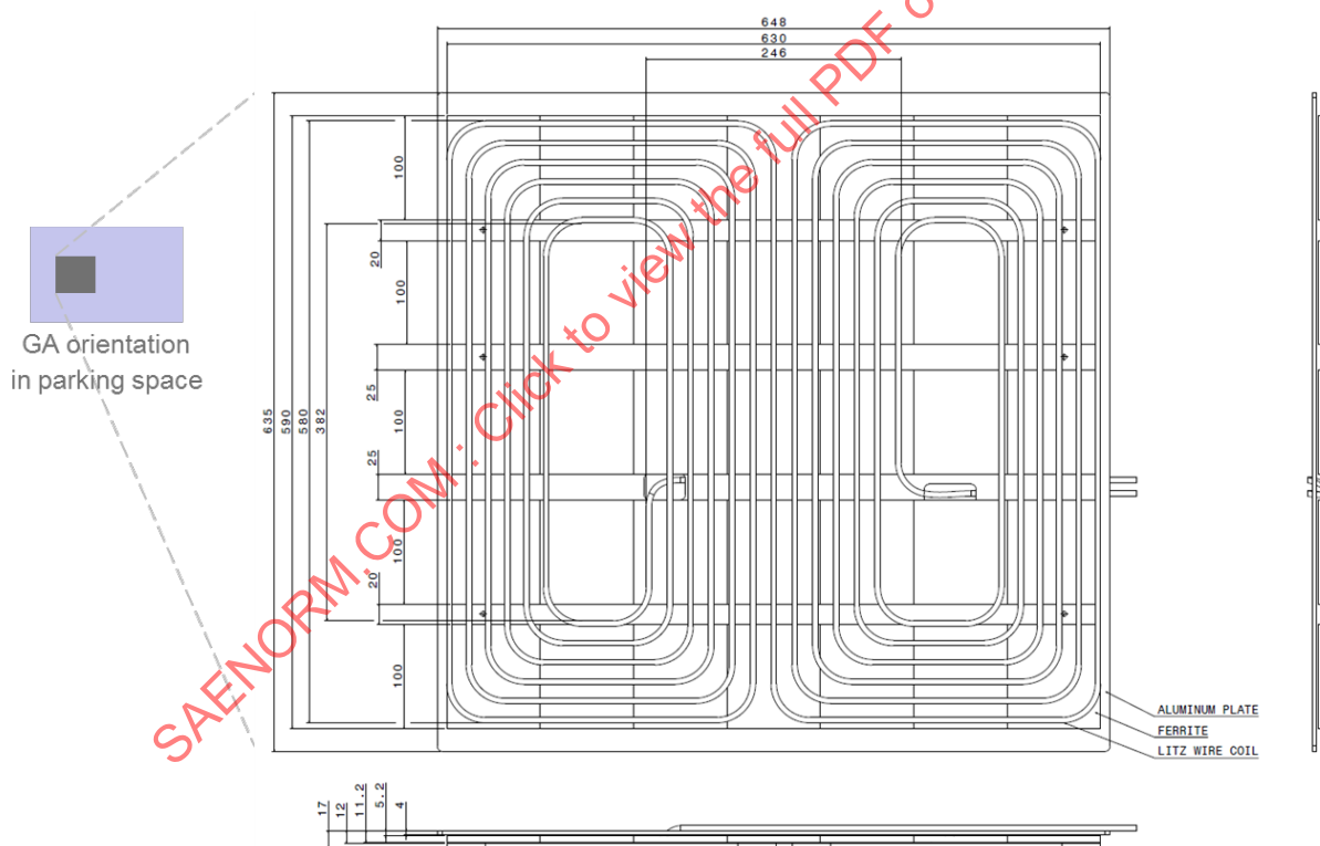
Figure I1 - Mechanical dimensions of the Product GA WPT2
