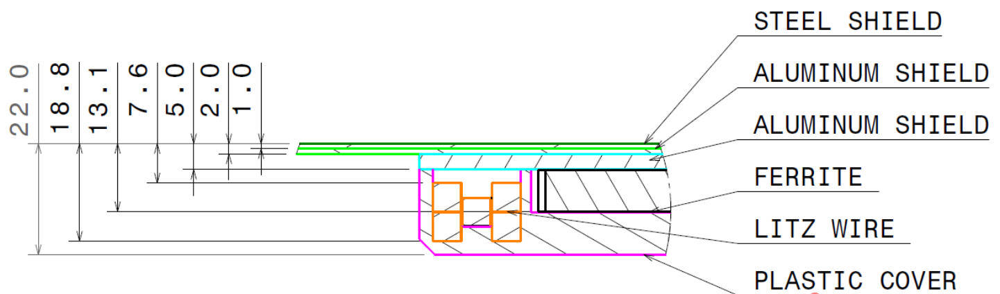
Figure H11 - Detailed cross-section view of the Product VA WPT3/Z1
