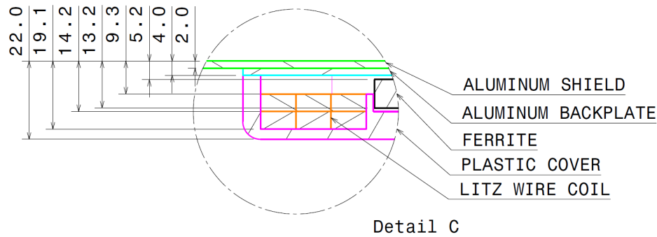
Figure H8 - Detailed cross-section view of the Product VA WPT2/Z3
