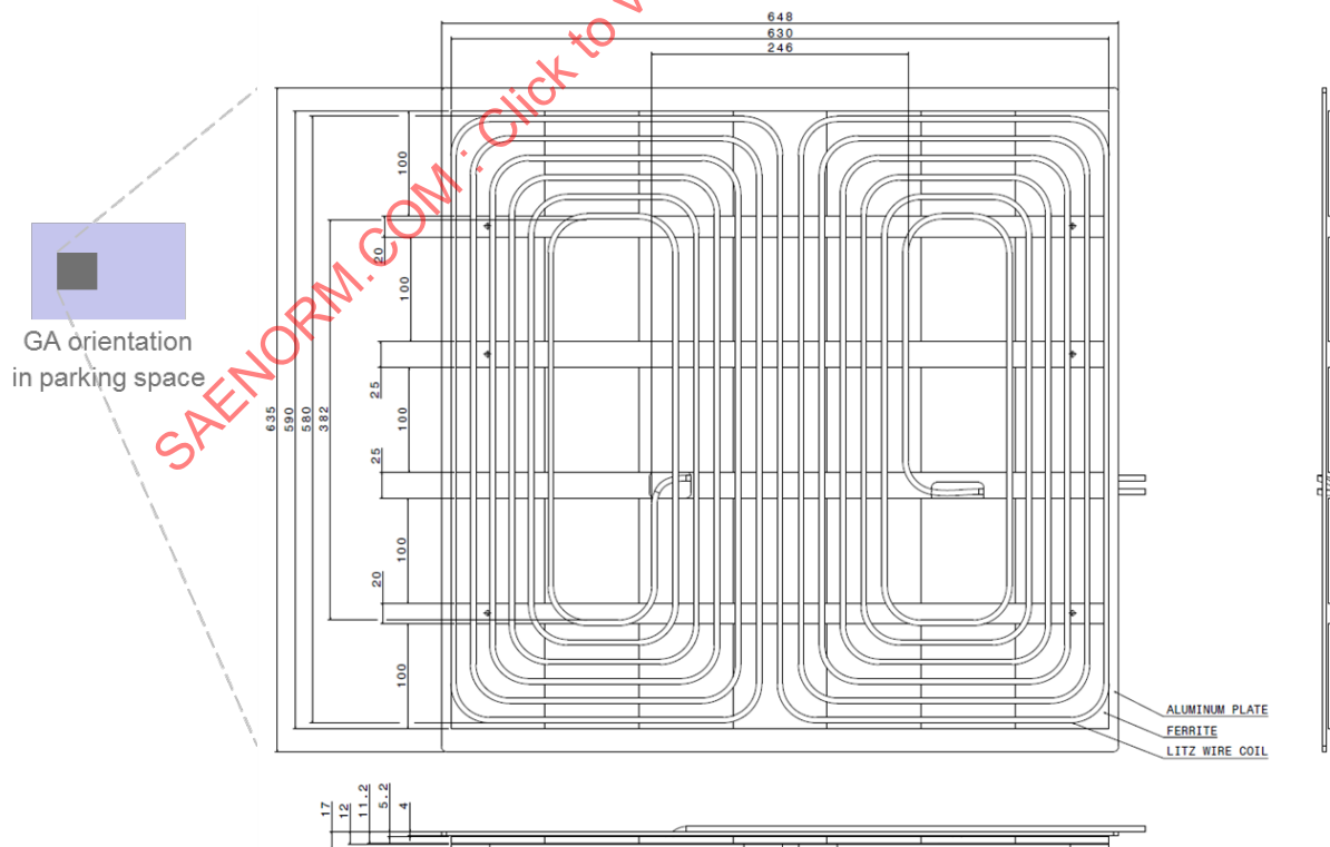
Figure I4 - Mechanical dimensions of the Product GA WPT3
