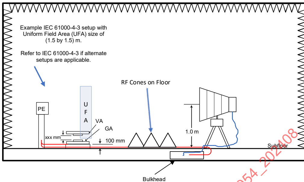
Figure 8 - Example of RI ALSE test setup for component-level wireless charging system (side view)
