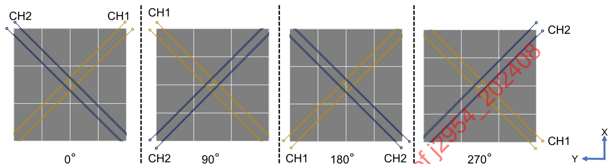
Figure C3 - Definition of the orientation of the DIPS Test Device
