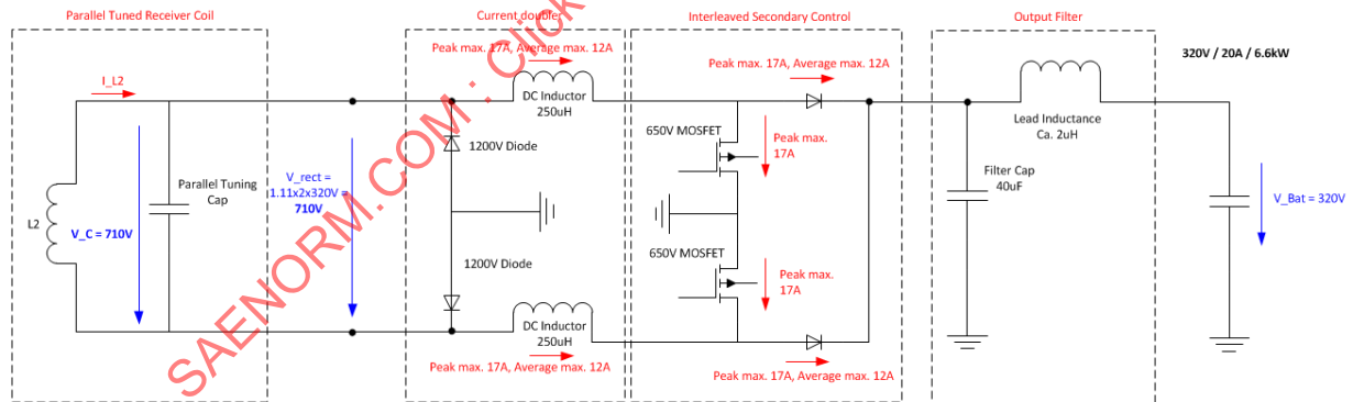
Figure H9 - Electrical specification of the Product VA WPT2/Z3
