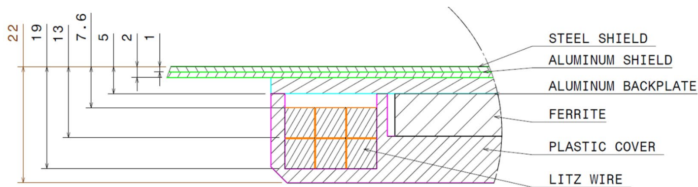
Figure H17 - Detailed cross-section view of the Product VA WPT3/Z3
