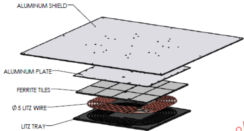
Figure A32 - Exploded view of the Test Station VA WPT3/Z3
