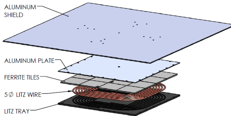
Figure A23 - Exploded view of the Test Station VA WPT2/Z3
