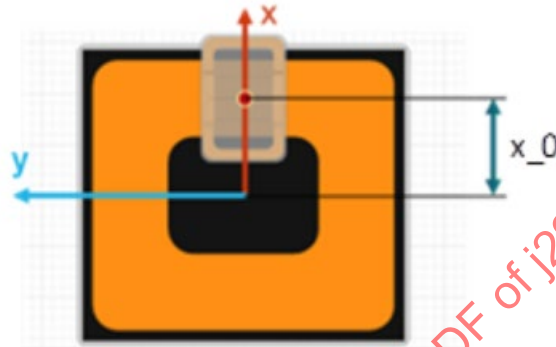
Figure 23 - Example for the “natural offset” definition x_0 for a DD-topology VA over a circular-topology GA
