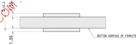
DETAIL B
