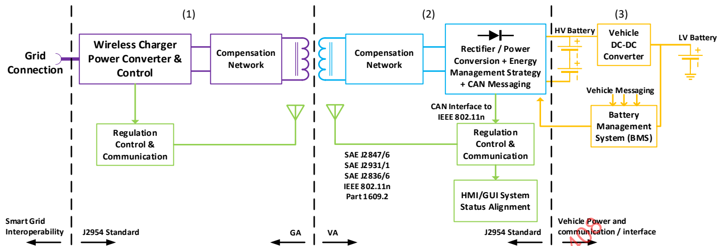
Figure 4 - Typical functional elements of a wireless charging system (WCS)
