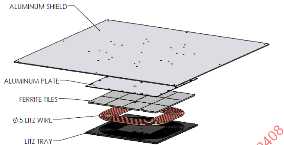
Figure A29 - Exploded view of the Test Station VA WPT3/Z2
