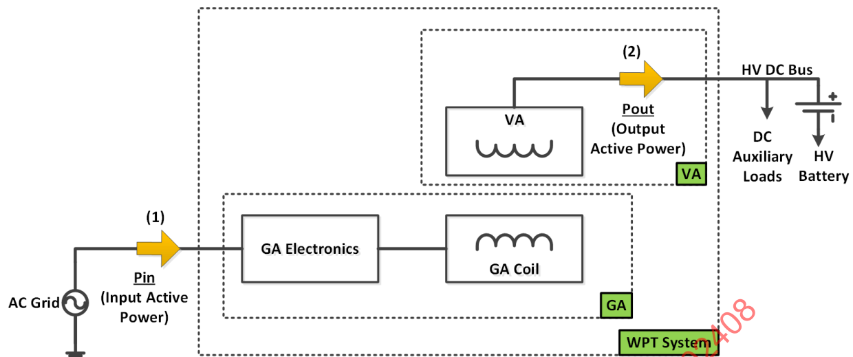
Figure 29 - Block diagram of a WPT system (including VA and GA) illustrating the efficiency points (1) and (2)
