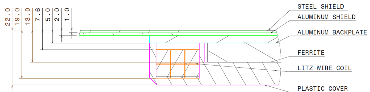
Figure H14 - Detailed cross-section view of the Product VA WPT3/Z2
