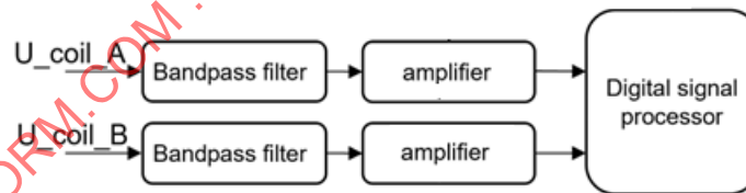
Figure D3 - Example of VA signal processing
