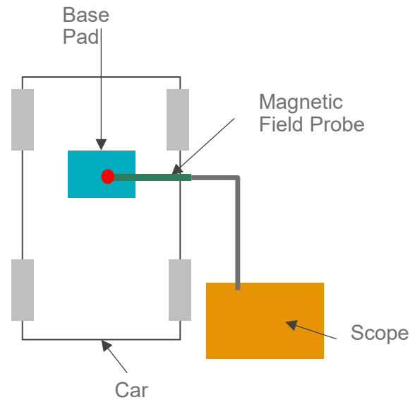
Figure E1 - Test measurement setup for LOP
