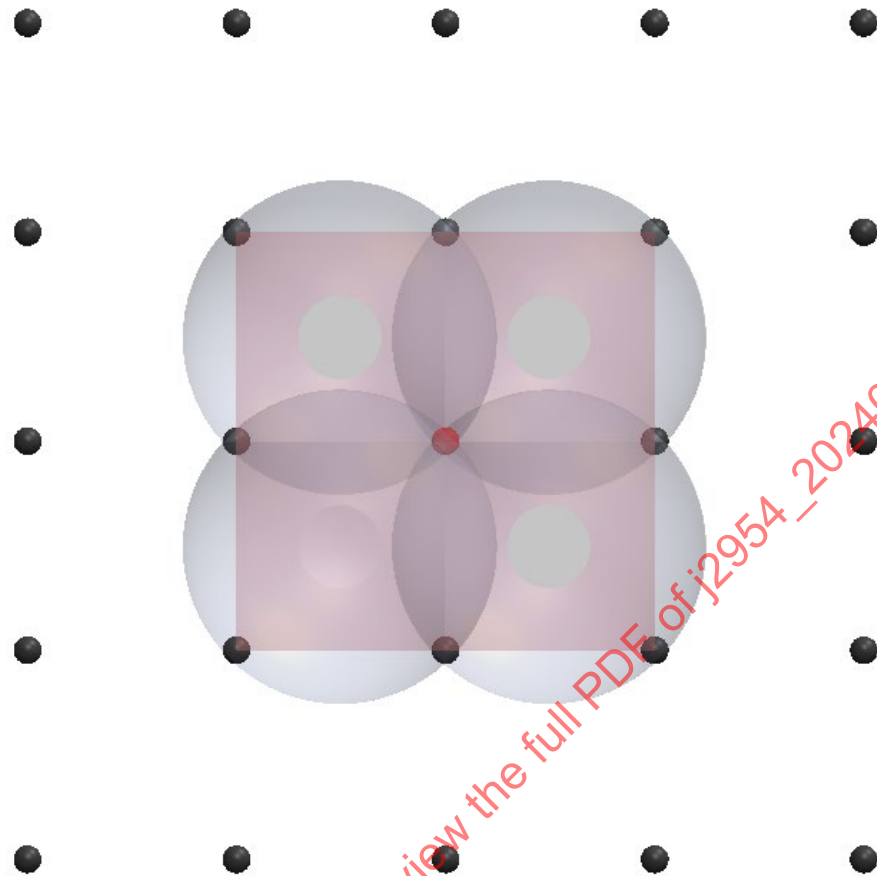
Figure 17 - Locations for standard field probe averages around peak - 2 x 2 grid separated equidistantly by 7.5 cm center-to-center
