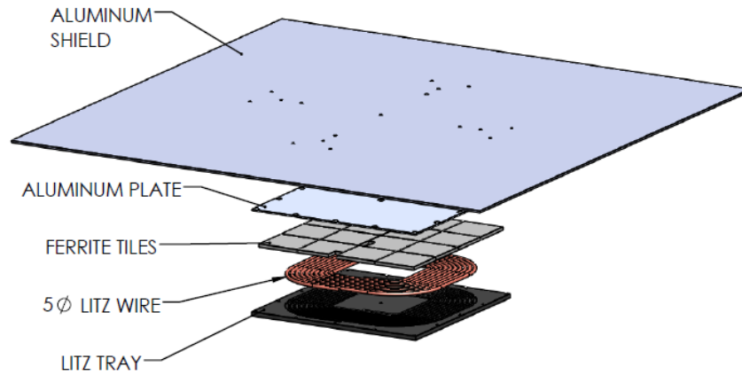
Figure A17 - Exploded view of the Test Station VA WPT2/Z1
