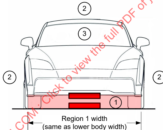
Figure 13 - EMF regions, front view
