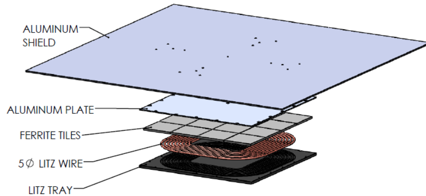
Figure A20 - Exploded view of the Test Station VA WPT2/Z2
