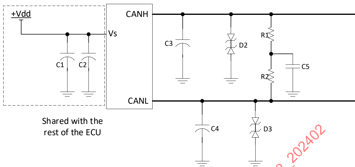
Figure 5 - Monitoring DUT with Vdd supply
