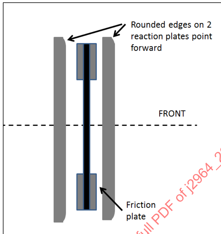
Figure B3 - Plate orientation in test head
