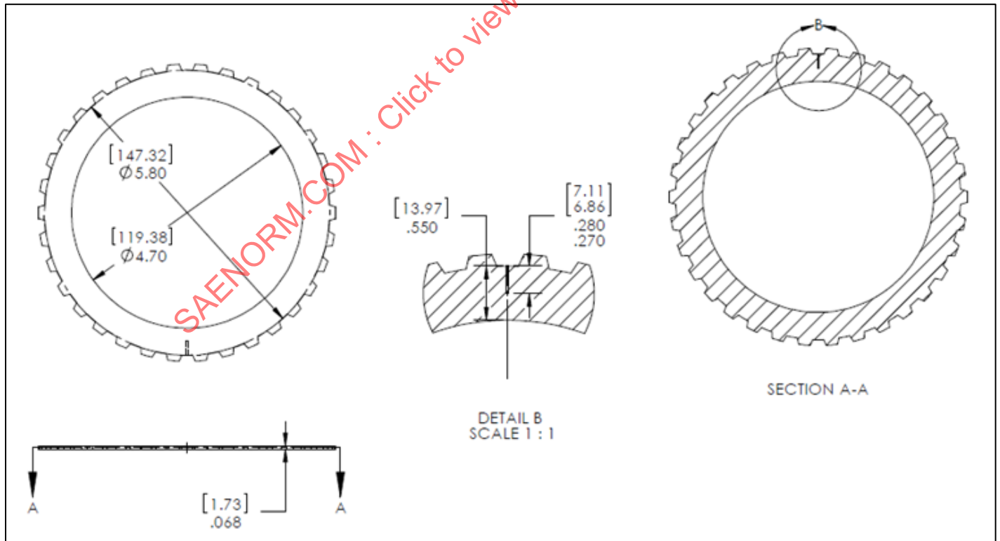
Figure B2 - Detail of thermocouple hole in the reaction plate
