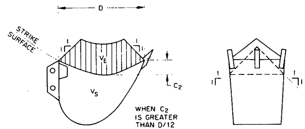
FIG. 2—BUCKET CAPACITY, TYPE B
