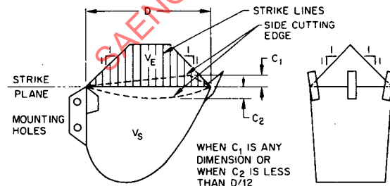
FIG. 1—BUCKET CAPACITY, TYPE A
