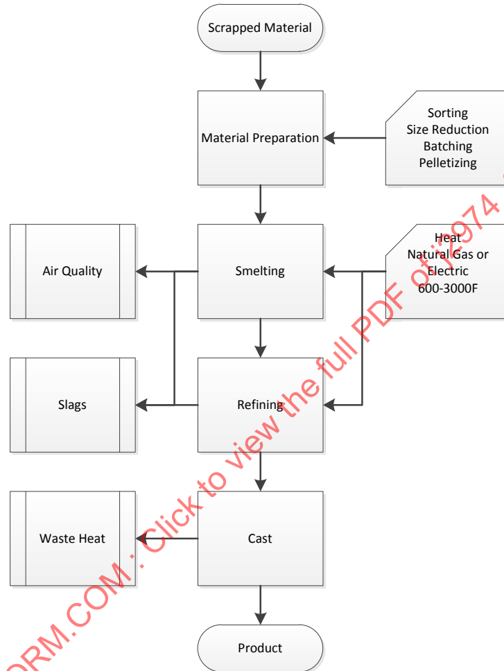
Figure 2 - Pyrometallurgical processing
