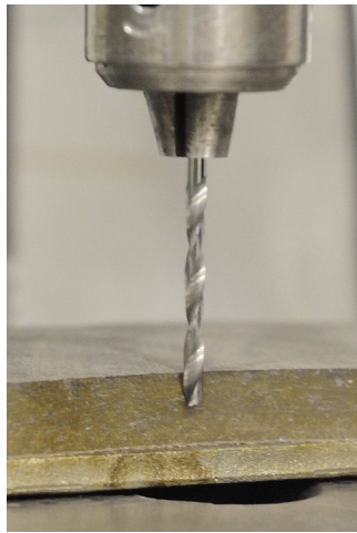
Figure 2 - Setting the drill press stop at \frac{1}{2} the friction material thickness
