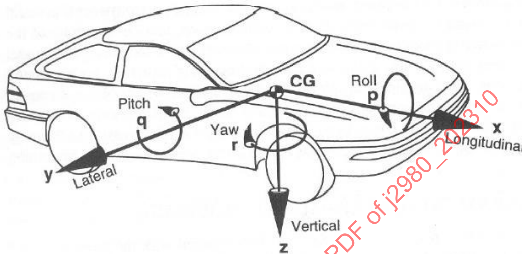
Figure A1 - Vehicle motion axes Source: SAE Vehicle Axis Reference
