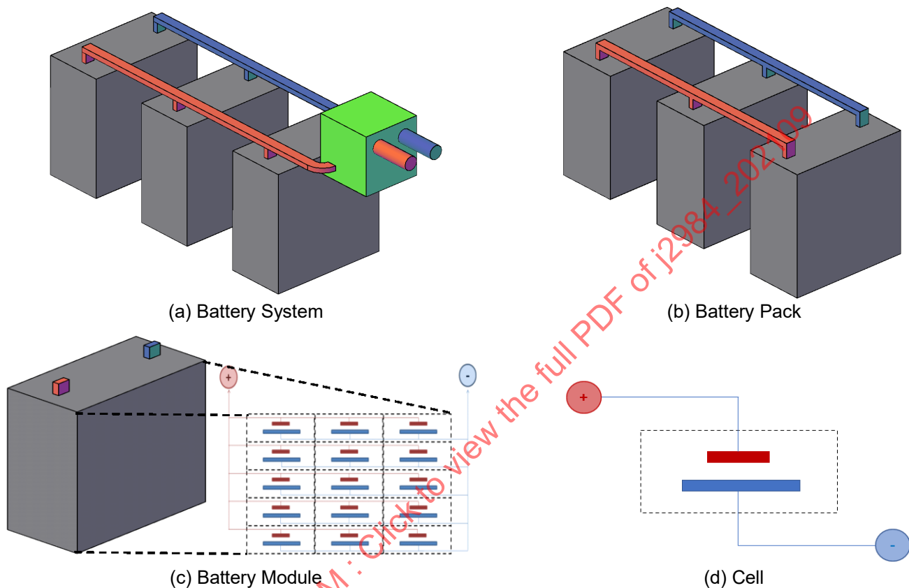
Figure 1 - Schematics of battery terminology for (a) battery system, (b) battery pack, (c) battery module, (d) cell
