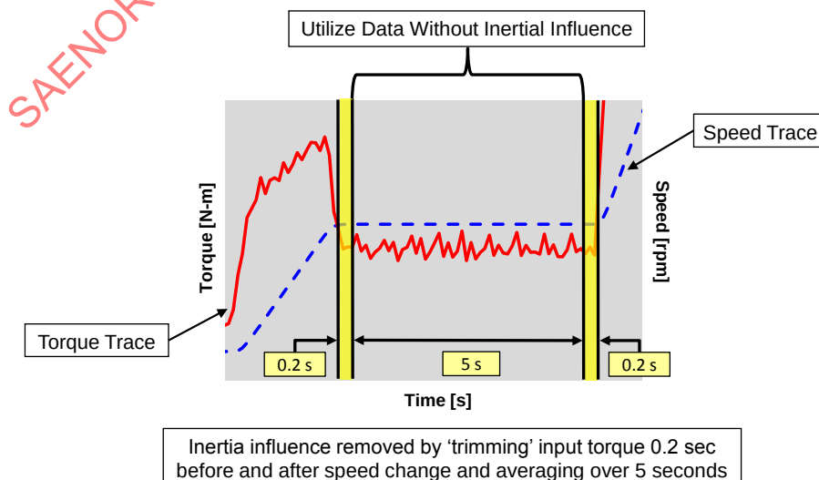
FIGURE 8 - INERTIA INFLUENCE
