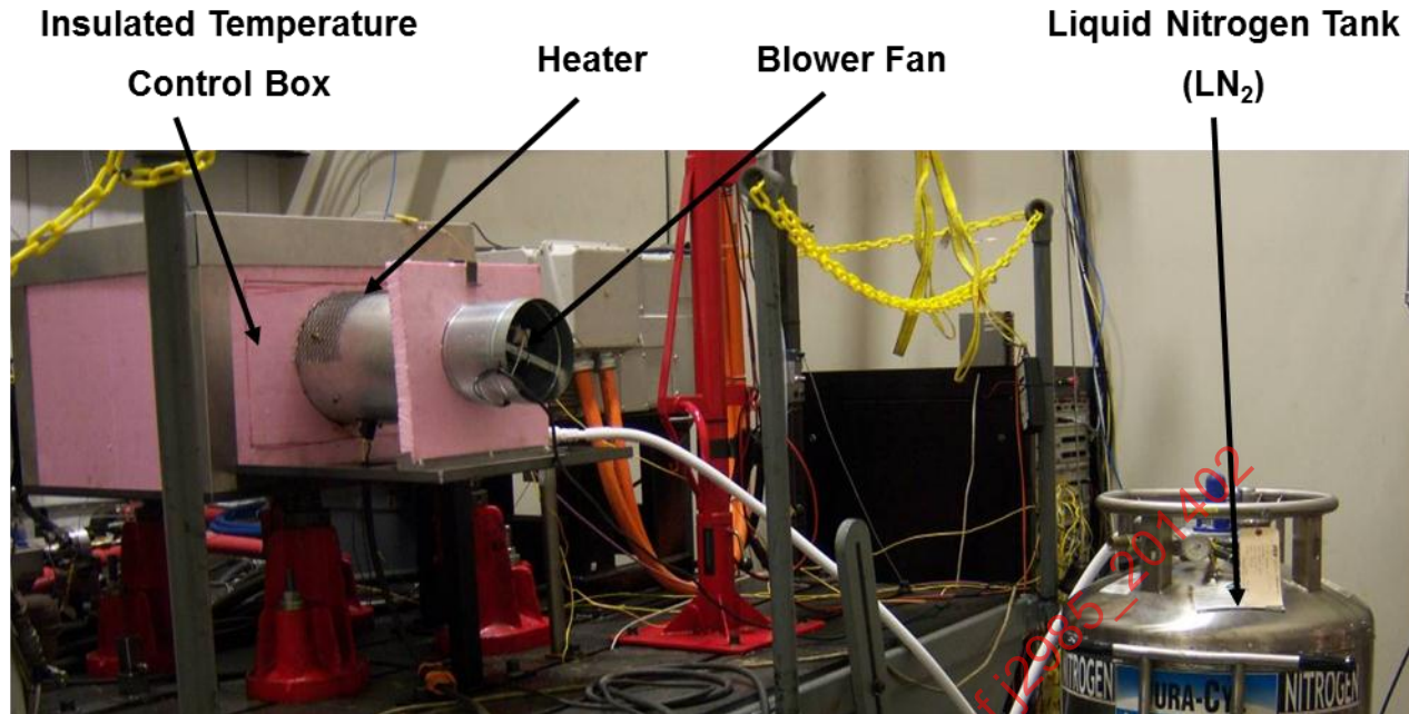
FIGURE 5 - PHOTOGRAPH OF TEMPERATURE CONTROLLED CHAMBER
