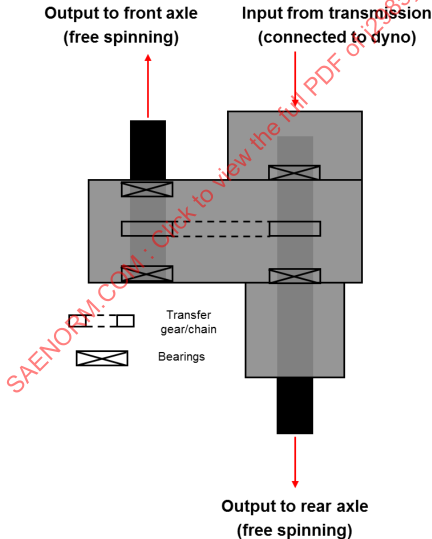
FIGURE 1 - TRANSFER CASE SCHEMATIC (SHOWN WITH REFERENCES TO VEHICLE POSITION)
