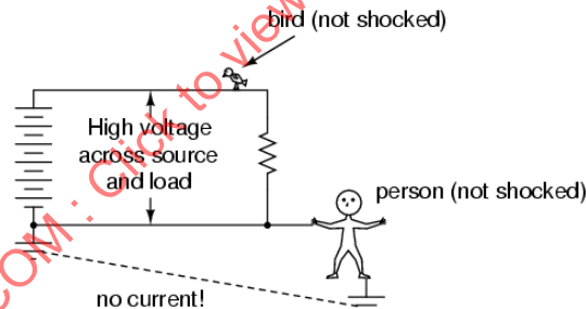
Figure 1 - Single point contact
