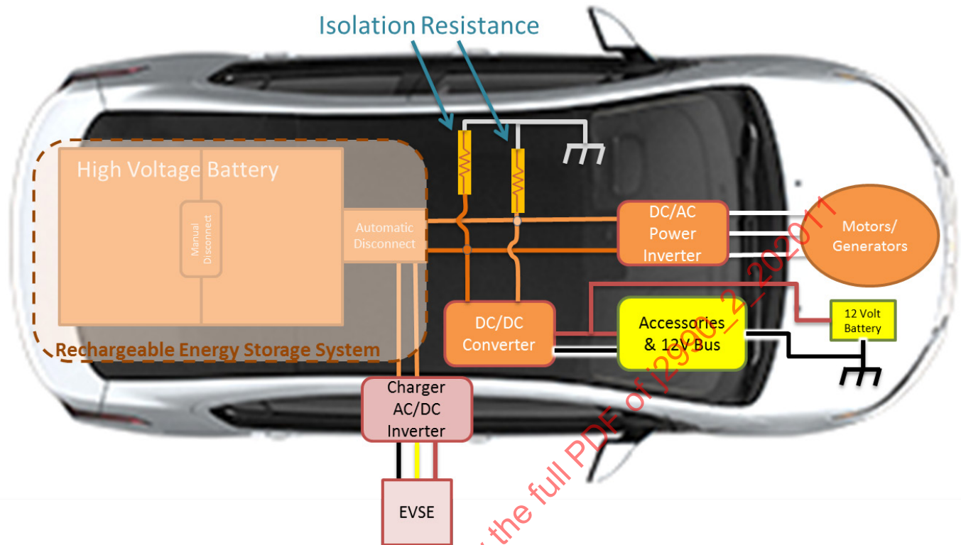
Figure 3 - Typical xEV high voltage system
