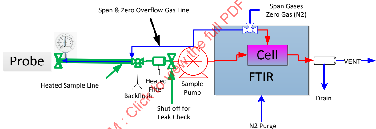
Figure 7 - Leak test with pump upstream of the analyzer
