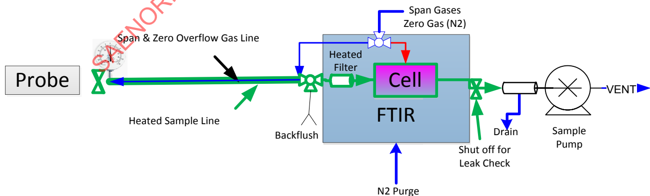
Figure 8 - Leak test with pump downstream of the analyzer
