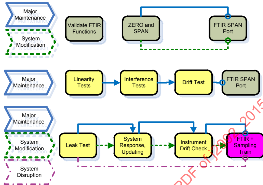
Figure 5 - Test requirements after major maintenance, system modification or system disruption
