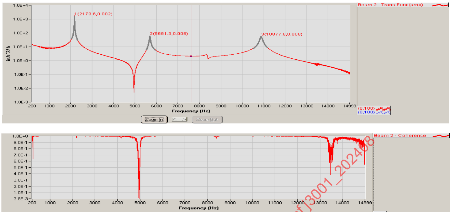
Figure 3 - Example of an FRF (top) and coherence function (bottom)
