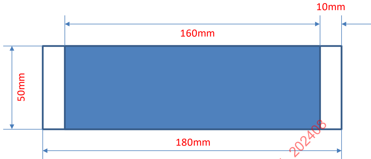
Figure 1 - Steel plate dimensions and insulator location
