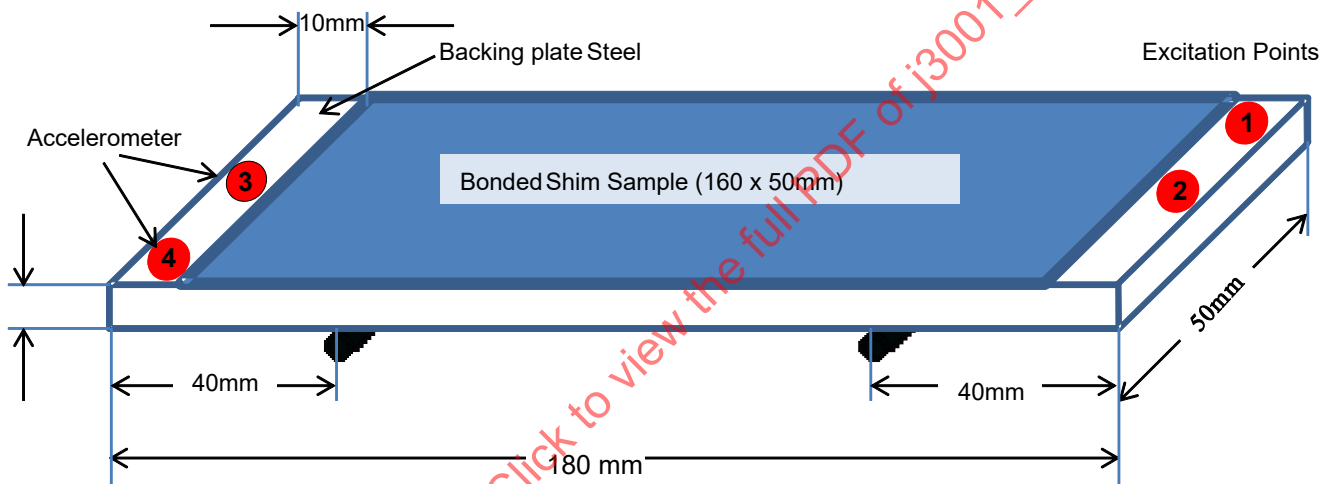
Figure 2 - Location of rubber mounts and excitation/measurement points
