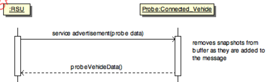
FIGURE 13 - EXCHANGE PROBE VEHICLE DATA DIALOG
