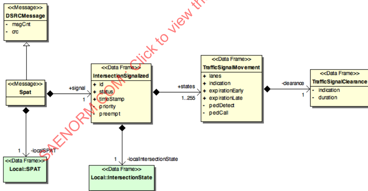
FIGURE 41 - DATA MODEL - sPAT
