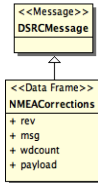
FIGURE 39 - DATA MODEL - nMEACorrections
