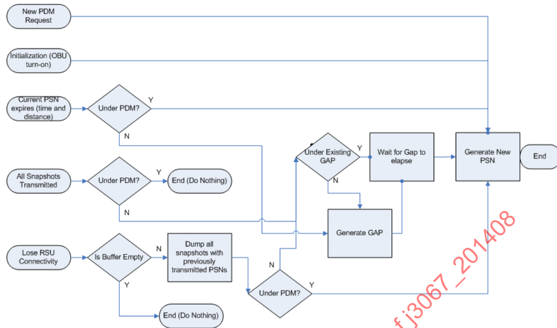
FIGURE 22 - PROBE DATA MESSAGES - PSN
