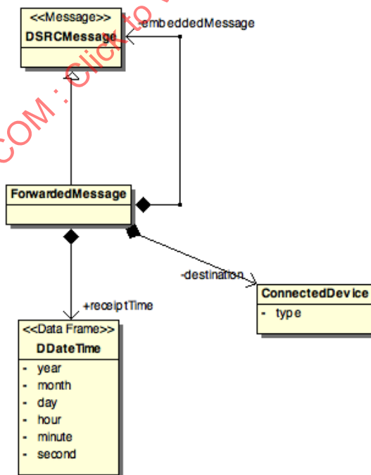
FIGURE 35 - DATA MODEL - forwardedMessage
