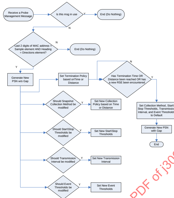
FIGURE 17 - PROBE DATA MANAGEMENT MESSAGE
