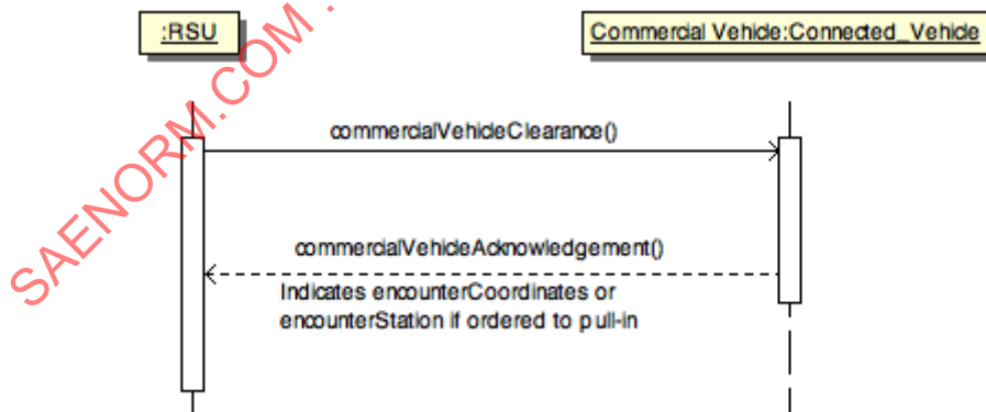
FIGURE 12 - EXCHANGE VEHICLE CLEARANCE DIALOG
