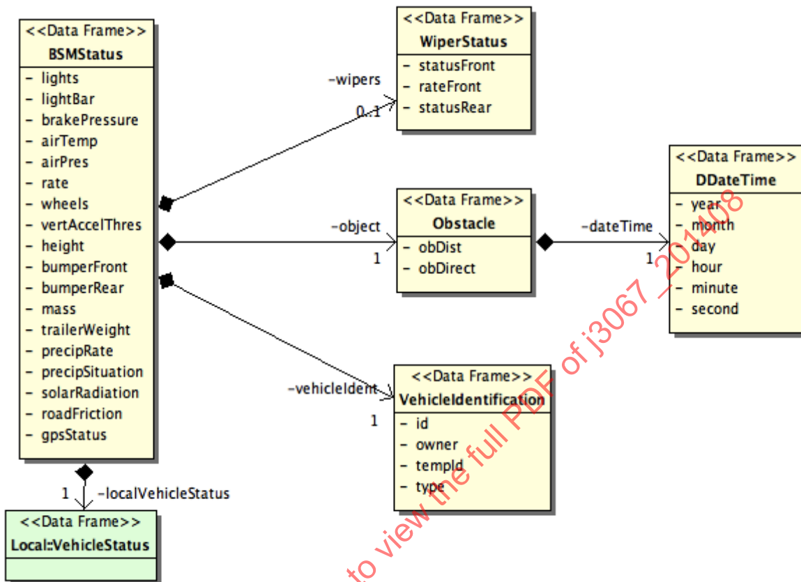
FIGURE 26 - DATA MODEL - bSMStatus
