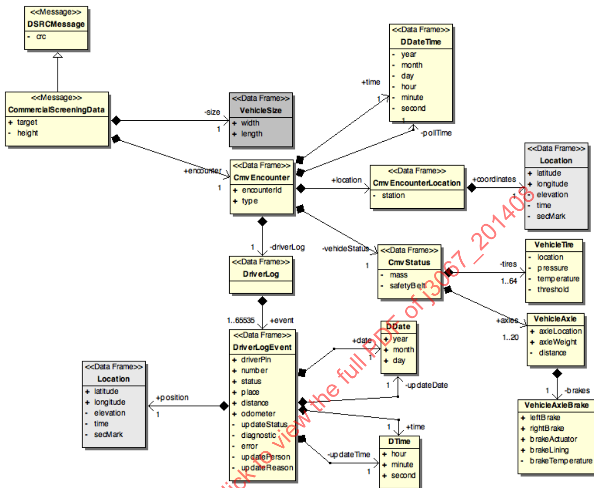
FIGURE 28- DATA MODEL - commercialScreeningData
