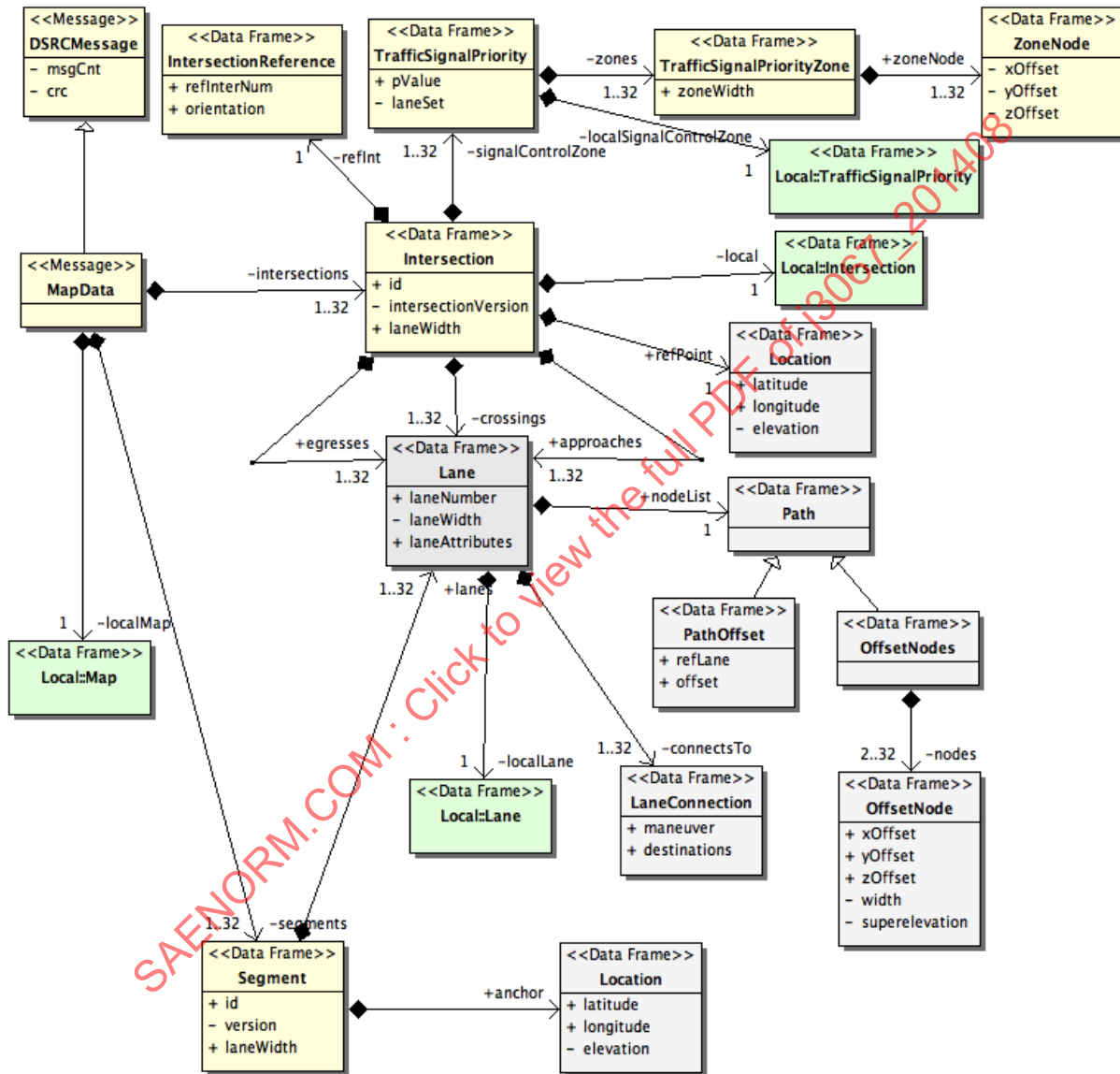
FIGURE 37 - DATA MODEL - mapData
