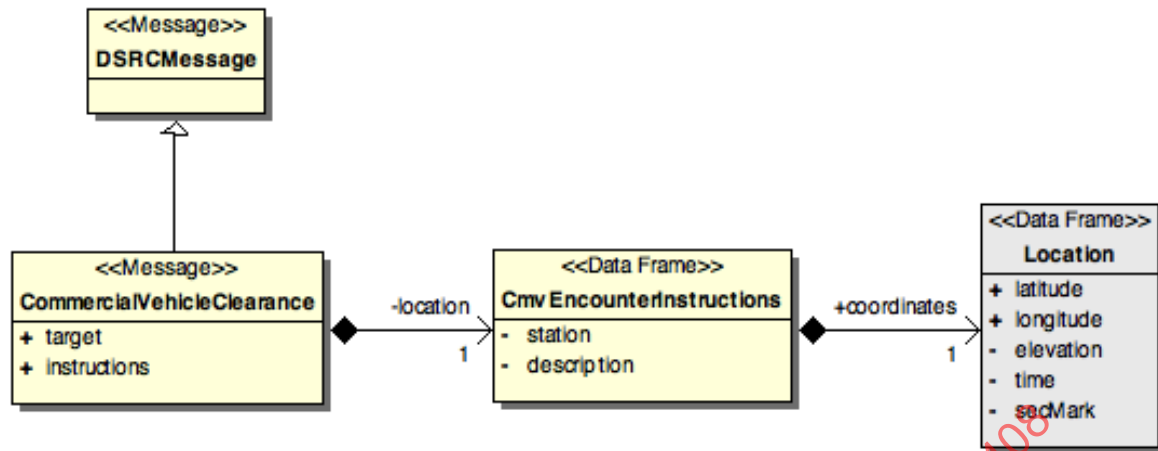
FIGURE 31 - DATA MODEL - commercialVehicleClearance
