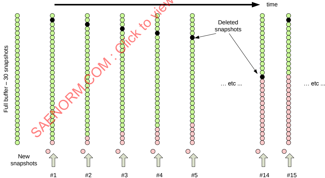
FIGURE 20 - CONNECTED VEHICLE - BUFFER OVERFLOW STATE - DELETING SNAPSHOTS
