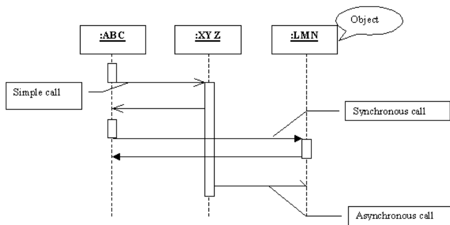
FIGURE 4 - PARTS OF A UML SEQUENCE DIAGRAM
