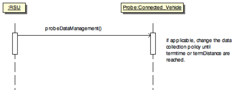
FIGURE 16 - PROBE DATA MANAGEMENT DIALOG
