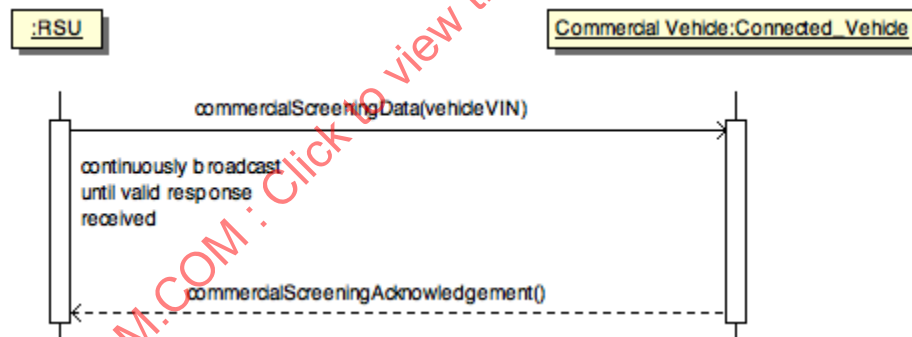
FIGURE 10 - EXCHANGE COMMERCIAL VEHICLE SCREENING RESULTS DIALOG
