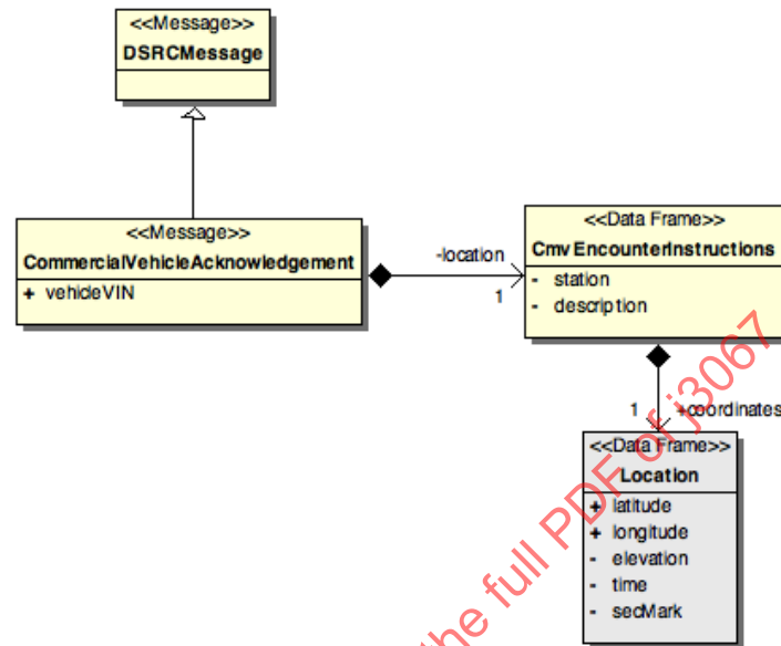
FIGURE 30 - DATA MODEL - commercialVehicleAcknowledgement
