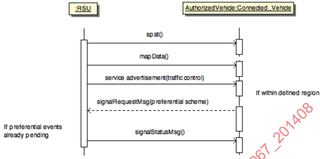
FIGURE 8 - REQUEST SIGNAL PREFERENTIAL TREATMENT DIALOG
