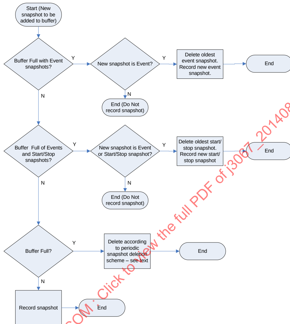
FIGURE 21 - CONNECTED VEHICLE - BUFFER OVERFLOW STATE - DELETING SNAPSHOTS
