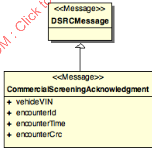
FIGURE 27 - DATA MODEL - commercialScreeningAcknowledgement
