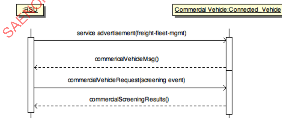
FIGURE 11 - EXCHANGE PREVIOUS COMMERCIAL VEHICLE SCREENING RESULTS DIALOG
