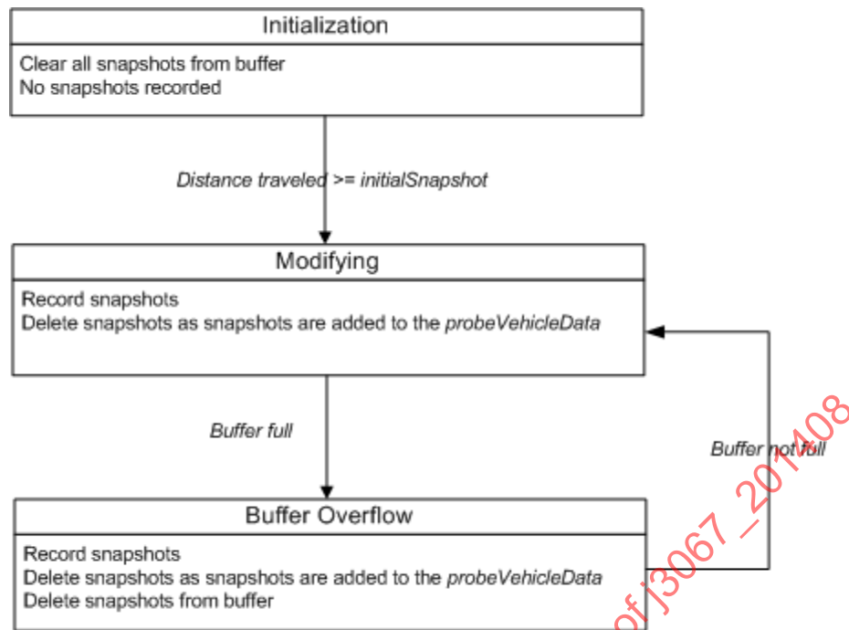
FIGURE 18 - CONNECTED VEHICLE - SNAPSHOT STATES
