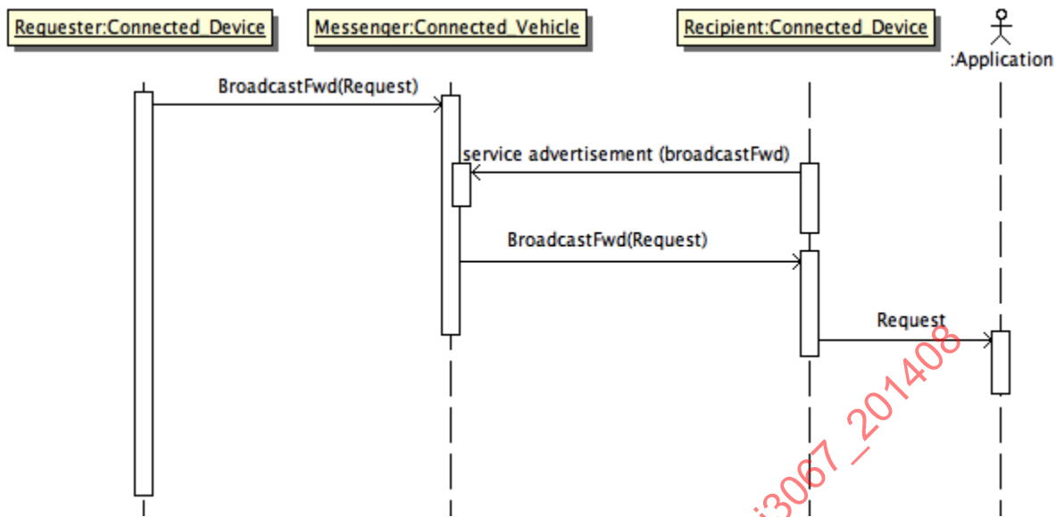
FIGURE 6 - FORWARD MAYDAY DIALOG
