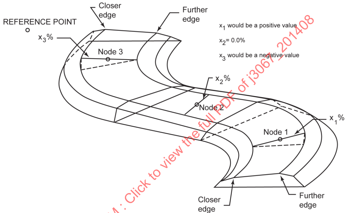
FIGURE 3 - SUPERELEVATION
