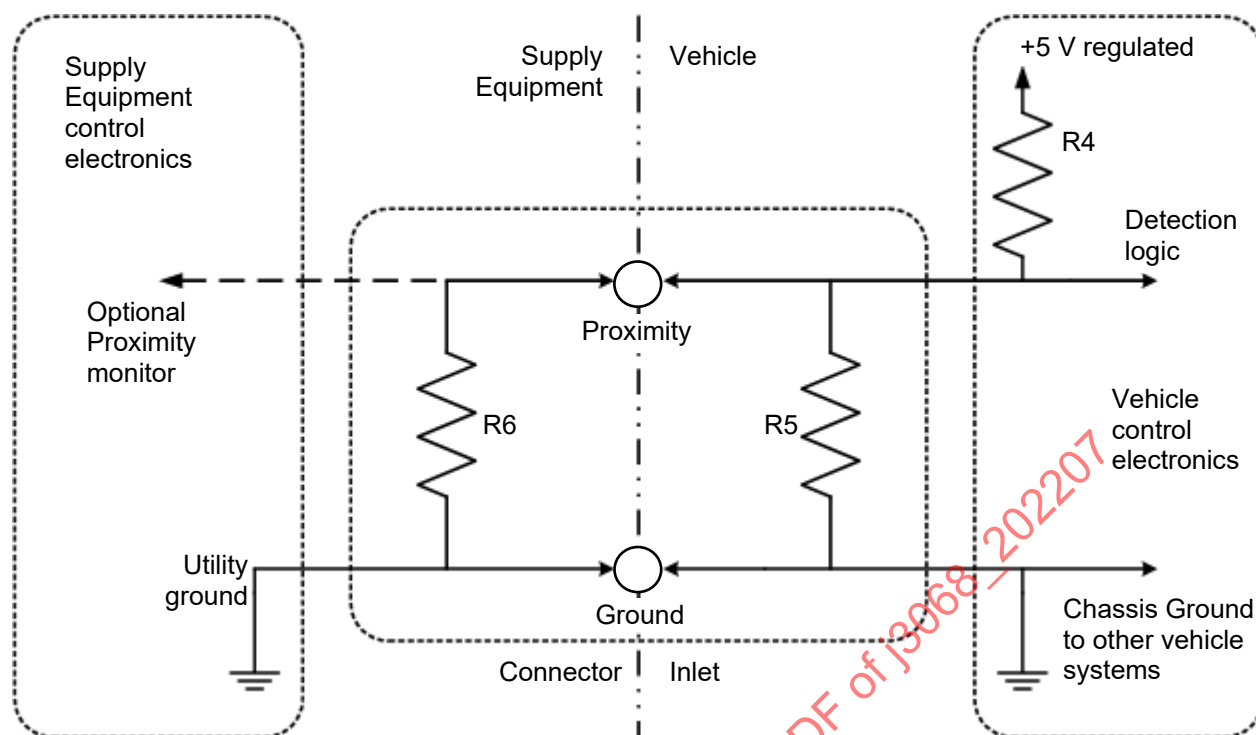
Figure 12 - Equivalent proximity circuit diagram for SAE J3068 coupler
