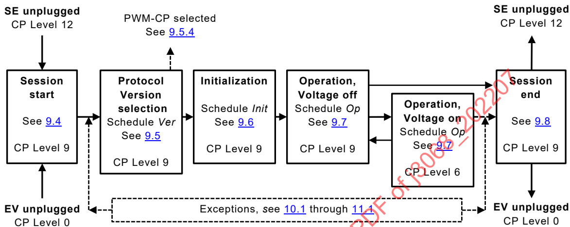
Figure 14 - Overview of typical application program control sequence during a connection session
