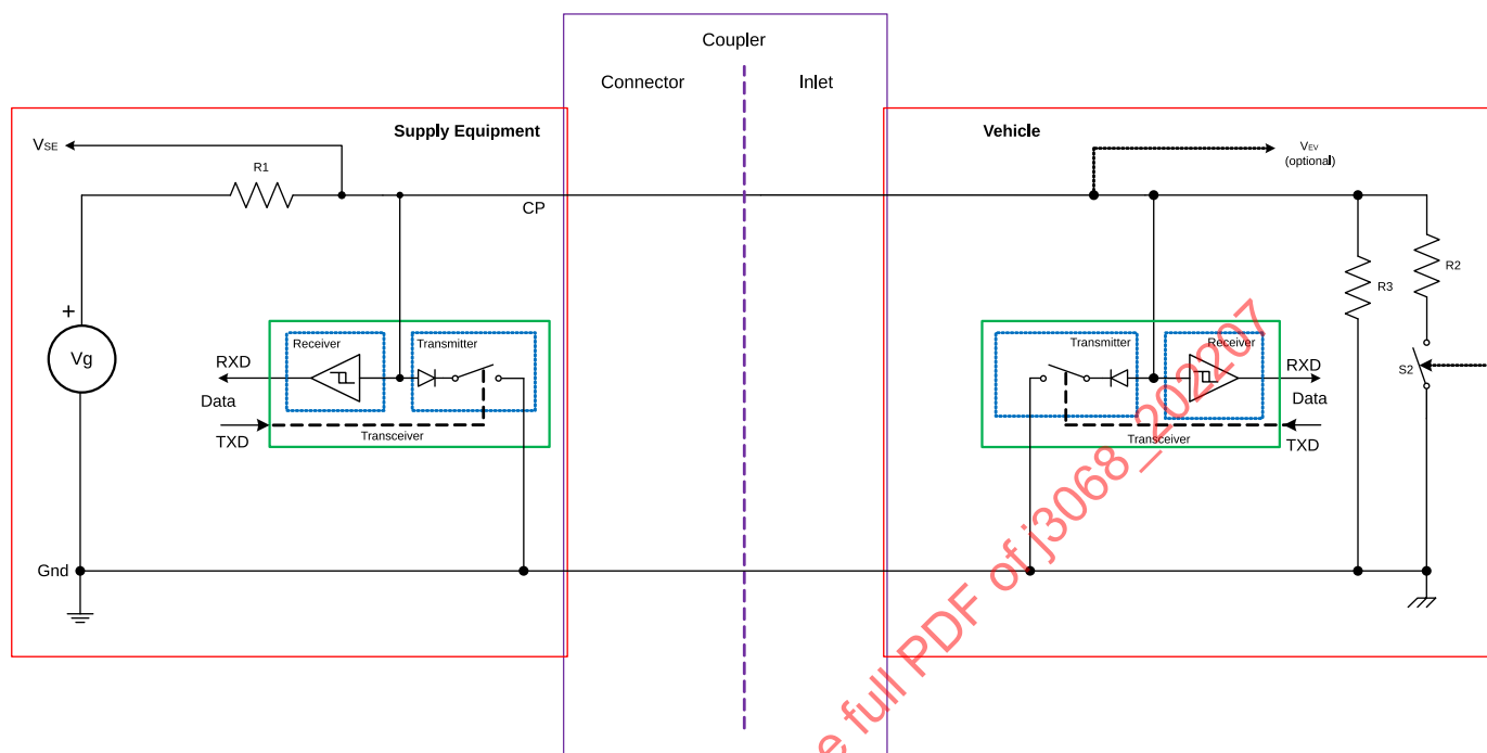
Figure 11A - Configuration without PWM-CP compatibility
