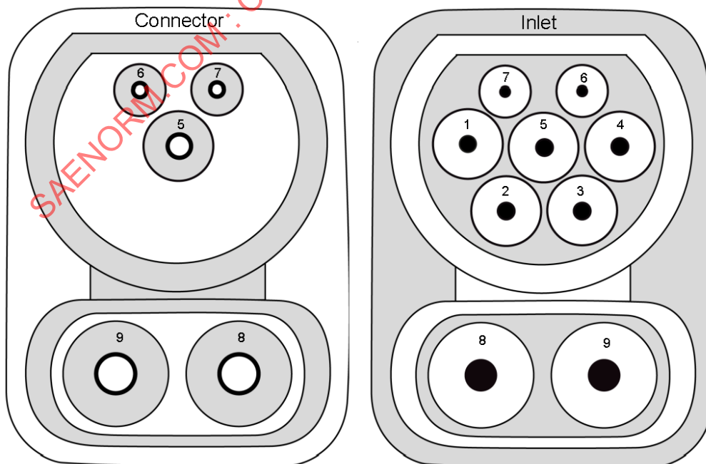
Figure 7 - Typical SAE J3068 AC 6 connector and inlet photos (contact placement as seen by user)
