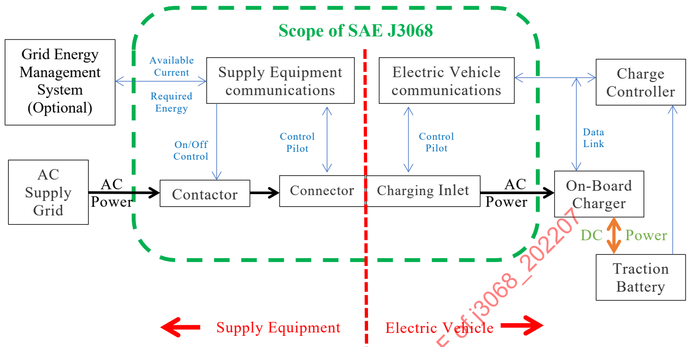
Figure 4 - General conductive charging system topology for typical case C
