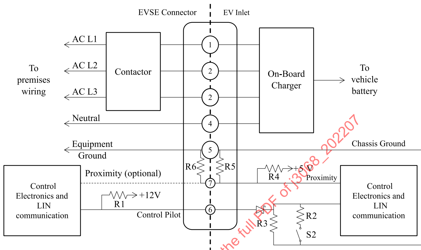
Figure 6 - Electrical system block diagram for three-phase supply (SE that supports LIN-CP only with EV that supports LIN-CP and PWM-CP shown)
