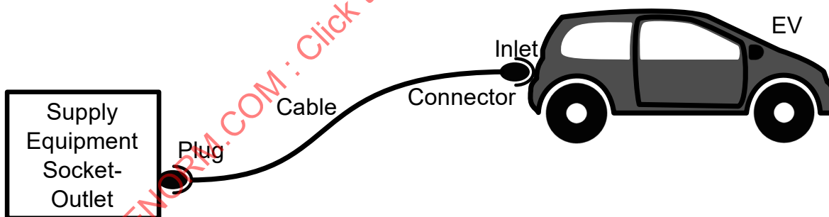
Figure 2 - Case B: Fully removable charging cord
