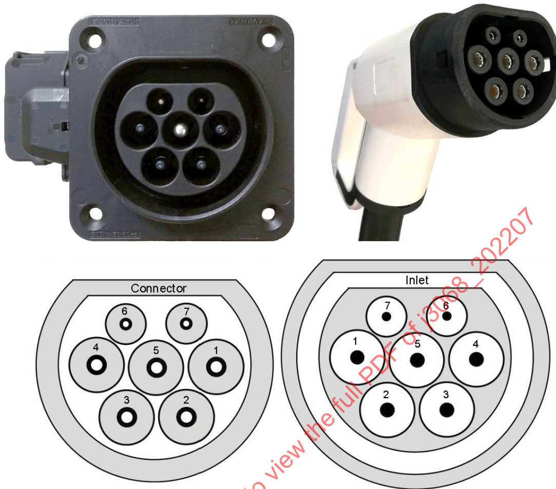
Figure 7 - Typical SAE J3068 AC 6 connector and inlet photos (contact placement as seen by user)
