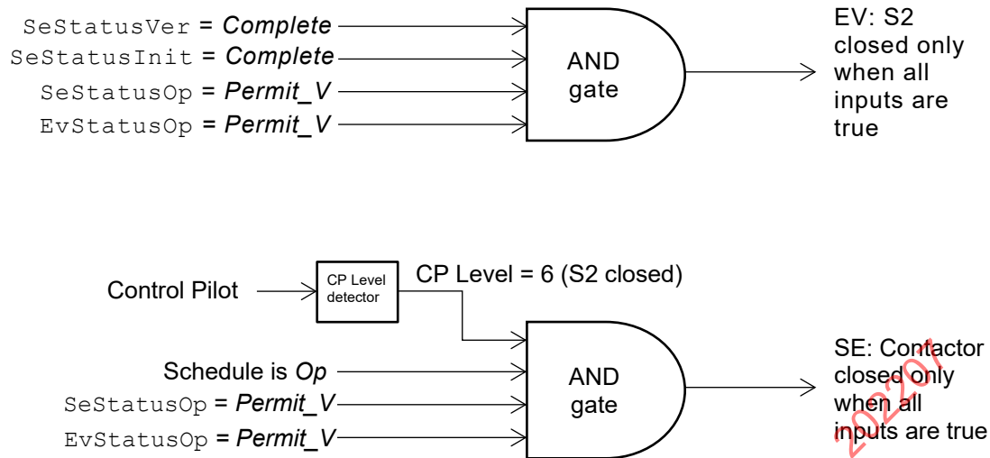
Figure 15 - Control logic concepts for S2 and contactor, informative
