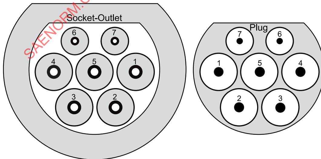
Figure B2 - SAE universal AC socket-outlet (left) and plug of the EV cable assembly (right)
