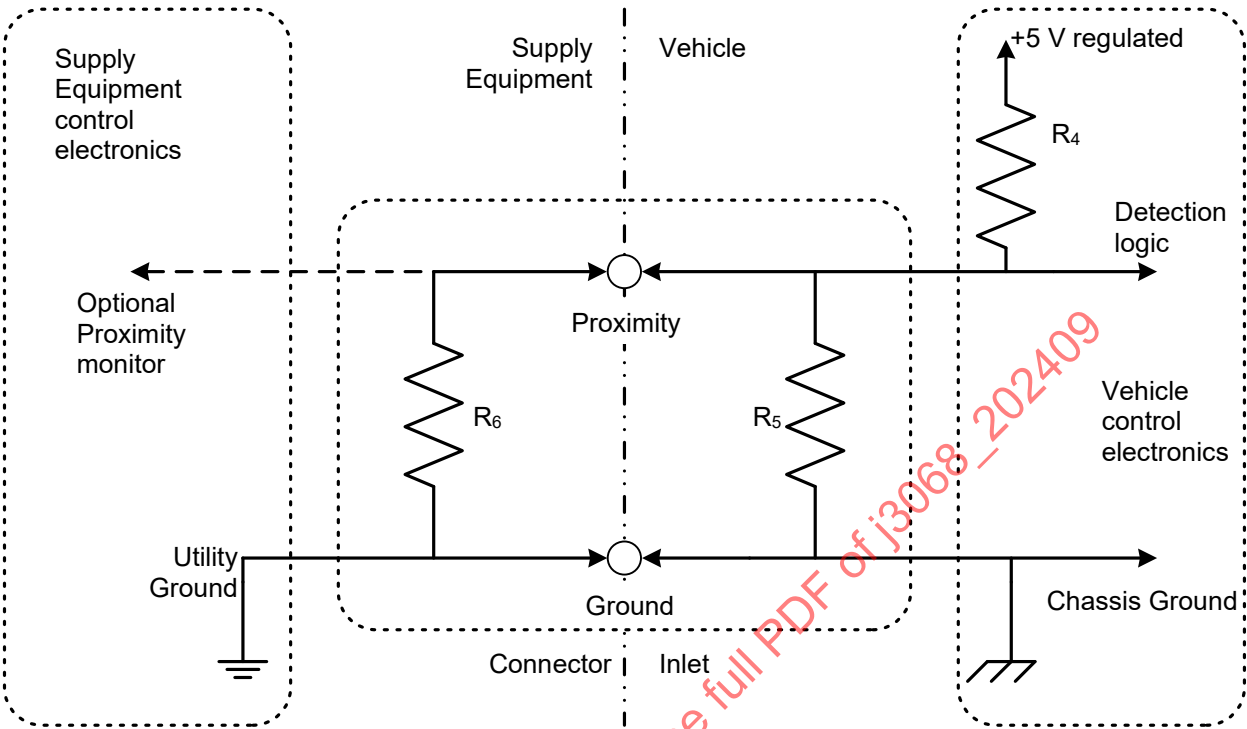
Figure 12 - Equivalent proximity circuit diagram for SAE J3068 coupler under case C
