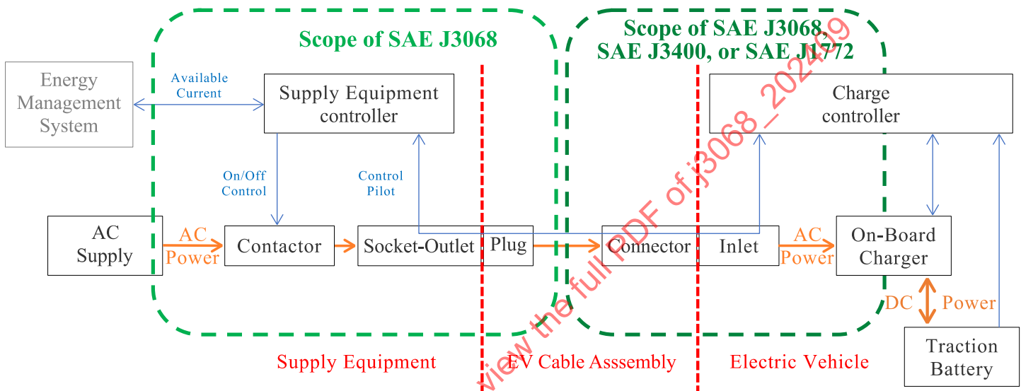
Figure B1 - General AC conductive charging system topology for case B
