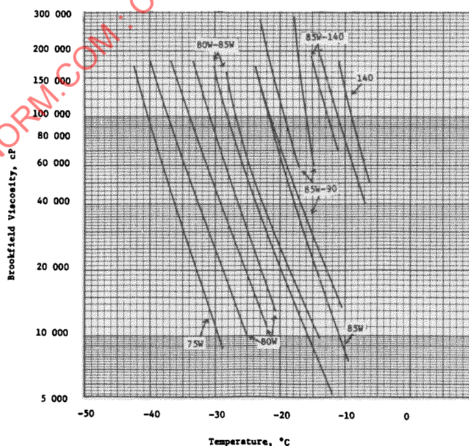
FIGURE 1 - Brookfield Viscosity Versus Temperature for Typical Gear Lubricants (SAE Viscosity Grades Indicated)
