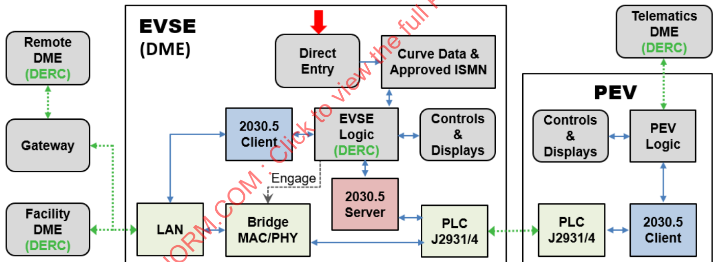
Figure C1 - EVSE as IEEE 2030.5 server for SAE J3072 communications
