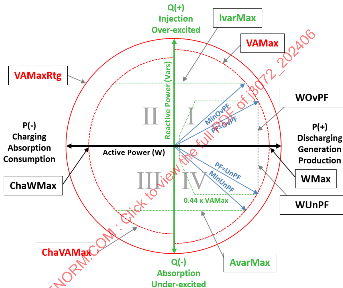
Figure B1 - Power vector quadrant diagram
