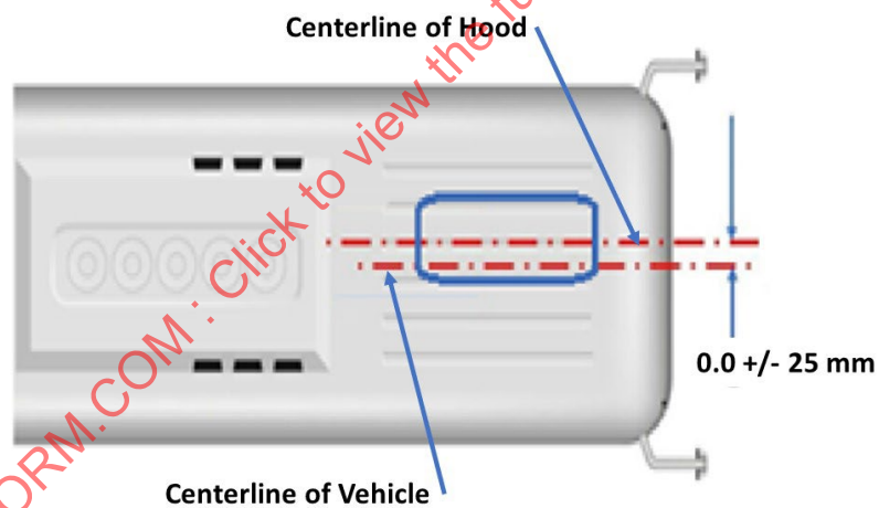
Figure 5 - Hood location above the vehicle
