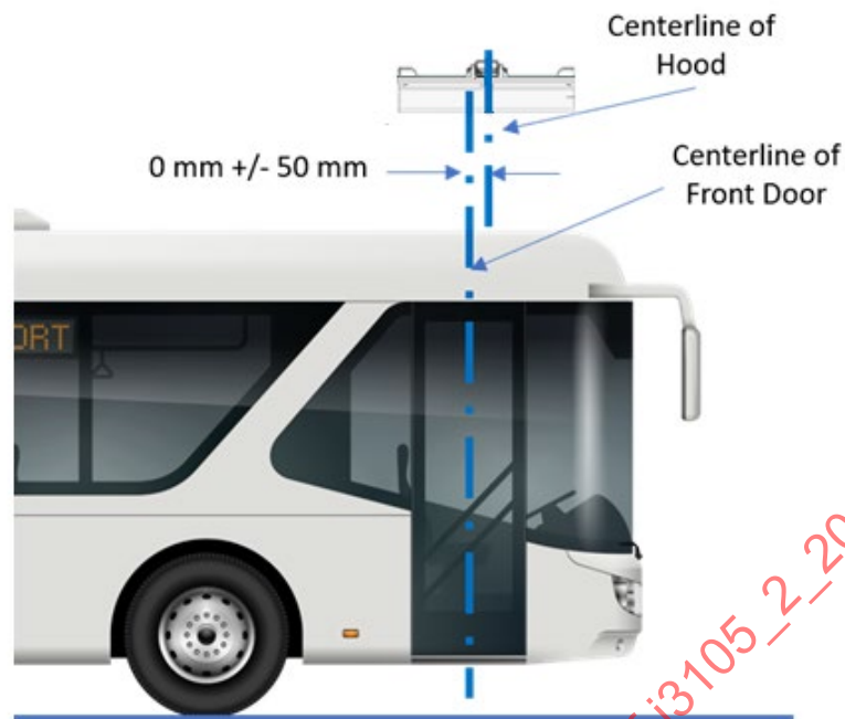
Figure 4 - Lateral hood location
