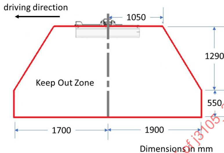
Figure 6 - Lateral keep-out zone dimensions under hood
