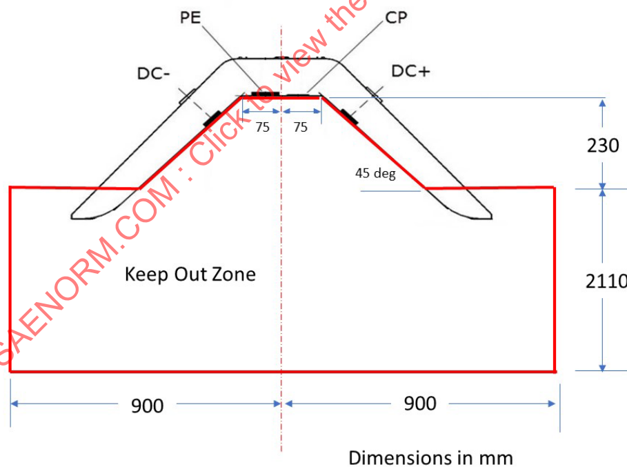
Figure 7 - Fore and aft keep-out zone dimensions (front view)
